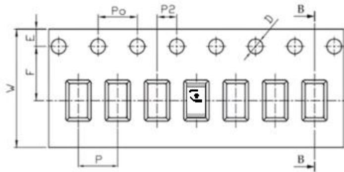
b. Tape Dimensions (unit: mm)
