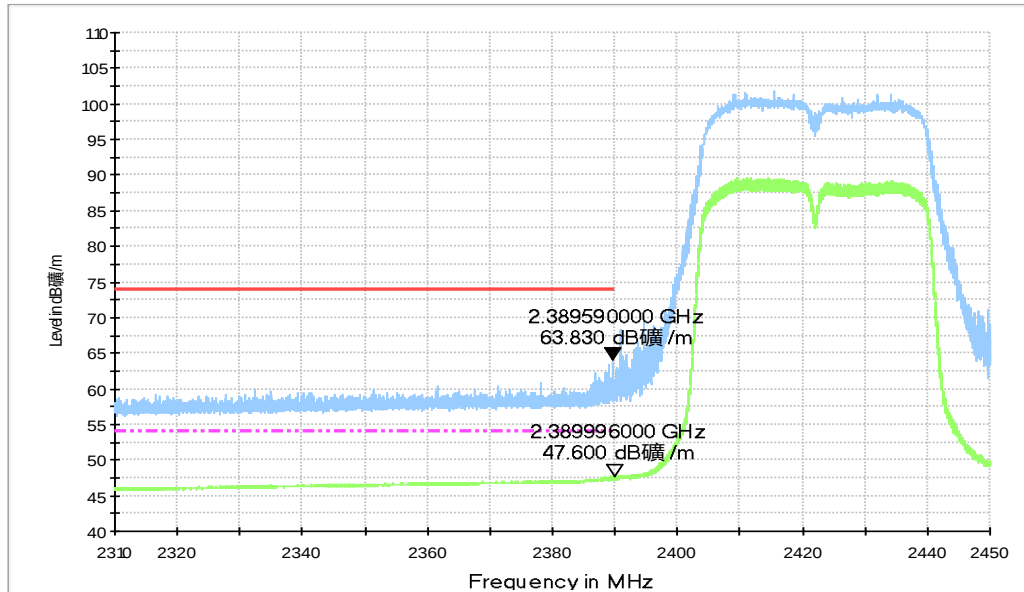
RE - Power-2.31GHz-2.45GHz
