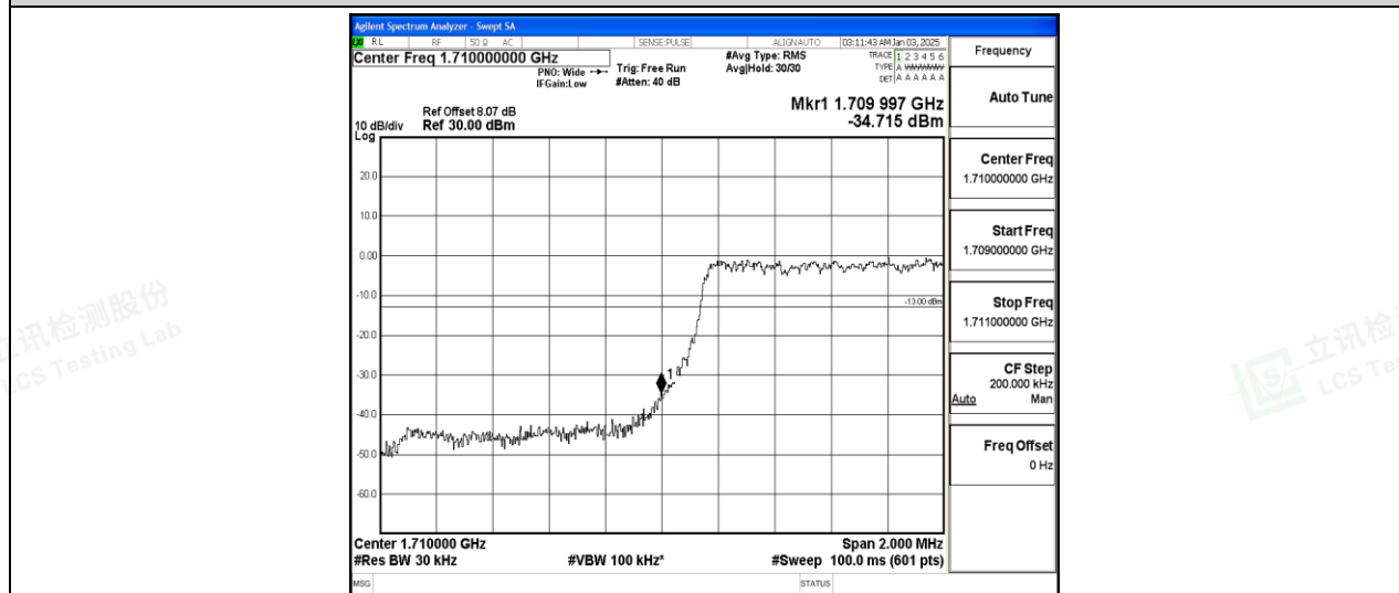
Band66-1.4MHz-16QAM-131979-6-0-Low--34.71-PASS
