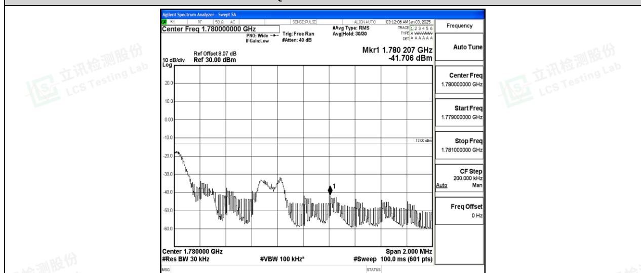
Band66-1.4MHz-16QAM-132665-1-0-High--41.71-PASS
