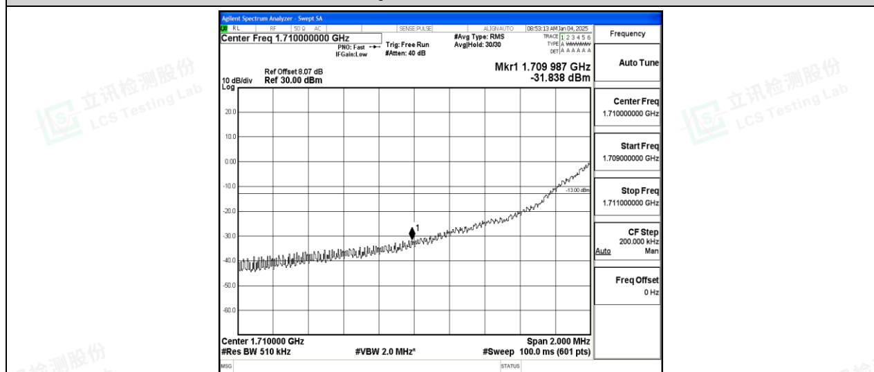
Band66-20MHz-16QAM-132072-6-0-Low--31.84-PASS
