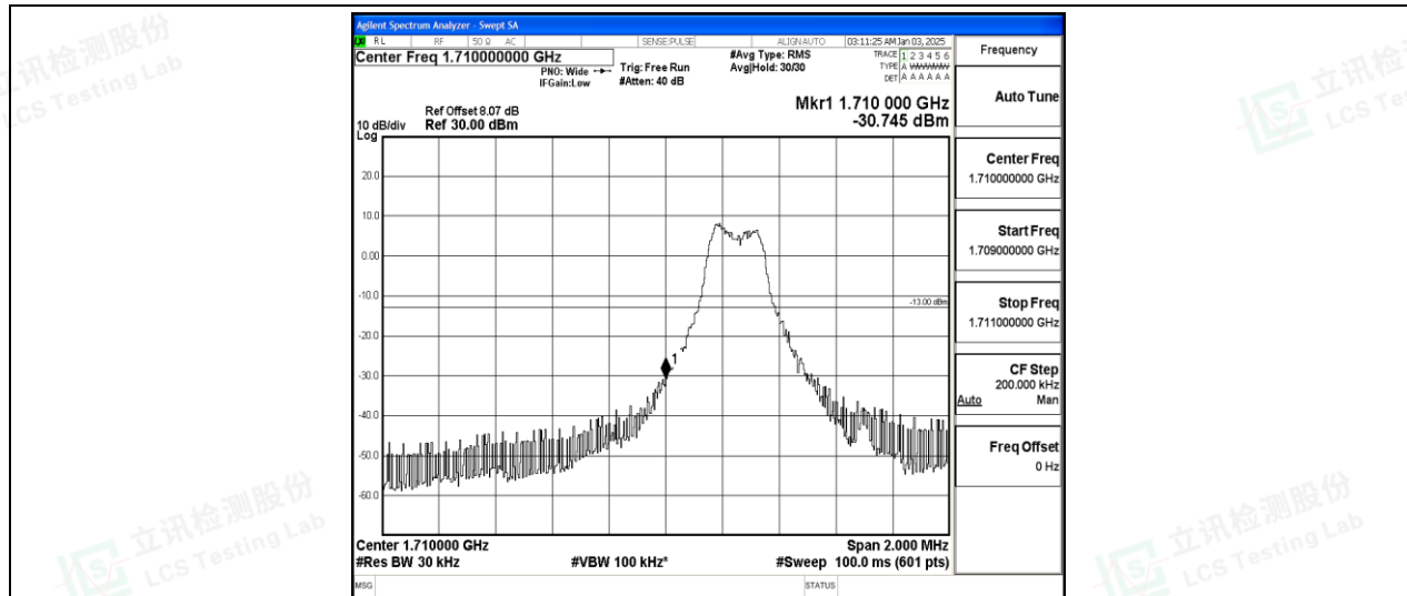
Band66-1.4MHz-16QAM-131979-1-0-Low--30.75-PASS
