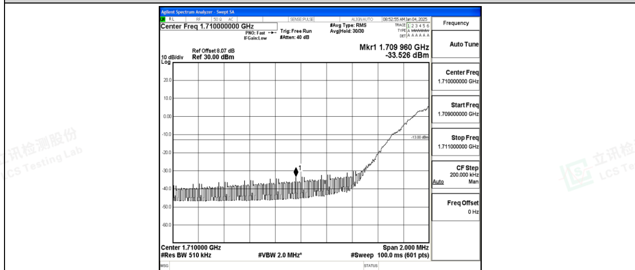
Band66-20MHz-16QAM-132072-1-0-Low--33.53-PASS
