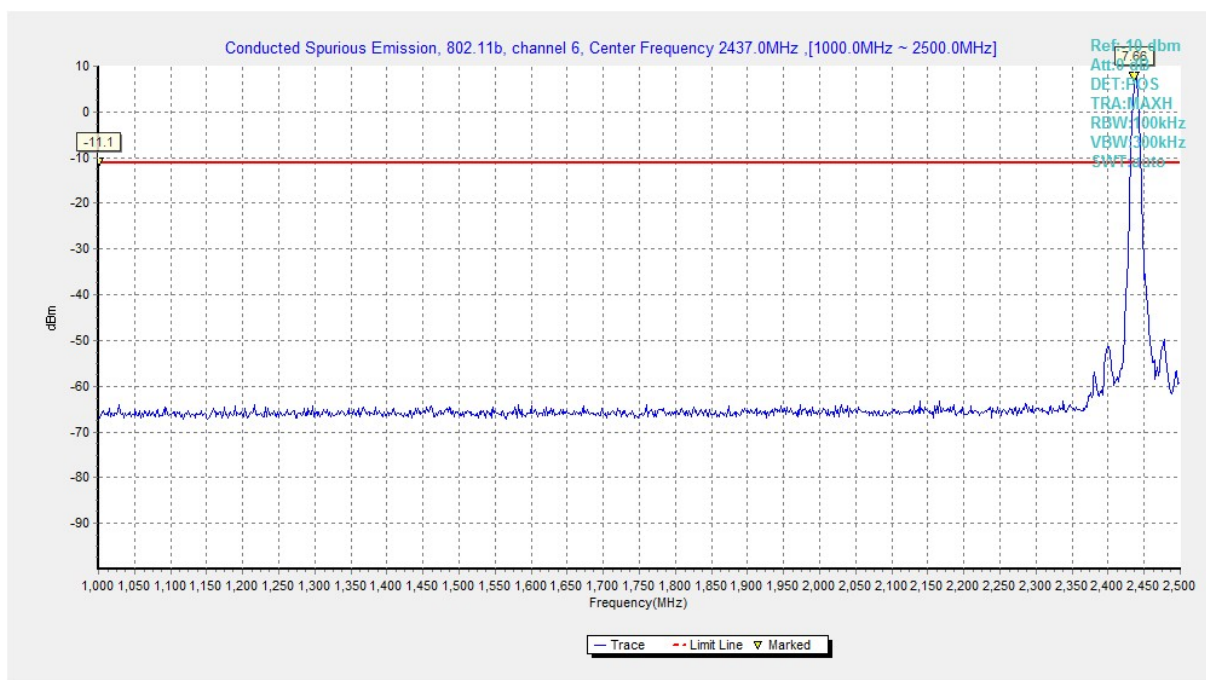
Fig.A.6.1.11 Conducted Spurious Emission (802.11b, Ch6, 1 GHz-2.5 GHz)
