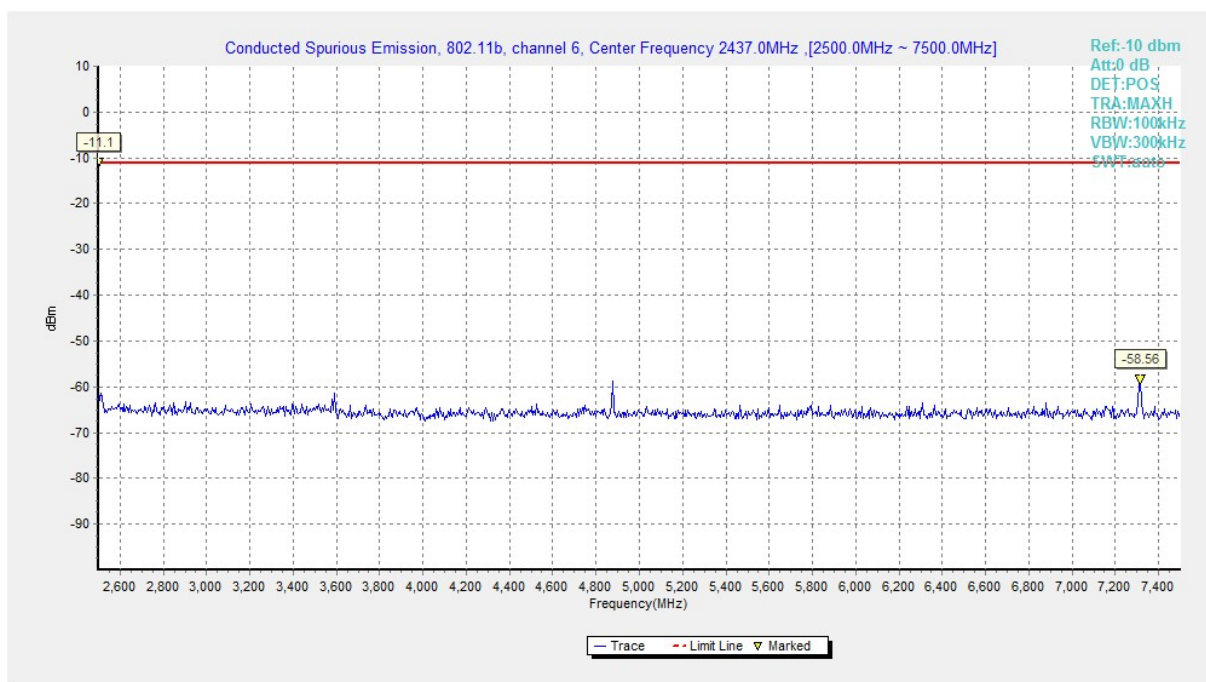
Fig.A.6.1.12 Conducted Spurious Emission (802.11b, Ch6, 2.5 GHz-7.5 GHz)
