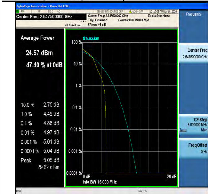
Band41(2535-2655)-15MHz-16QAM-41165-1RB#0-PASS
