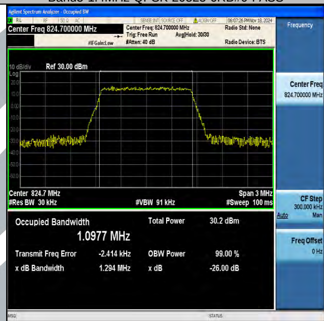
Band5-1.4MHz-16QAM-20407-6RB#0-PASS
