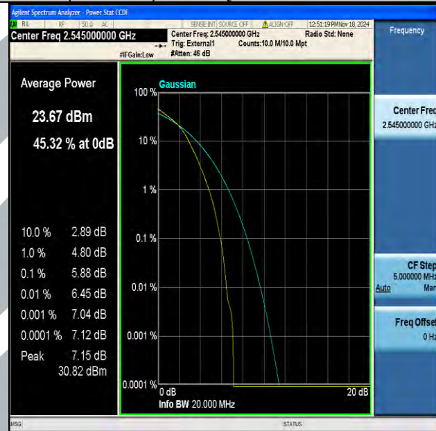
Band41(2535-2655)-20MHz-16QAM-40140-100RB#0-PASS
