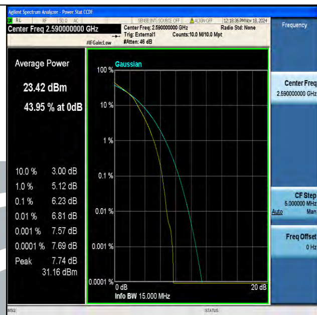
Band41(2535-2655)-15MHz-16QAM-40590-75RB#0-PASS
