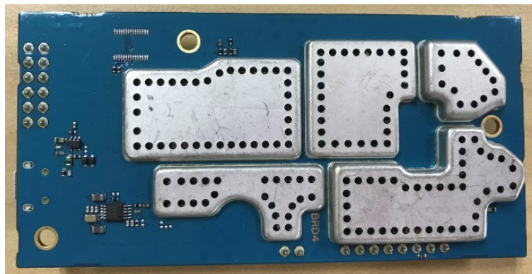
DLR Modem Board Side 2 (With Shield)
