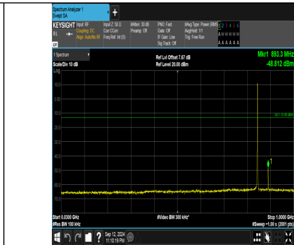
Band5_1.4MHz_16QAM_20643_6RB#0_30~1000_30~1000
