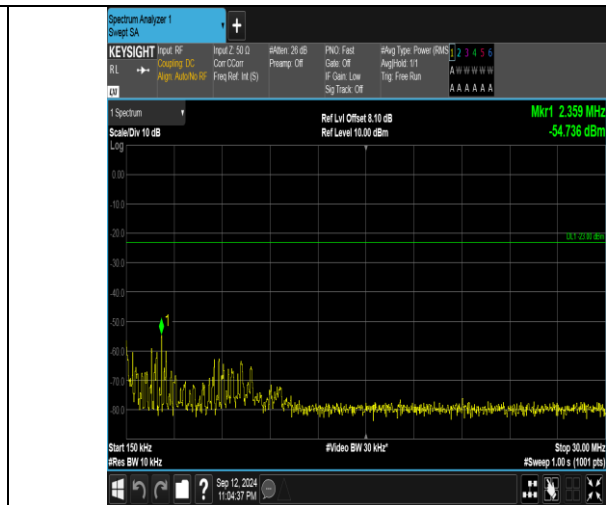
Band5_1.4MHz_QPSK_20525_6RB#0_0.15~30_0.15~30
