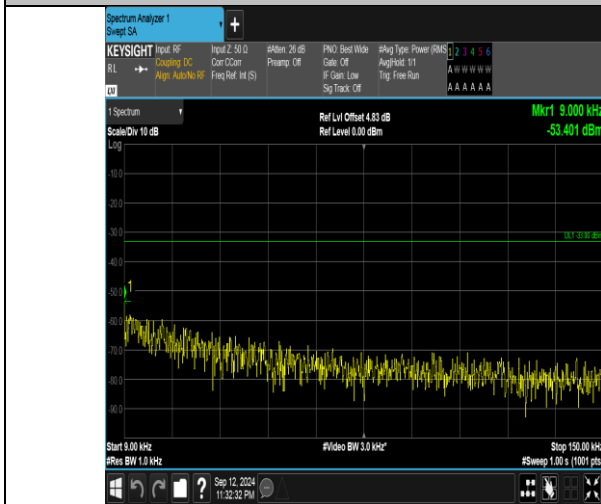
Band5_3MHz_QPSK_20525_1RB#14_0.009~0.15_0.009~0.15
