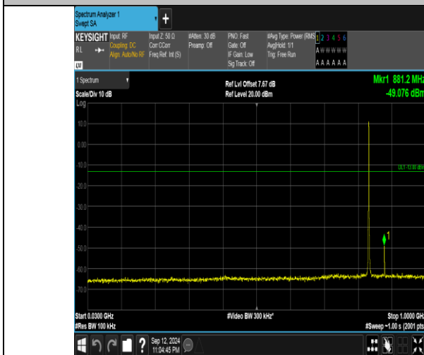
Band5_1.4MHz_QPSK_20525_6RB#0_30~1000_30~1000
