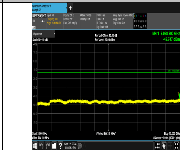
Band5_1.4MHz_16QAM_20525_6RB#0_3000~10000_3000~10000
