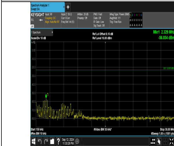
Band5_3MHz_16QAM_20525_1RB#14_0.15~30_0.15~30
