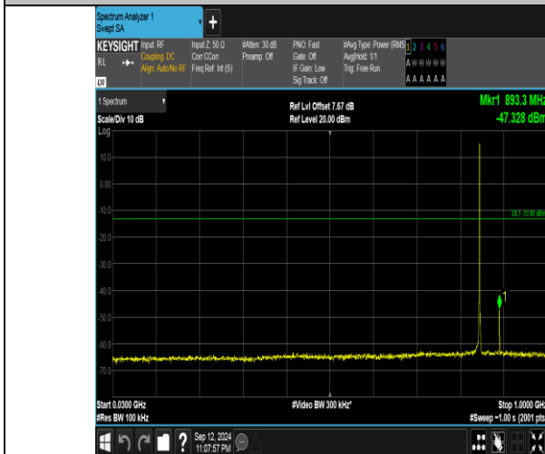
Band5_1.4MHz_QPSK_20643_1RB#5_30~1000_30~1000
