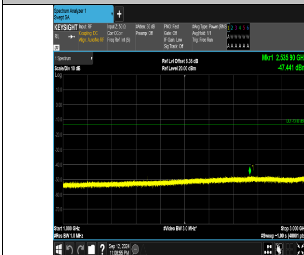
Band5_1.4MHz_16QAM_20643_1RB#5_1000~3000_1000~3000
