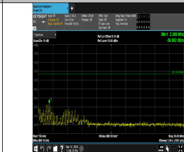
Band5_1.4MHz_QPSK_20643_1RB#0_0.15~30_0.15~30
