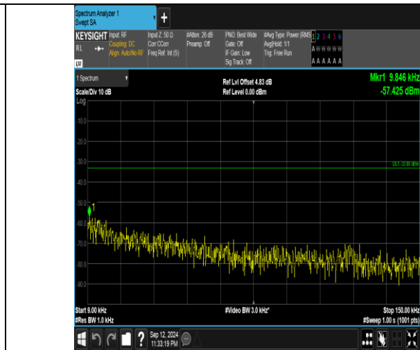
Band5_3MHz_16QAM_20525_1RB#14_0.009~0.15_0.009~0.15
