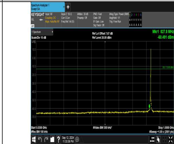
Band5_3MHz_16QAM_20525_1RB#14_30~1000_30~1000
