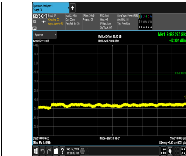
Band5_3MHz_QPSK_20525_1RB#14_3000~10000_3000~10000
