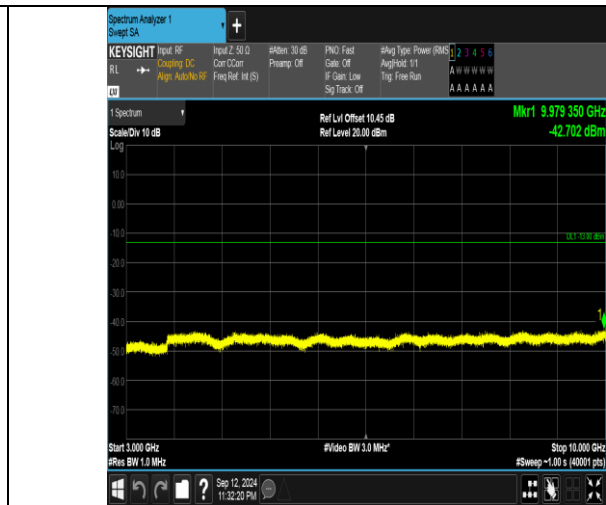
Band5_3MHz_16QAM_20525_1RB#0_3000~10000_3000~10000
