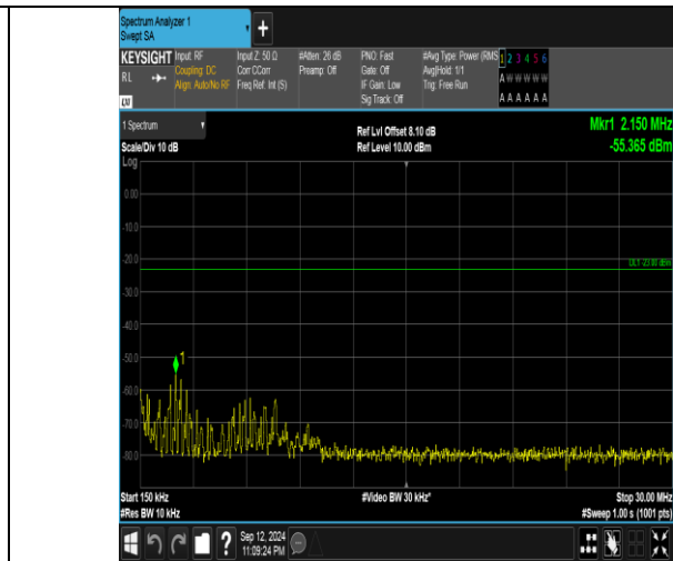
Band5_1.4MHz_QPSK_20643_6RB#0_0.15~30_0.15~30
