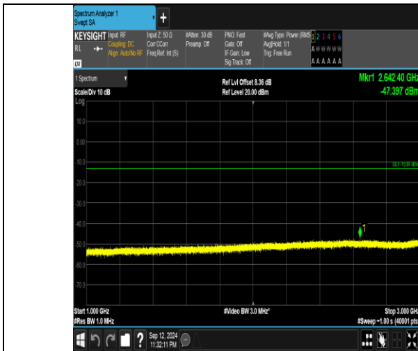
Band5_3MHz_16QAM_20525_1RB#0_1000~3000_1000~3000
