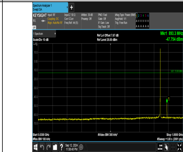
Band5_1.4MHz_16QAM_20643_1RB#5_30~1000_30~1000
