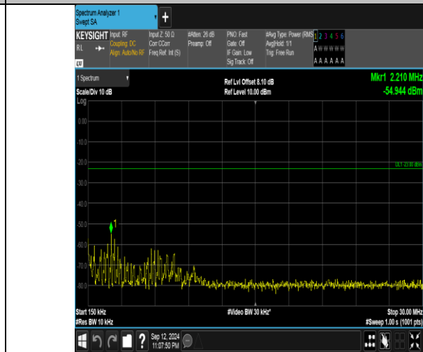
Band5_1.4MHz_QPSK_20643_1RB#5_0.15~30_0.15~30
