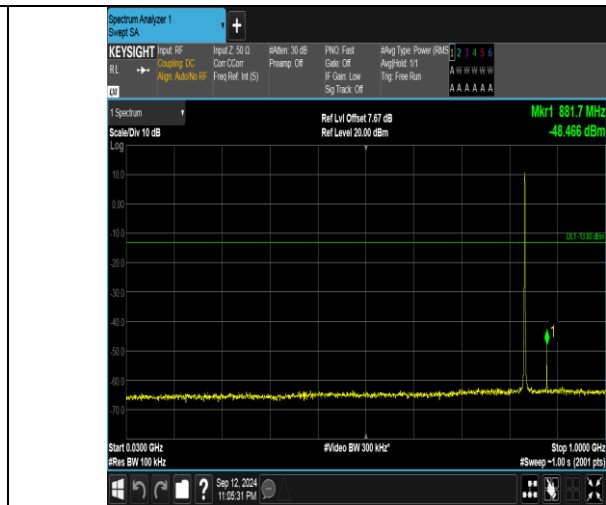
Band5_1.4MHz_16QAM_20525_6RB#0_30~1000_30~1000
