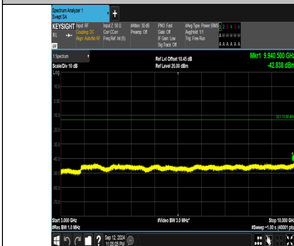
Band5_1.4MHz_QPSK_20525_6RB#0_3000~10000_3000~10000
