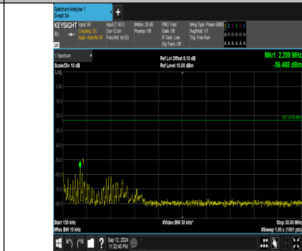
Band5_3MHz_QPSK_20525_1RB#14_0.15~30_0.15~30
