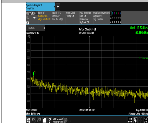
Band5_1.4MHz_QPSK_20643_1RB#0_0.009~0.15_0.009~0.15
