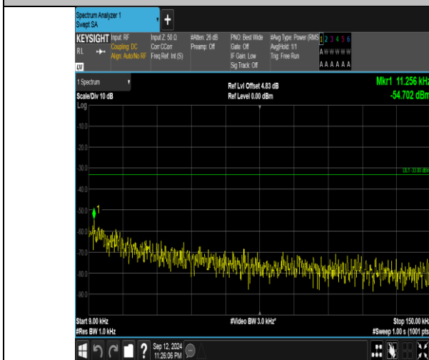
Band5_3MHz_QPSK_20415_1RB#0_0.009~0.15_0.009~0.15
