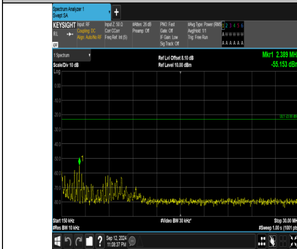
Band5_1.4MHz_16QAM_20643_1RB#5_0.15~30_0.15~30
