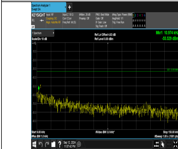
Band5_1.4MHz_QPSK_20643_1RB#5_0.009~0.15_0.009~0.15
