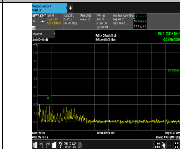
Band5_3MHz_QPSK_20415_1RB#0_0.15~30_0.15~30
