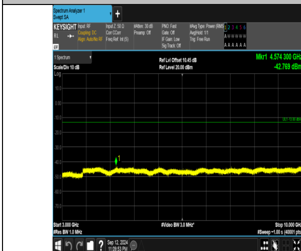
Band5_1.4MHz_QPSK_20643_6RB#0_3000~10000_3000~10000
