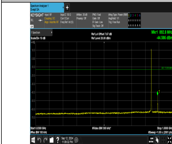
Band5_1.4MHz_QPSK_20643_6RB#0_30~1000_30~1000
