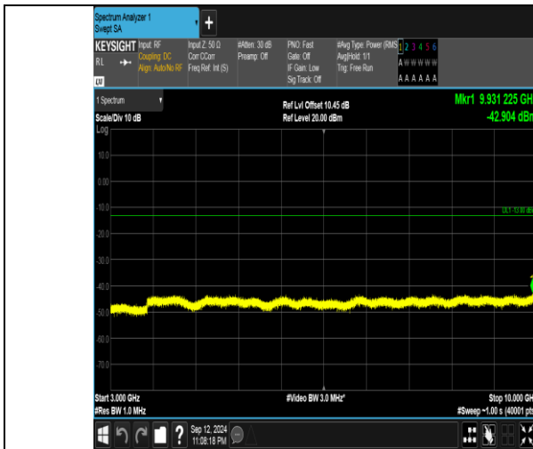
Band5_1.4MHz_QPSK_20643_1RB#5_3000~10000_3000~10000
