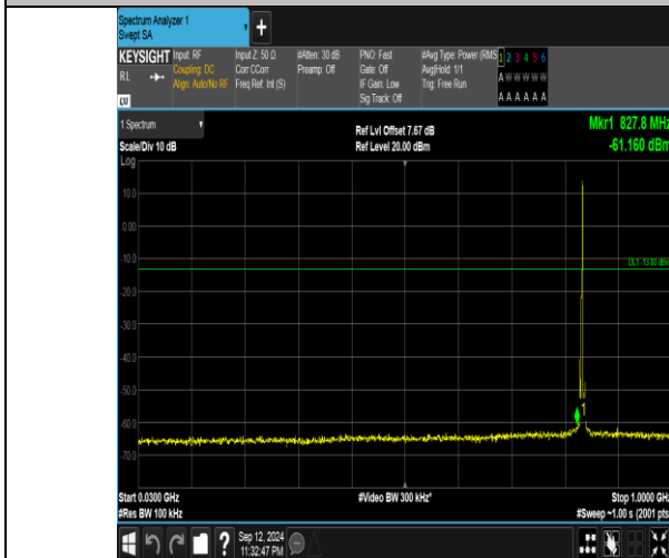
Band5_3MHz_QPSK_20525_1RB#14_30~1000_30~1000
