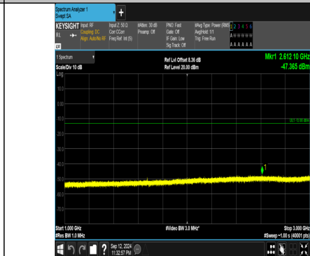
Band5_3MHz_QPSK_20525_1RB#14_1000~3000_1000~3000
