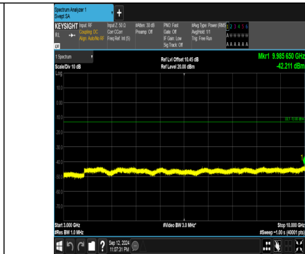
Band5_1.4MHz_16QAM_20643_1RB#0_3000~10000_3000~10000
