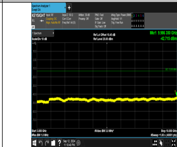
Band5_1.4MHz_16QAM_20643_6RB#0_3000~10000_3000~10000
