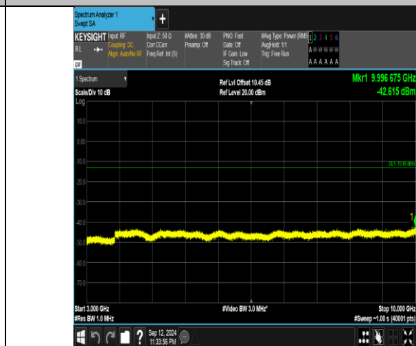
Band5_3MHz_16QAM_20525_1RB#14_3000~10000_3000~10000
