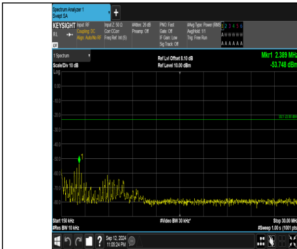
Band5_1.4MHz_16QAM_20525_6RB#0_0.15~30_0.15~30
