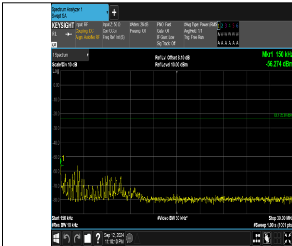
Band5_1.4MHz_16QAM_20643_6RB#0_0.15~30_0.15~30
