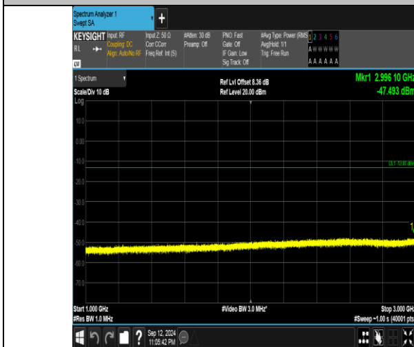
Band5_1.4MHz_16QAM_20525_6RB#0_1000~3000_1000~3000
