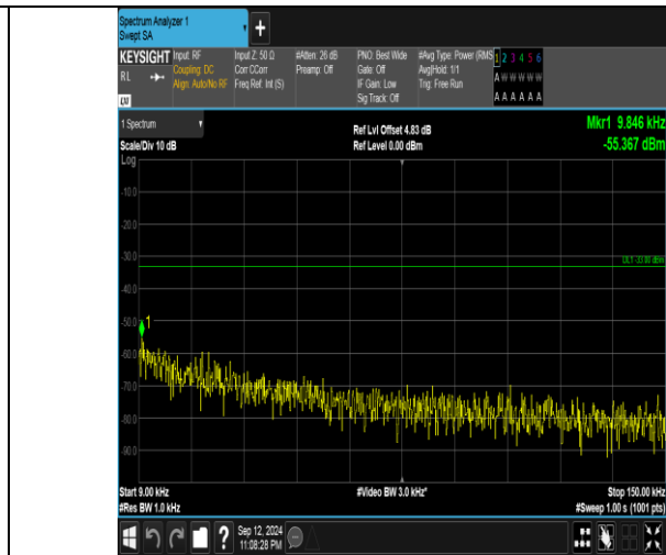
Band5_1.4MHz_16QAM_20643_1RB#5_0.009~0.15_0.009~0.15
