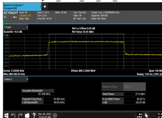
B4_N41(70M)_CP-OFDM_16 QAM_Outer_Full_Mid_CH
