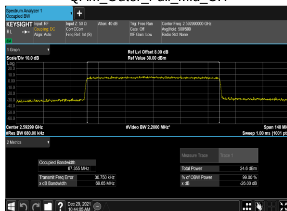
B4_N41(70M)_CP-OFDM_256 QAM_Outer_Full_Mid_CH
