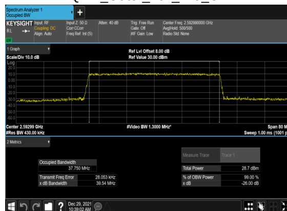
B4_N41(40M)_CP-OFDM_16 QAM_Outer_Full_Mid_CH
