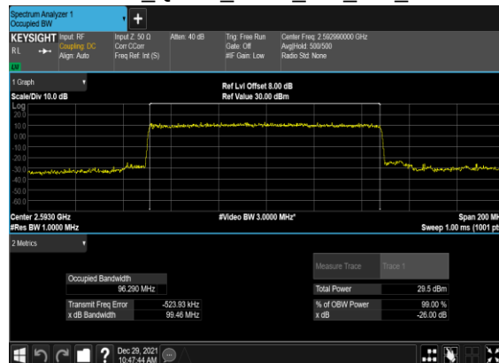
B4_N41(100M)_DFT-s- OFDM_QPSK_Outer_Full_Mid_CH
