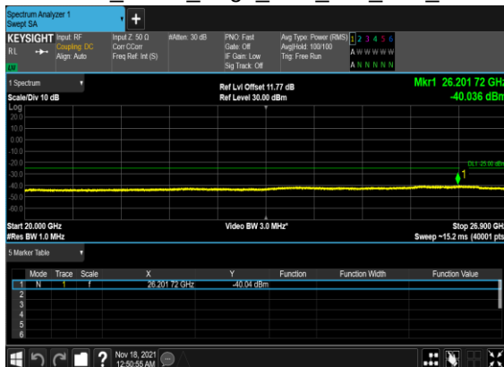
B4_N41(100M)_DFT-s- OFDM_BPSK_Edge_1RB_Left_Low_CH
