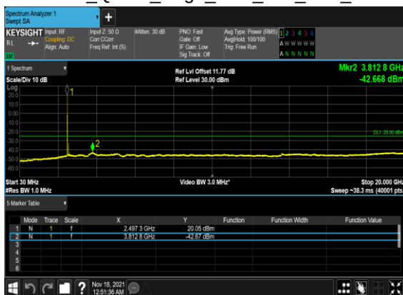
B4_N41(100M)_DFT-s- OFDM_QPSK_Edge_1RB_Left_Low_CH
