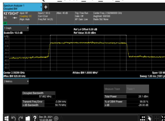
B4_N41(60M)_CP-OFDM_16 QAM_Outer_Full_Mid_CH
