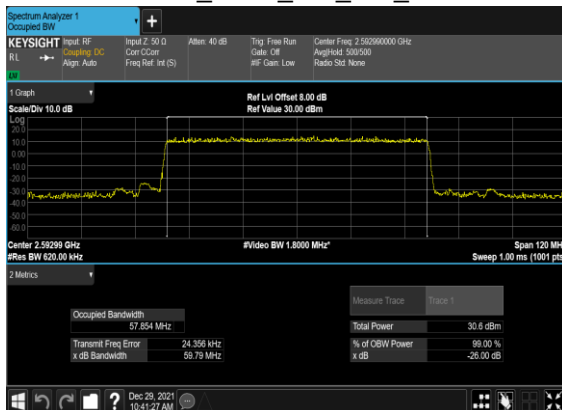
B4_N41(60M)_DFT-s-OFDM_PI_2- BPSK_Outer_Full_Mid_CH
