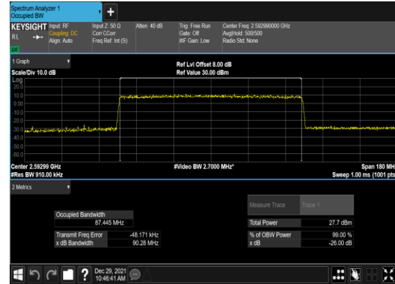
B4_N41(90M)_CP-OFDM_16 QAM_Outer_Full_Mid_CH
