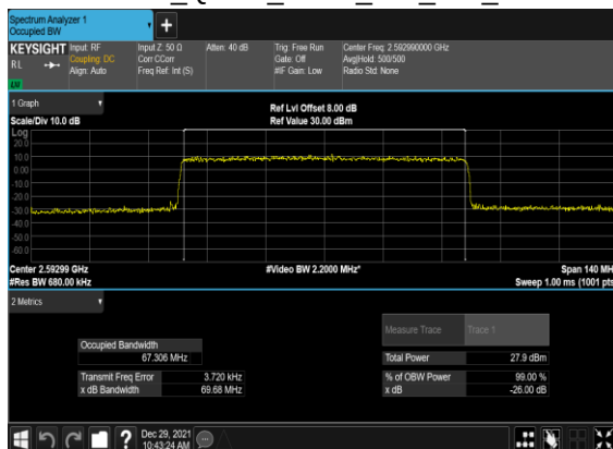
B4_N41(70M)_CP- OFDM_QPSK_Outer_Full_Mid_CH
