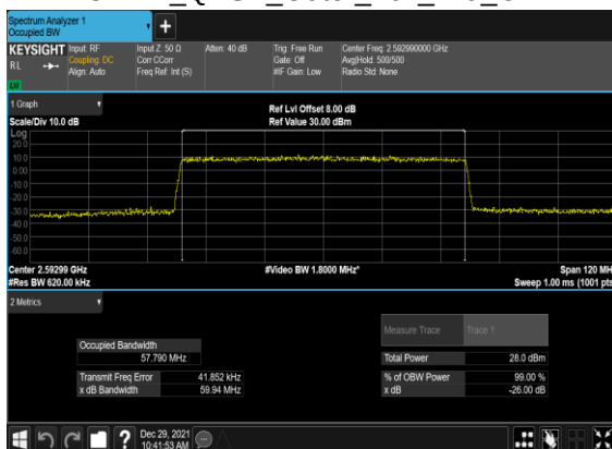
B4_N41(60M)_CP- OFDM_QPSK_Outer_Full_Mid_CH
