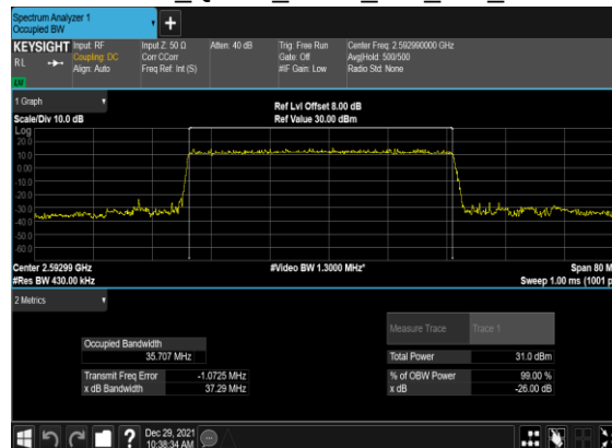
B4_N41(40M)_DFT-s- OFDM_QPSK_Outer_Full_Mid_CH
