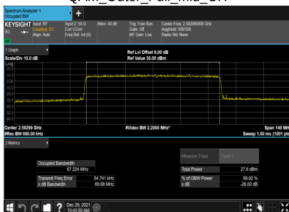
B4_N41(70M)_CP-OFDM_64 QAM_Outer_Full_Mid_CH
