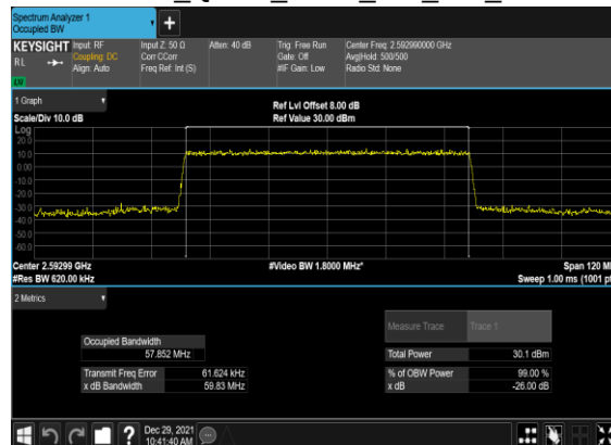
B4_N41(60M)_DFT-s- OFDM_QPSK_Outer_Full_Mid_CH
