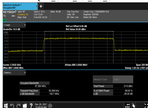
B4_N41(100M)_CP-OFDM_16 QAM_Outer_Full_Mid_CH
