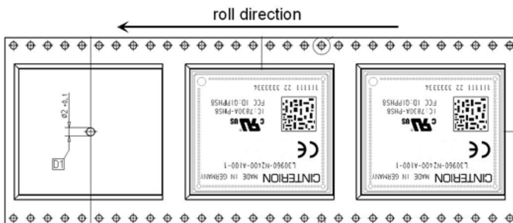
Figure 38: Reel direction
