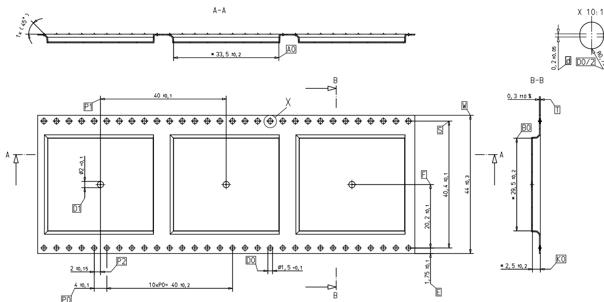
Figure 37: Carrier tape
