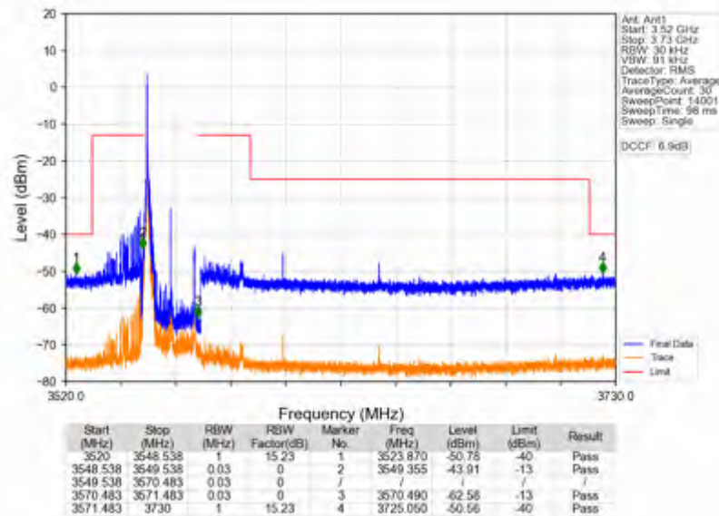
n78d_30kHz_SISO_NTNV_20MHz_DFT-s-OFDM PI/2 BPSK_3560.01MHz_Edge_1RB_Left
