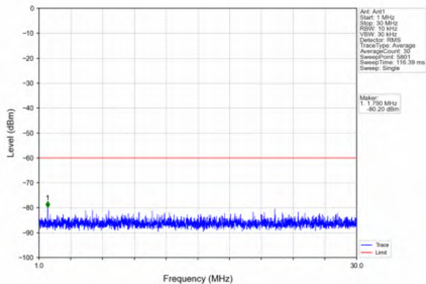
n78d_30kHz_SISO_NTNV_15MHz_DFT-s-OFDM_QPSK_3692.49MHz_Edge_1RB_Right
