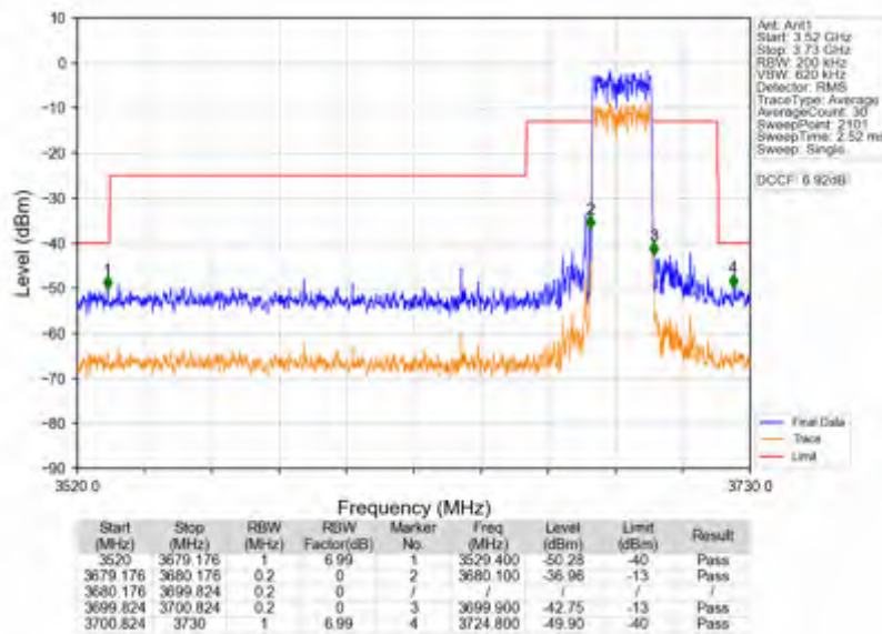
n78d_30kHz_SISO_NTNV_20MHz_CP-OFDM QPSK_3690MHz_Outer_Full
