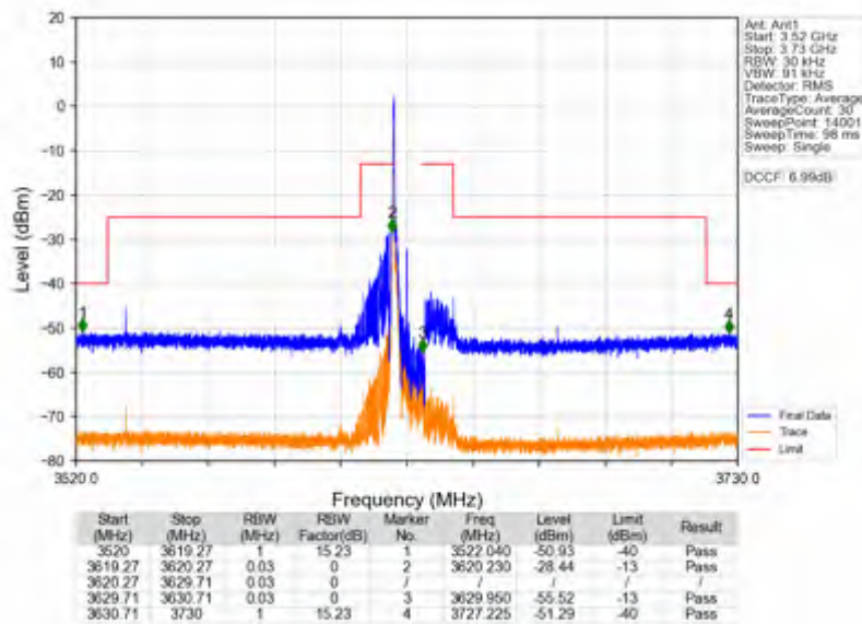
n78d_30kHz_SISO_NTNV_10MHz_DFT-s-OFDM PI/2 BPSK_3624.99MHz_Edge_1RB_Left
