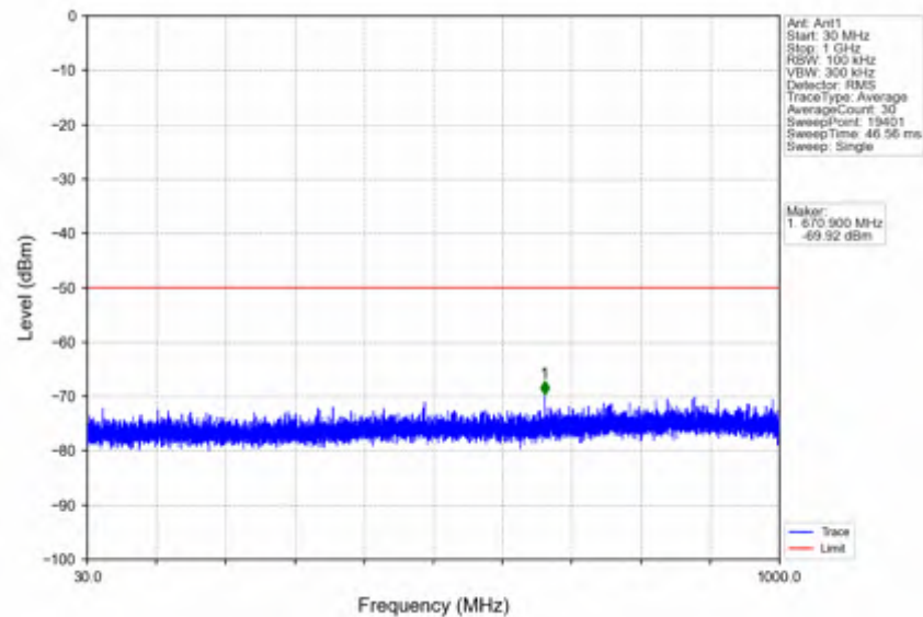
n78d_15kHz_SISO_NTNV_50MHz_CP-OFDM_QPSK_3675MHz_Inner_1RB_Right
