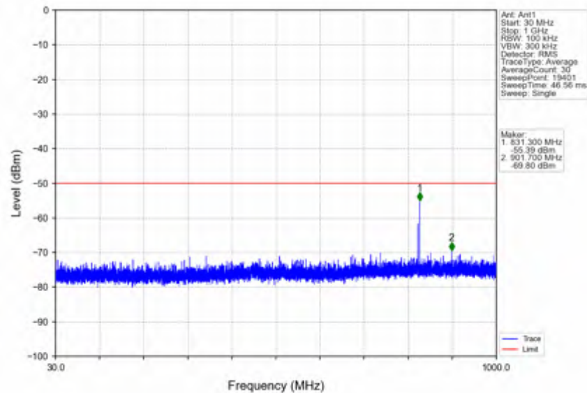
n78d_30kHz_SISO_NTNV_15MHz_CP-OFDM QPSK_3692.49MHz_Edge_1RB_Right
