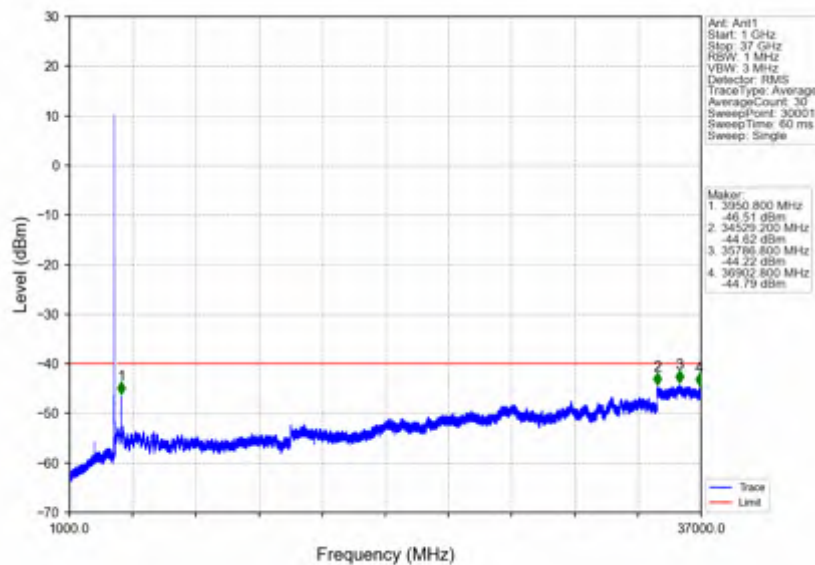
n78d_30kHz_SISO_NTNV_10MHz_DFT-s-OFDM_PI/2_BPSK_3555MHz_Outer_Full
