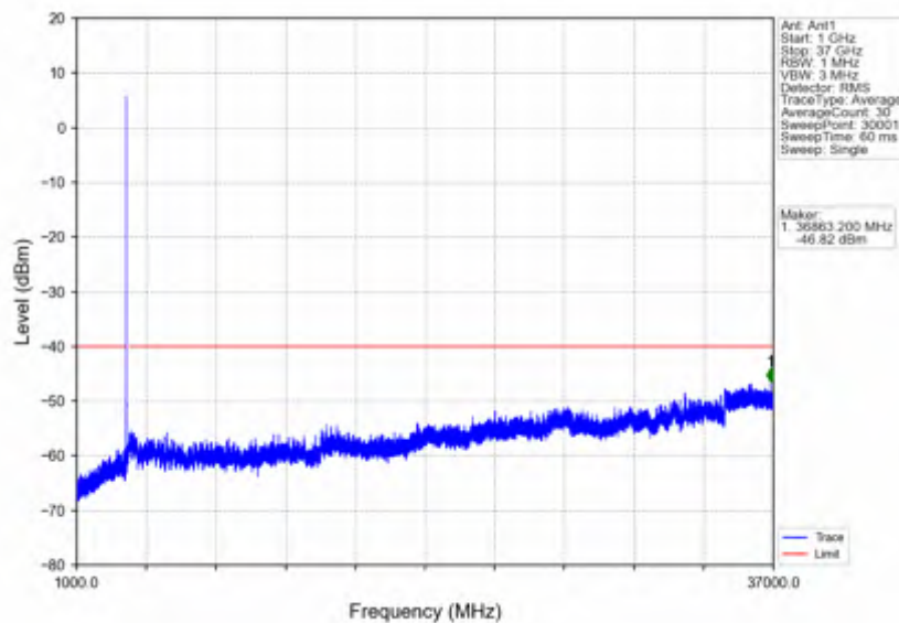
n78d 30kHz SISO NTN 10MHz CP-OFDM QPSK 3555MHz Outer Full
