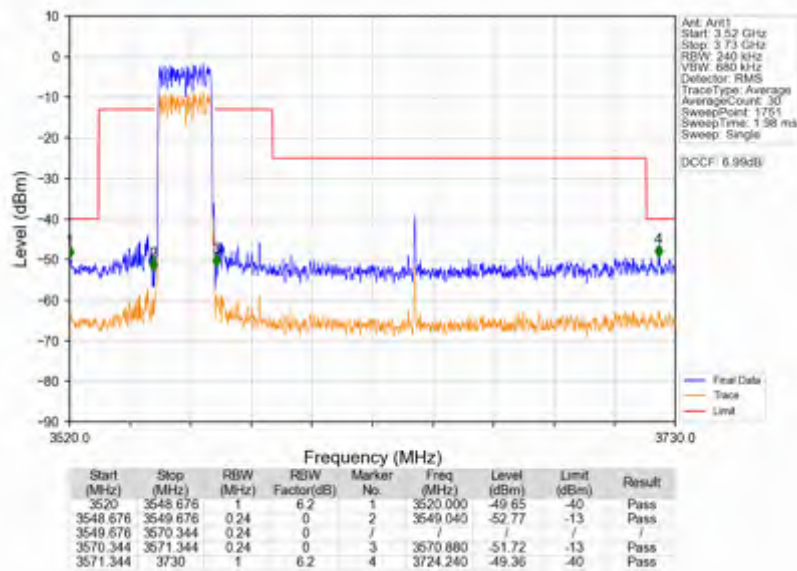
n78d_30kHz_SISO_NTNV_20MHz_CP-OFDM QPSK_3560.01MHz_Outer_Full
