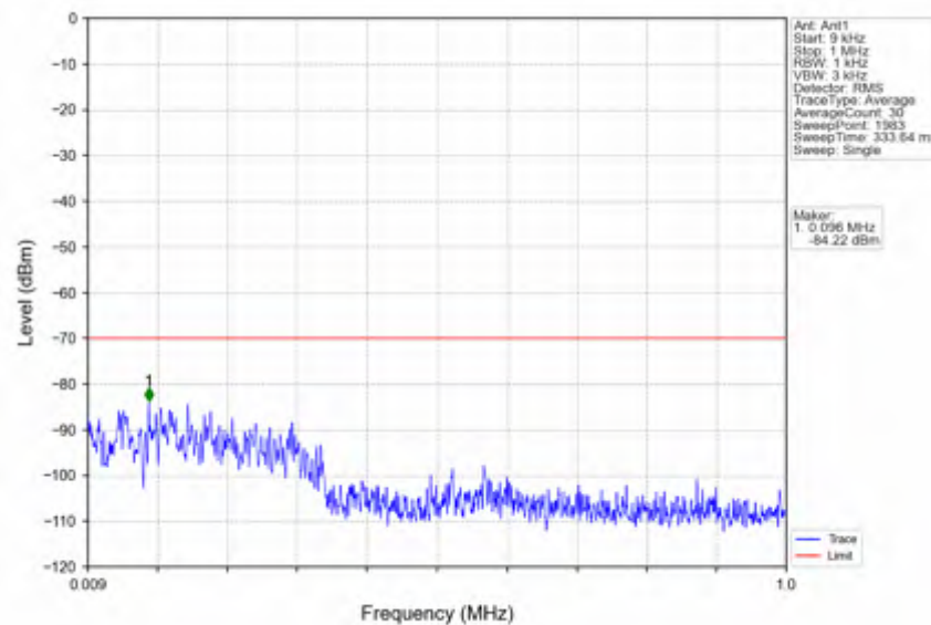
n78d_30kHz_SISO_NTNV_25MHz_DFT-s-OFDM QPSK_3562.5MHz_Edge_1RB_Left
