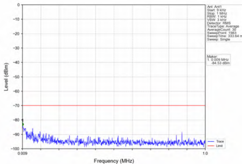
n78d_15kHz_SISO_NTNV_50MHz_CP-OFDM_QPSK_3675MHz_Inner_1RB_Right
