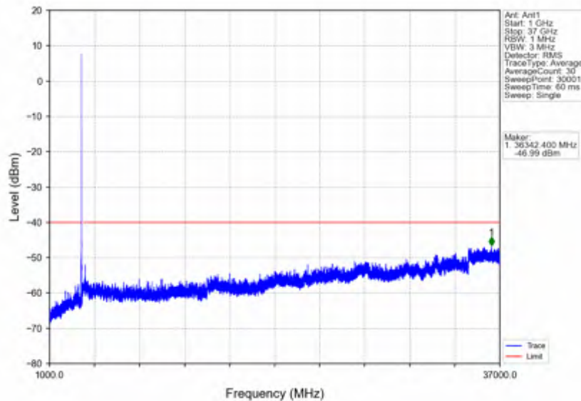
n78d_30kHz_SISO_NTV_10MHz_CP-OFDM_QPSK_3624.99MHz_Edge_1RB_Left
