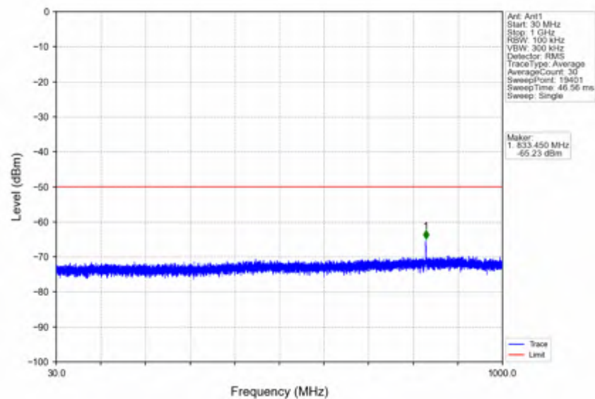
n78d_30kHz_SISO_NTNV_10MHz_DFT-s-OFDM_QPSK_3624.99MHz_Edge_1RB_Left
