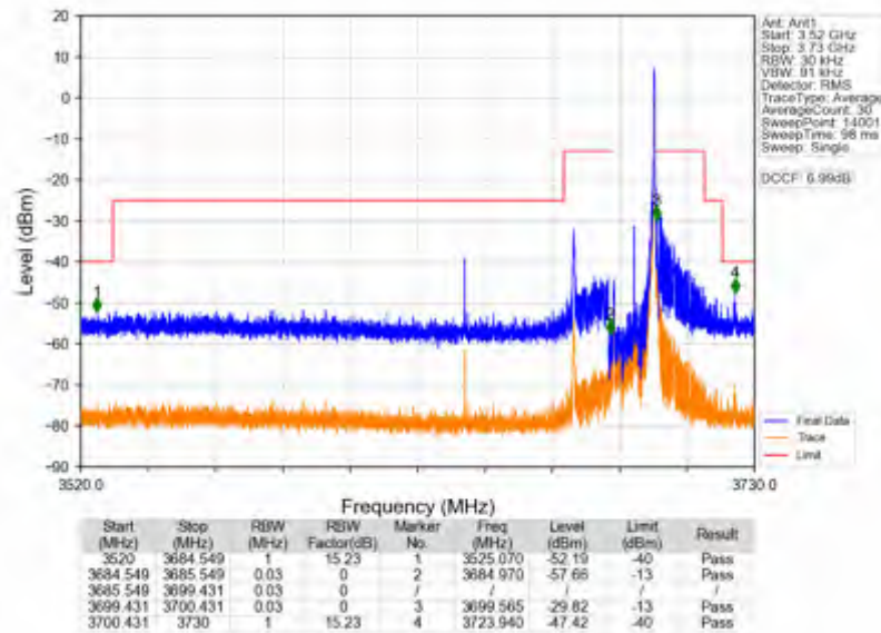
n78d_30kHz_SISO_NTNV_15MHz_CP-OFDM QPSK_3692.49MHz_Inner_1RB_Right
