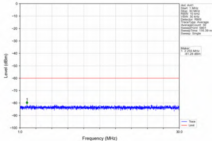
n78d_30kHz_SISO_NTNV_10MHz_DFT-s-OFDM PI/2 BPSK_3555MHz_Edge_1RB_Left
