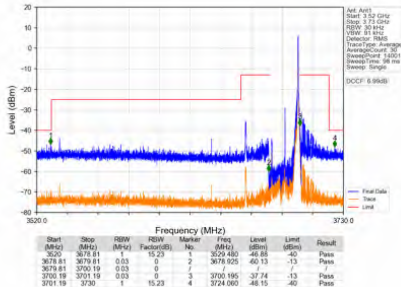
n78d_30kHz_SISO_NTNV_20MHz_CP-OFDM QPSK_3690MHz_Edge_1RB_Right
