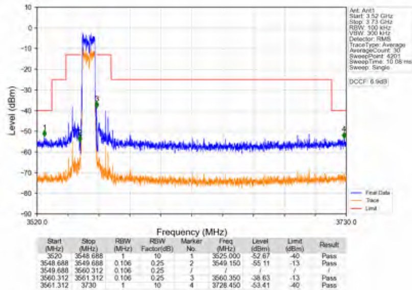
n78d_30kHz_SISO_NTNV_10MHz_DFT-s-OFDM_QPSK_3555MHz_Outer_Full
