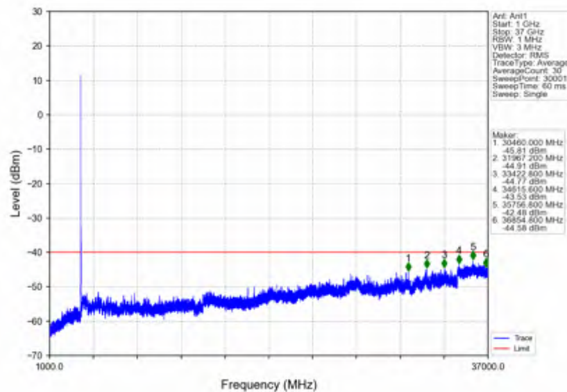
n78d_30kHz_SISO_NTNV_20MHz_DFT-s-OFDM_QPSK_3560.01MHz_Edge_1RB_Left
