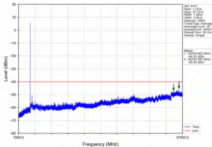
n78d_30kHz_SISO_NTNV_10MHz_DFT-s-OFDM QPSK_3555MHz_Inner_1RB_Left
