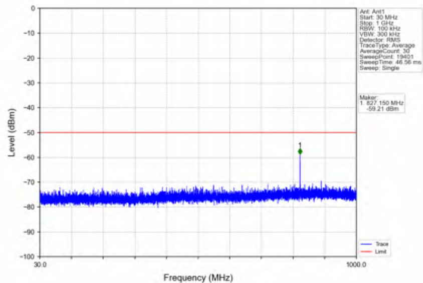
n78d_30kHz_SISO_NTNV_15MHz_CP-OFDM QPSK_3692.49MHz_Inner_1RB_Right
