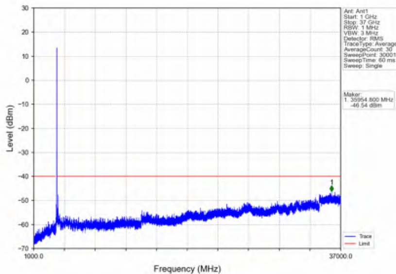
n78d 30kHz SISO NTNv 15MHz CP-OFDM QPSK 3692.49MHz Outer Full
