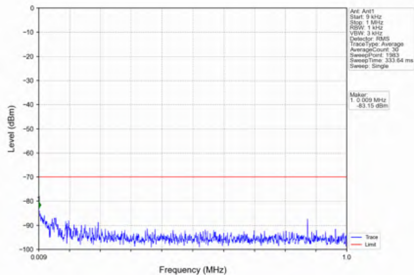
n78d_30kHz_SISO_NTNV_15MHz_DFT-s-OFDM QPSK_3692.49MHz_Inner_1RB_Right
