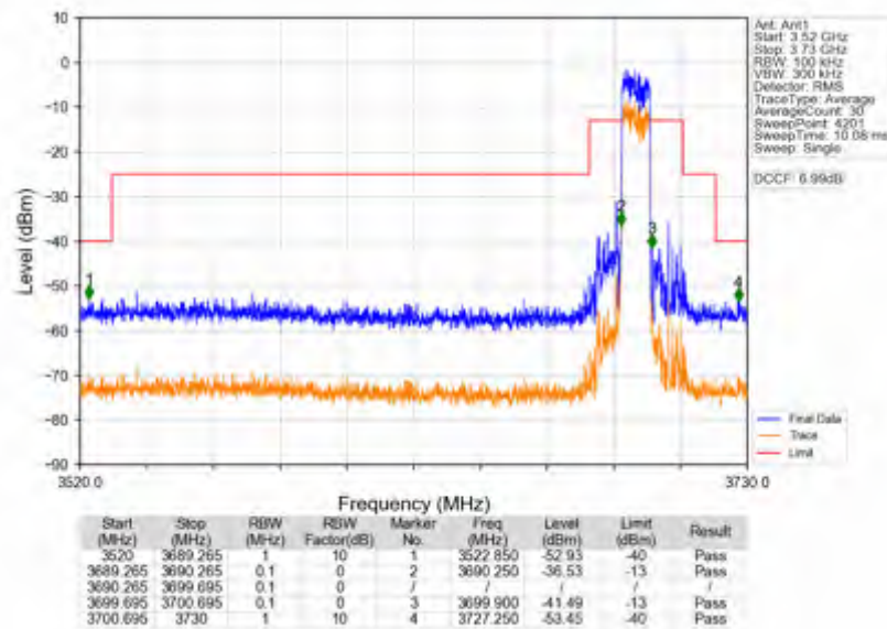
n78d_30kHz_SISO_NTNV_10MHz_DFT-s-OFDM_QPSK_3694.98MHz_Outer_Full
