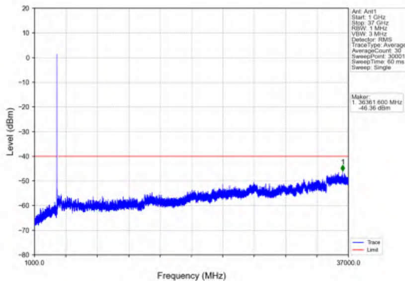
n78d_30kHz_SISO_NTNV_15MHz_DFT-s-OFDM_QPSK_3557.52MHz_Inner_1RB_Left
