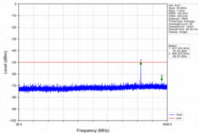
n78d_30kHz_SISO_NTNV_20MHz_DFT-s-OFDM_QPSK_3560.01MHz_Edge_1RB_Left
