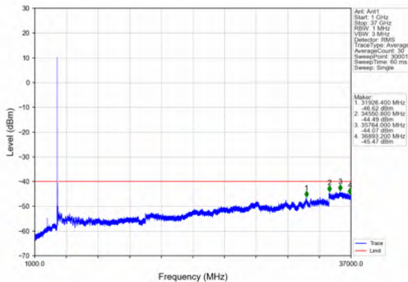
n78d 30kHz SISO NTNV 25MHz DFT-s-OFDM PI/2 BPSK 3562.5MHz Outer Full
