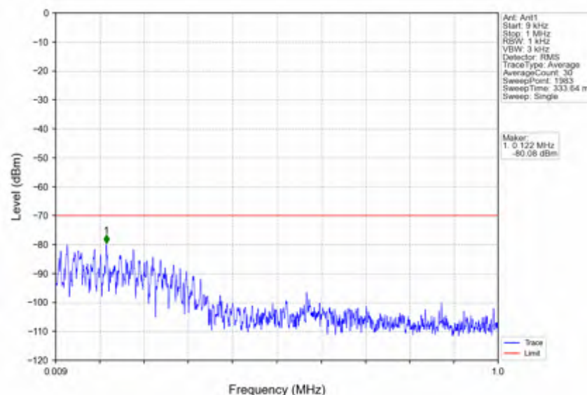
n78d_30kHz_SISO_NTNV_20MHz_CP-OFDM QPSK_3690MHz_Edge_1RB_Right
