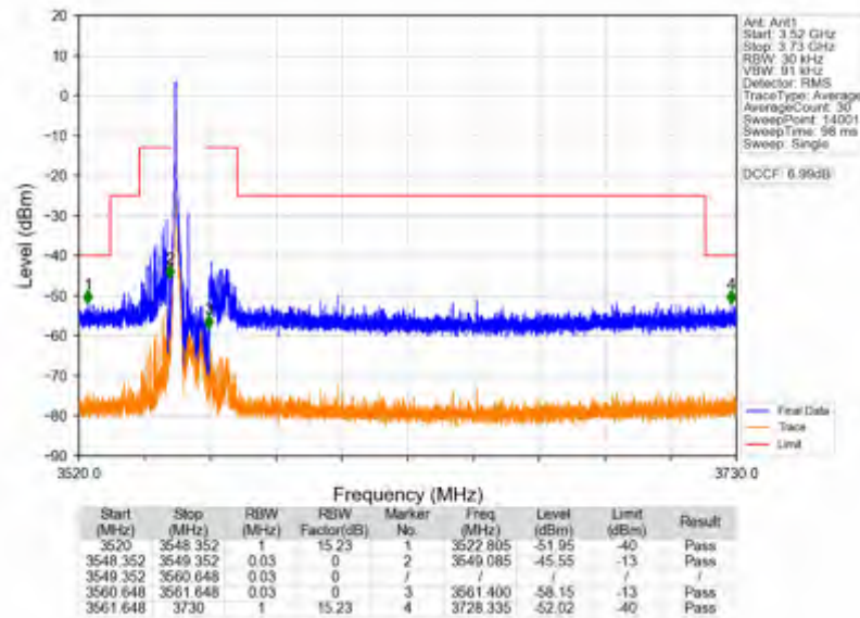
n78d_30kHz_SISO_NTNV_10MHz_CP-OFDM_QPSK_3555MHz_Edge_1RB_Left
