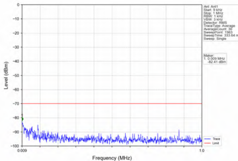
n78d_30kHz_SISO_NTNV_10MHz_CP-OFDM_QPSK_3694.98MHz_Inner_1RB_Right
