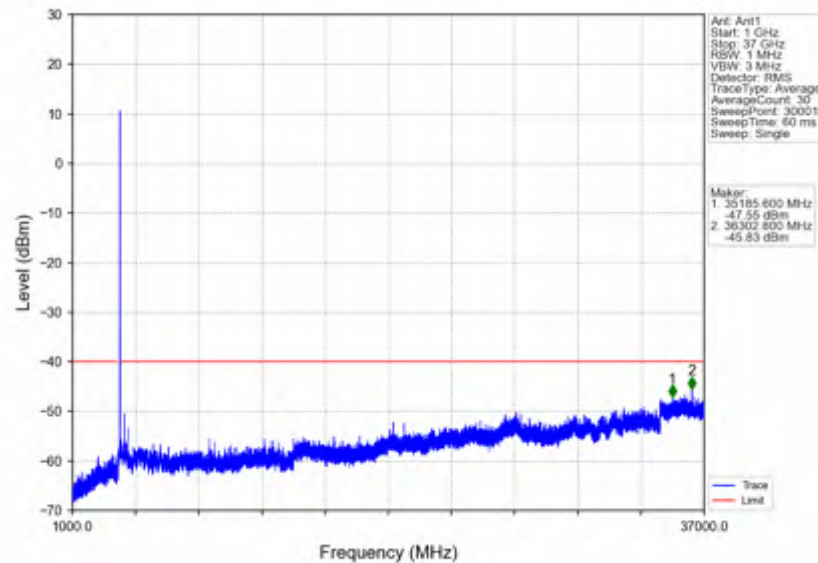
n78d_30kHz_SISO_NTNV_15MHz_DFT-s-OFDM_QPSK_3692.49MHz_Inner_1RB_Right
