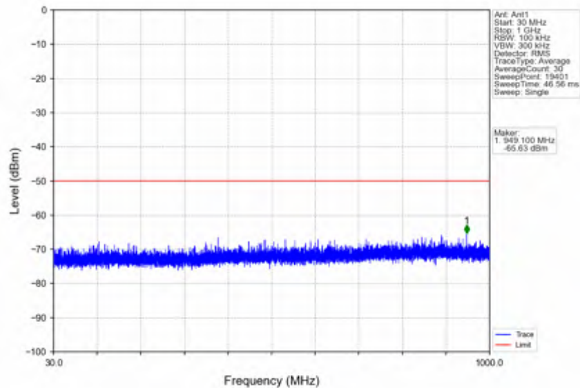
n78d_30kHz_SISO_NTNV_25MHz_DFT-s-OFDM QPSK_3562.5MHz_Edge_1RB_Left
