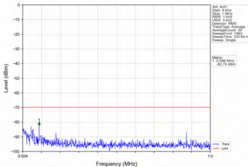
n78d_30kHz_SISO_NTNV_10MHz_CP-OFDM_QPSK_3555MHz_Edge_1RB_Left
