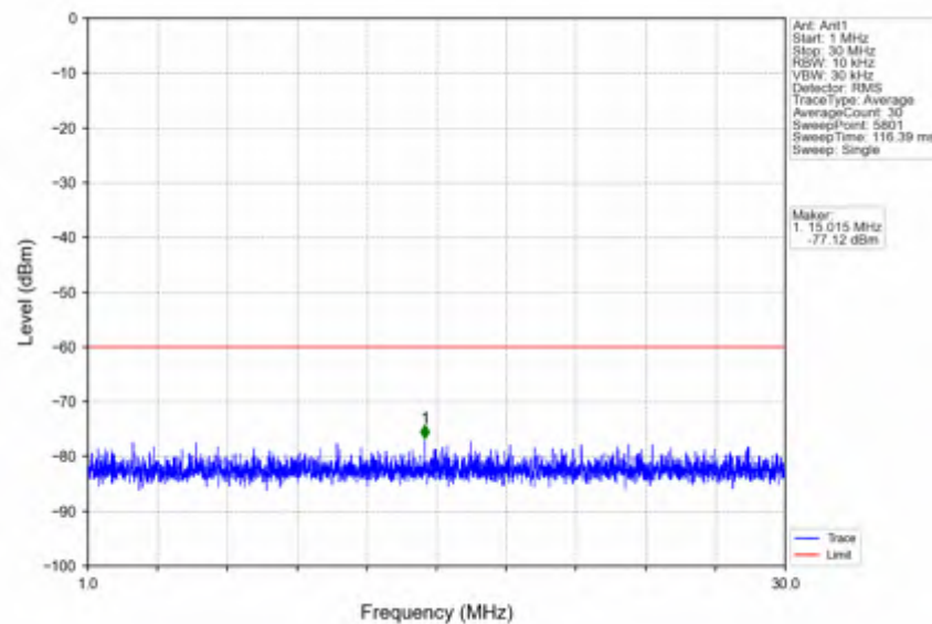
n78d_30kHz_SISO_NTNV_20MHz_CP-OFDM_QPSK_3690MHz_Inner_1RB_Right
