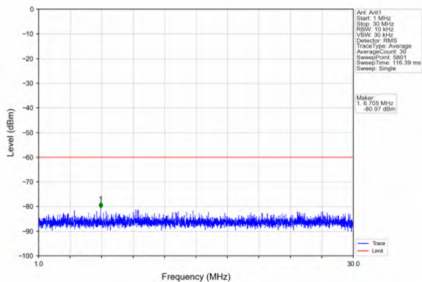
n78d 30kHz SISO NTN 10MHz CP-OFDM QPSK 3555MHz Outer Full
