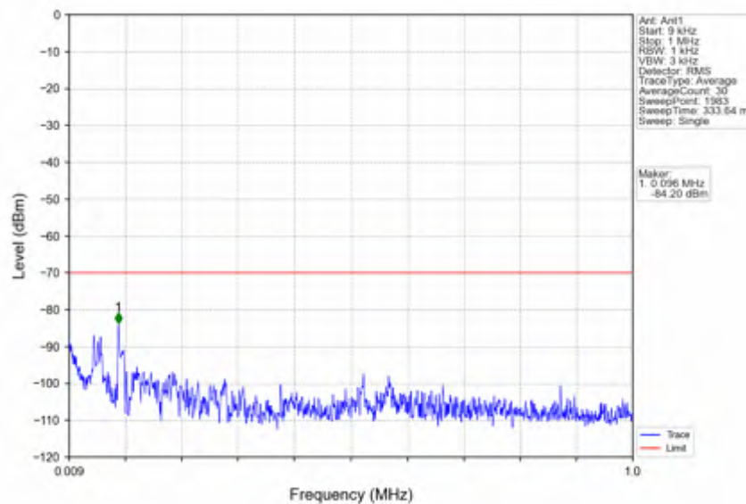
n78d_30kHz_SISO_NTNV_25MHz_DFT-s-OFDM QPSK_3562.5MHz_Outer_Full
