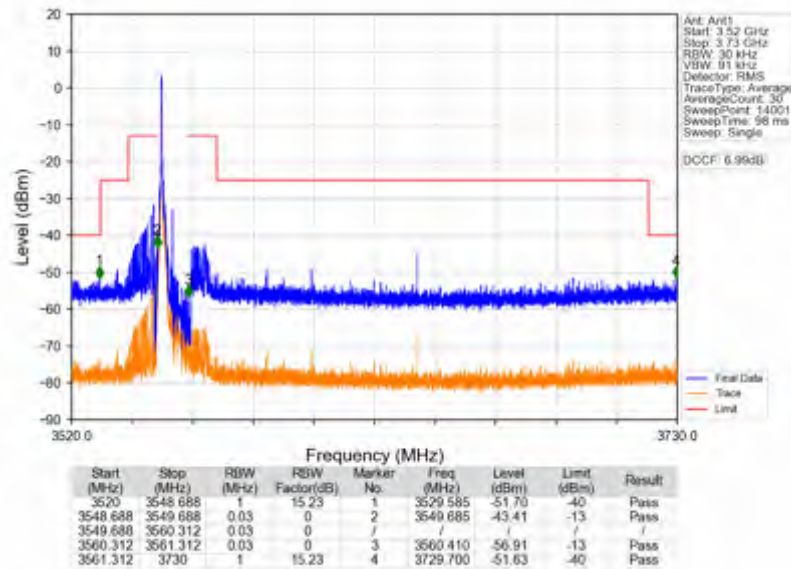
n78d_30kHz_SISO_NTNV_10MHz_DFT-s-OFDM QPSK_3555MHz_Inner_1RB_Left
