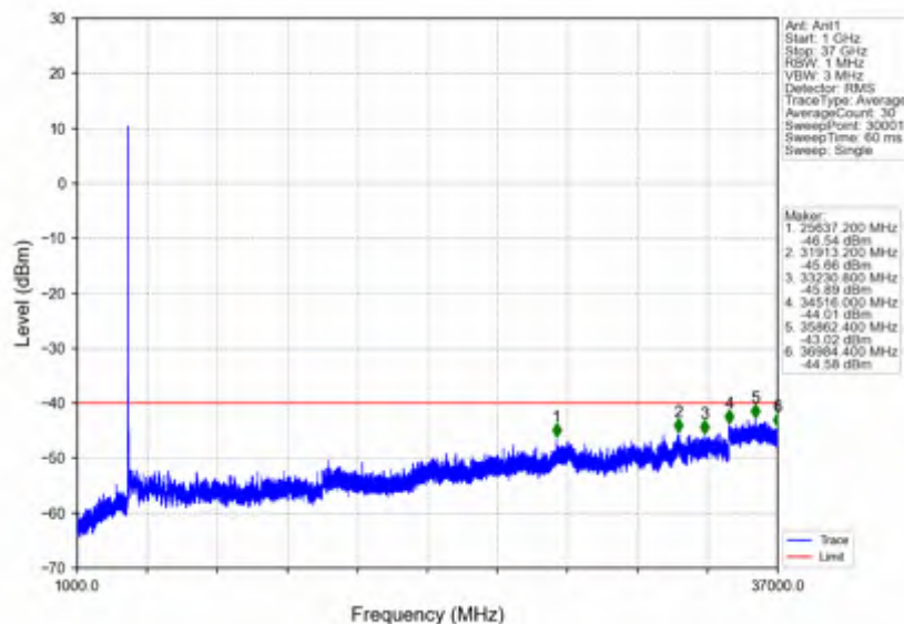
n78d_30kHz_SISO_NTNV_20MHz_DFT-s-OFDM QPSK_3690MHz_Edge_1RB_Right
