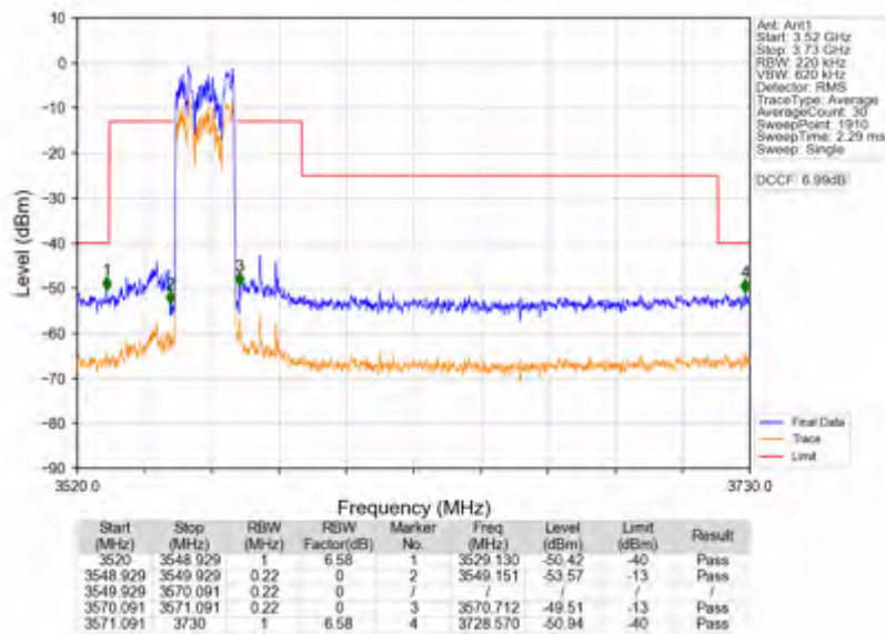
n78d_30kHz_SISO_NTNV_20MHz_DFT-s-OFDM PI/2 BPSK_3560.01MHz_Outer_Full
