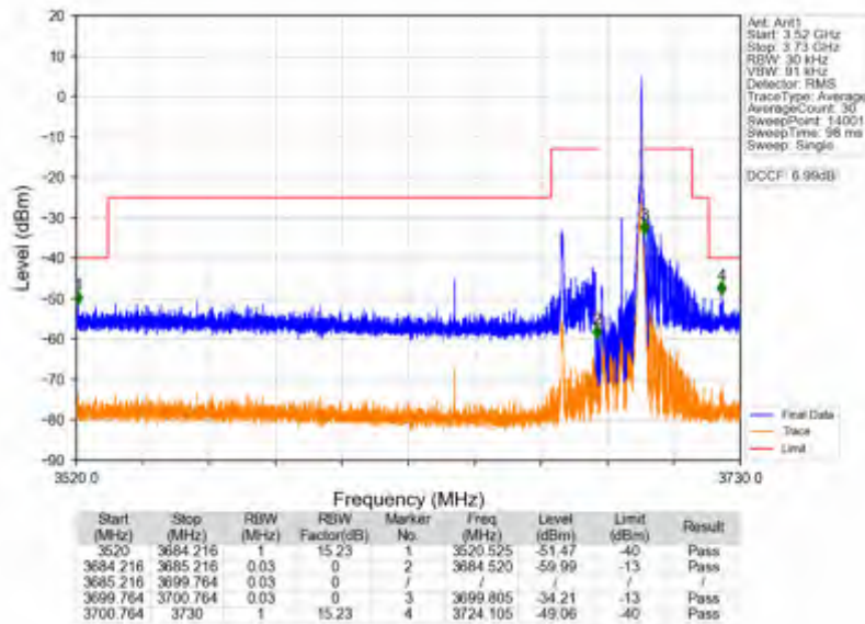
n78d_30kHz_SISO_NTNV_15MHz_DFT-s-OFDM QPSK_3692.49MHz_Inner_1RB_Right
