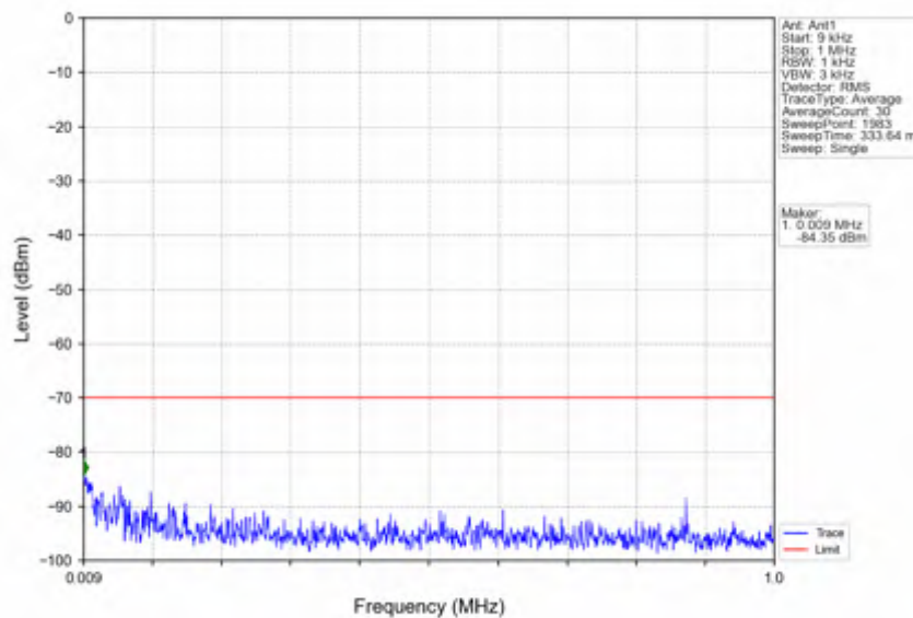
n78d_30kHz_SISO_NTNV_10MHz_DFT-s-OFDM_QPSK_3555MHz_Outer_Full
