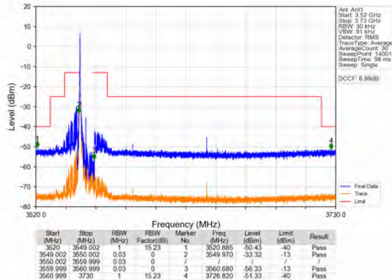
n78d_30kHz_SISO_NTNV_10MHz_DFT-s-OFDM_PI/2_BPSK_3555MHz_Edge_1RB_Left
