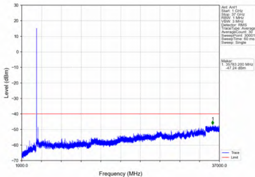
n78d 30kHz SISO NTNv 10MHz CP-OFDM QPSK 3694.98MHz Outer Full
