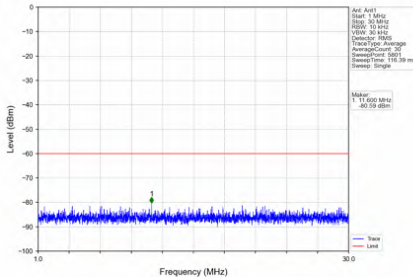
n78d_30kHz_SISO_NTNV_10MHz_CP-OFDM_QPSK_3555MHz_Edge_1RB_Left
