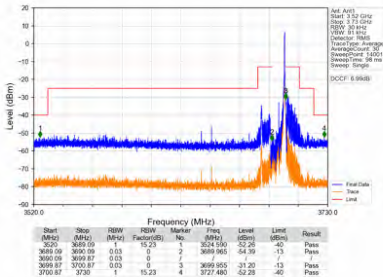
n78d_30kHz_SISO_NTNV_10MHz_DFT-s-OFDM QPSK_3694.98MHz_Edge_1RB_Right
