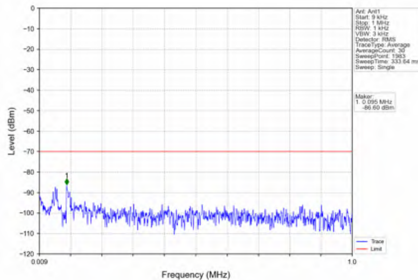
n78d 30kHz SISO NTN 20MHz CP-OFDM QPSK 3690MHz Outer Full
