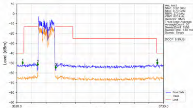
n78d 30kHz SISO NTNV 25MHz DFT-s-OFDM PI/2 BPSK 3562.5MHz Outer Full
