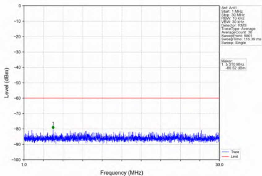
n78d 15kHz SISO NTN 50MHz CP-OFDM QPSK 3675MHz Outer Full
