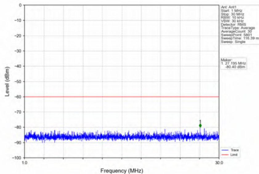
n78d_30kHz_SISO_NTNV_15MHz_DFT-s-OFDM_QPSK_3557.52MHz_Outer_Full
