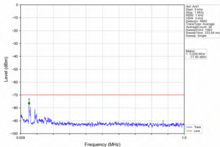
n78d_30kHz_SISO_NTNV_20MHz_DFT-s-OFDM PI/2 BPSK_3560.01MHz_Edge_1RB_Left
