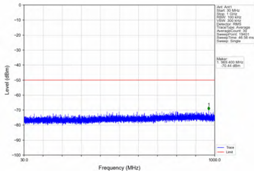
n78d_30kHz_SISO_NTNV_10MHz_CP-OFDM QPSK_3694.98MHz_Inner_1RB_Right
