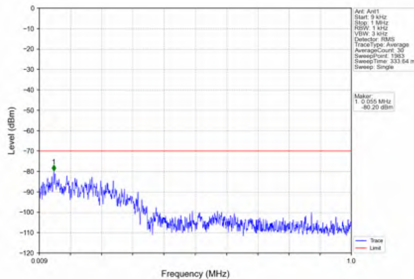
n78d_30kHz_SISO_NTNV_20MHz_CP-OFDM_QPSK_3690MHz_Inner_1RB_Right
