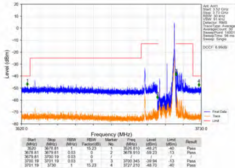
n78d_30kHz_SISO_NTNV_20MHz_CP-OFDM_QPSK_3690MHz_Inner_1RB_Right
