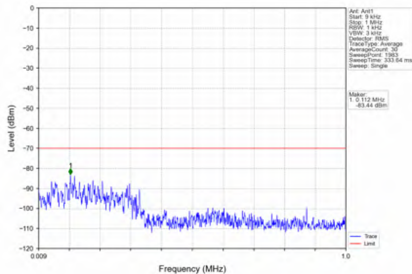
n78d_30kHz_SISO_NTNV_20MHz_DFT-s-OFDM QPSK_3690MHz_Inner_1RB_Right
