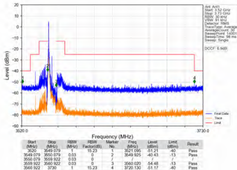
n78d_30kHz_SISO_NTNV_10MHz_CP-OFDM_QPSK_3555MHz_Inner_1RB_Left
