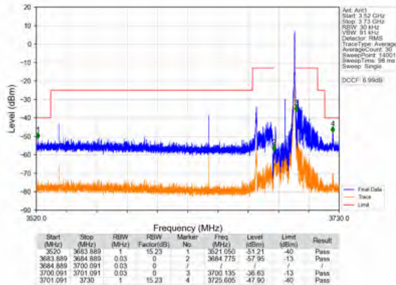
n78d_30kHz_SISO_NTNV_15MHz_CP-OFDM QPSK_3692.49MHz_Edge_1RB_Right
