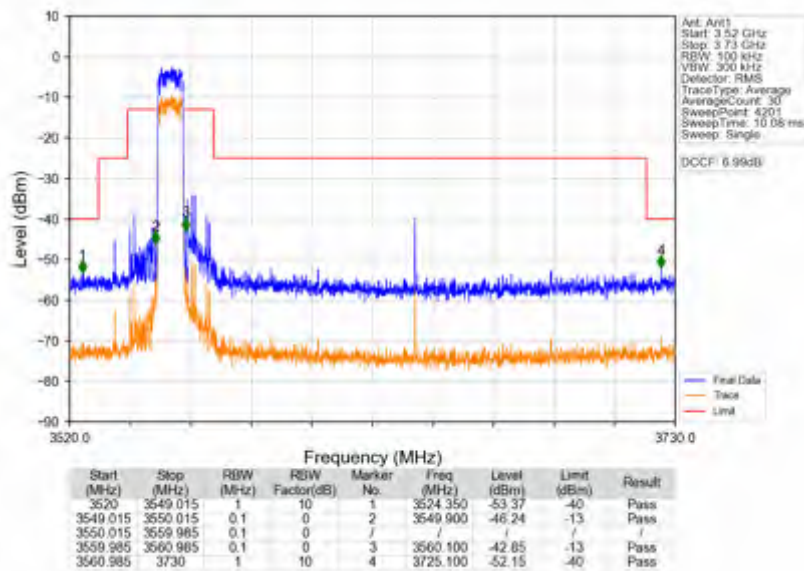
n78d_30kHz_SISO_NTNV_10MHz_CP-OFDM QPSK_3555MHz_Outer_Full
