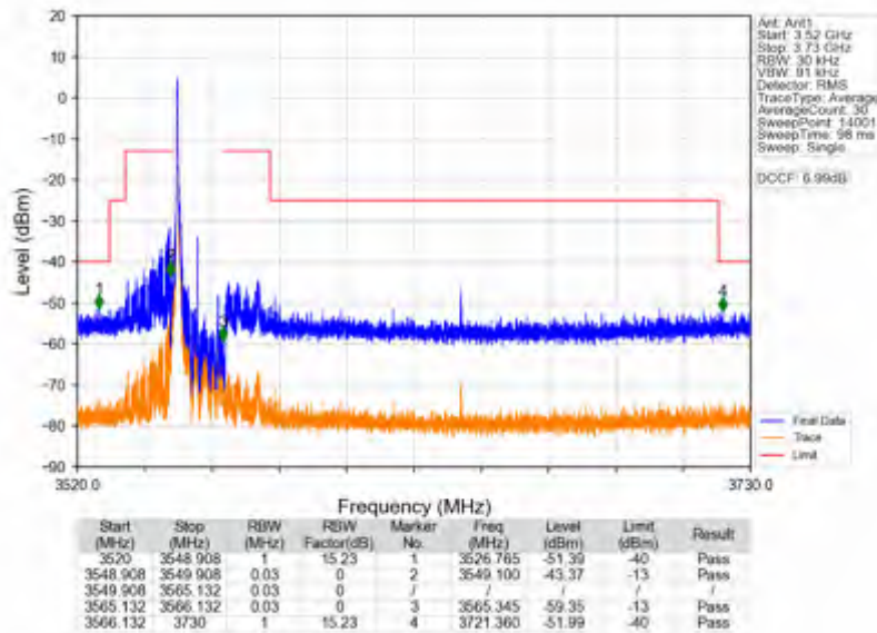
n78d_30kHz_SISO_NTNV_15MHz_DFT-s-OFDM_QPSK_3557.52MHz_Inner_1RB_Left
