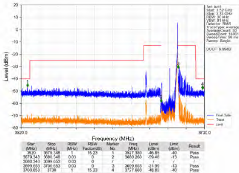
n78d_30kHz_SISO_NTNV_20MHz_DFT-s-OFDM QPSK_3690MHz_Edge_1RB_Right
