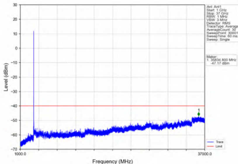
n78d_30kHz_SISO_NTNV_15MHz_DFT-s-OFDM QPSK_3692.49MHz_Edge_1RB_Right
