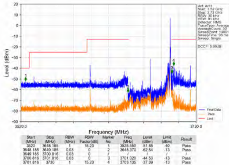
n78d_15kHz_SISO_NTNV_50MHz_CP-OFDM_QPSK_3675MHz_Inner_1RB_Right
