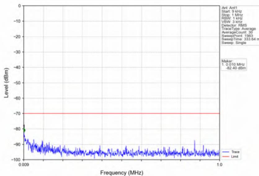
n78d_30kHz_SISO_NTNV_15MHz_DFT-s-OFDM_QPSK_3692.49MHz_Outer_Full
