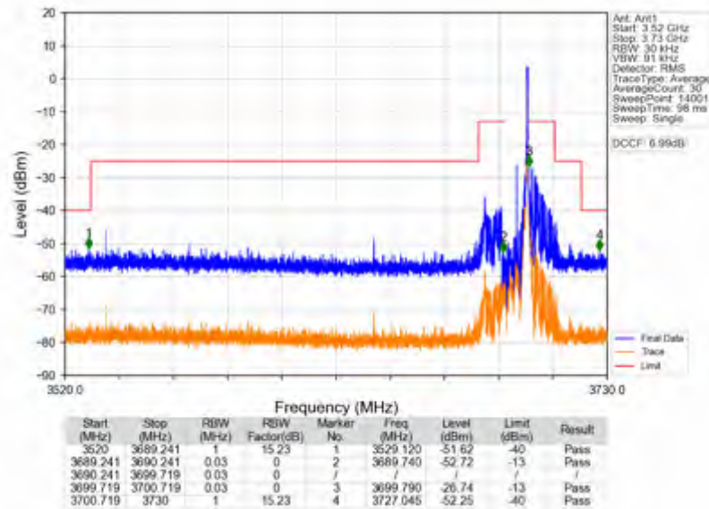
n78d_30kHz_SISO_NTNV_10MHz_CP-OFDM QPSK_3694.98MHz_Edge_1RB_Right
