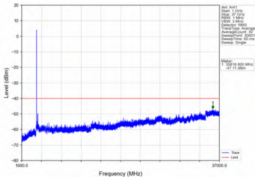
n78d_30kHz_SISO_NTNV_15MHz_DFT-s-OFDM QPSK_3692.49MHz_Inner_1RB_Right
