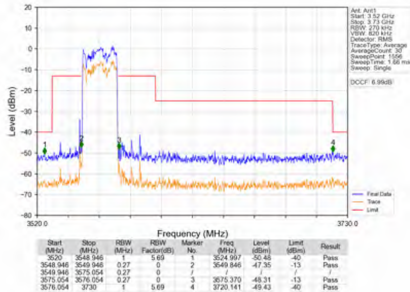
n78d_30kHz_SISO_NTNV_25MHz_DFT-s-OFDM QPSK_3562.5MHz_Outer_Full
