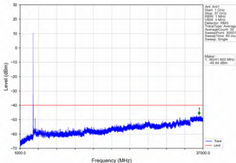
n78d_30kHz_SISO_NTV_15MHz_CP-OFDM QPSK_3624.99MHz_Edge_1RB_Left
