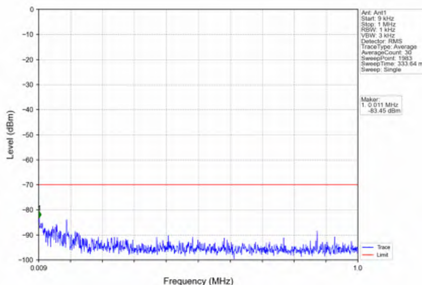
n78d_30kHz_SISO_NTNV_10MHz_CP-OFDM_QPSK_3555MHz_Inner_1RB_Left
