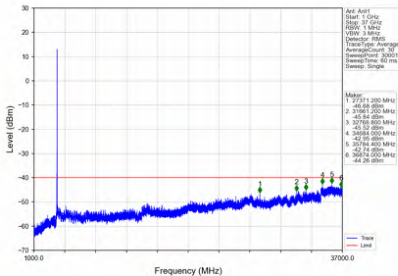
n78d_30kHz_SISO_NTNV_20MHz_CP-OFDM QPSK_3690MHz_Outer_Full
