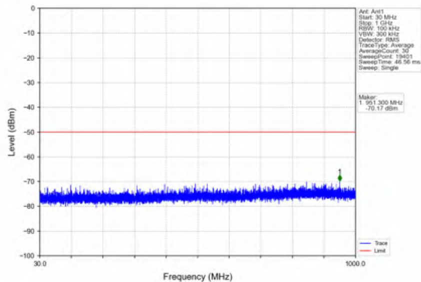
n78d_30kHz_SISO_NTNV_10MHz_DFT-s-OFDM QPSK_3694.98MHz_Inner_1RB_Right
