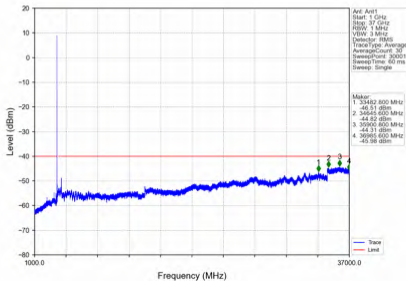
n78d_30kHz_SISO_NTNV_10MHz_DFT-s-OFDM PI/2 BPSK_3624.99MHz_Edge_1RB_Left
