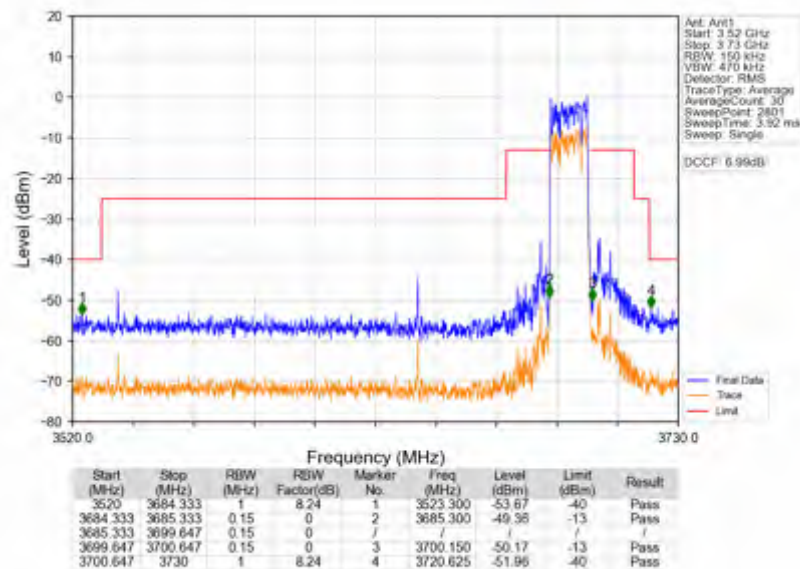
n78d_30kHz_SISO_NTNV_15MHz_DFT-s-OFDM_QPSK_3692.49MHz_Outer_Full
