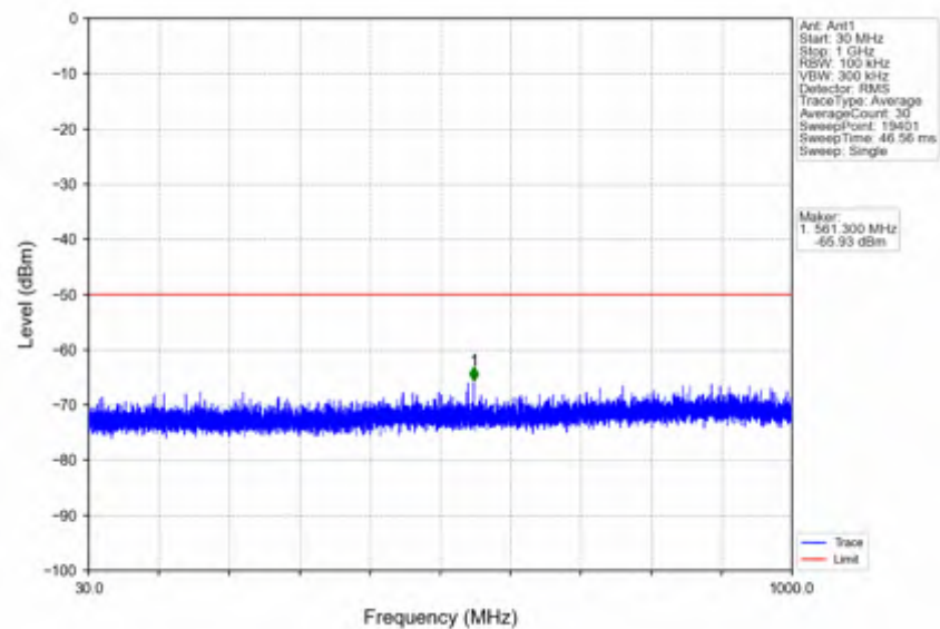
n78d_30kHz_SISO_NTNV_25MHz_DFT-s-OFDM QPSK_3562.5MHz_Outer_Full
