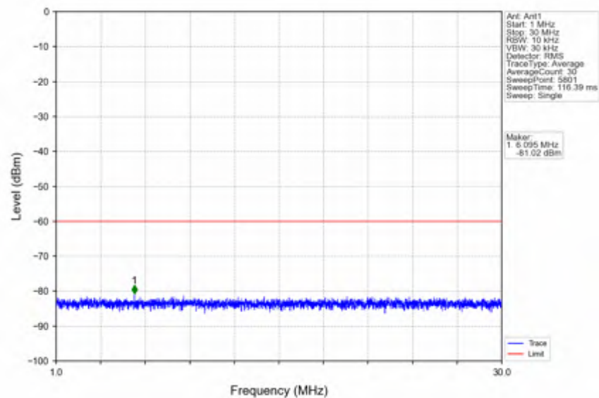
n78d_30kHz_SISO_NTNV_10MHz_DFT-s-OFDM_QPSK_3624.99MHz_Edge_1RB_Left
