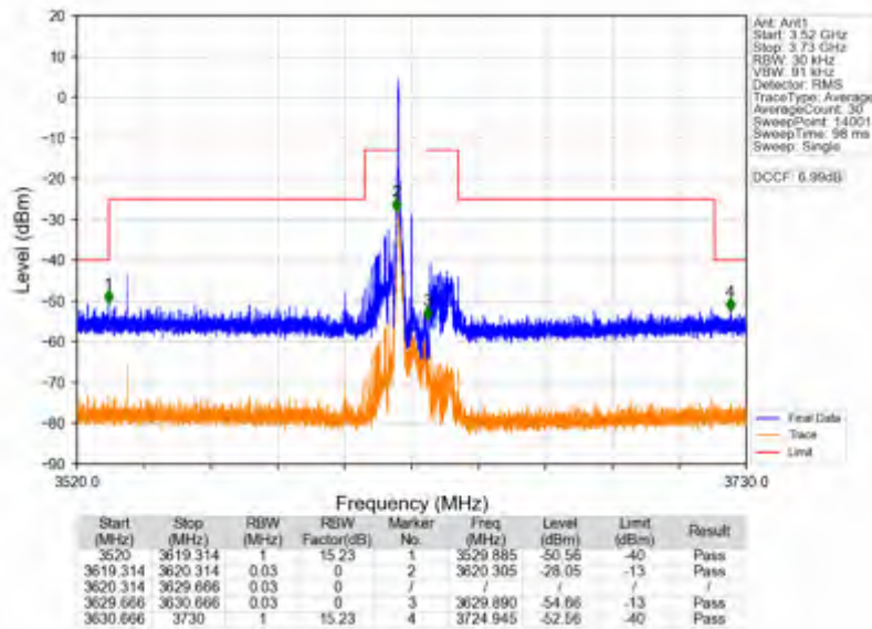
n78d_30kHz_SISO_NTV_10MHz_CP-OFDM_QPSK_3624.99MHz_Edge_1RB_Left
