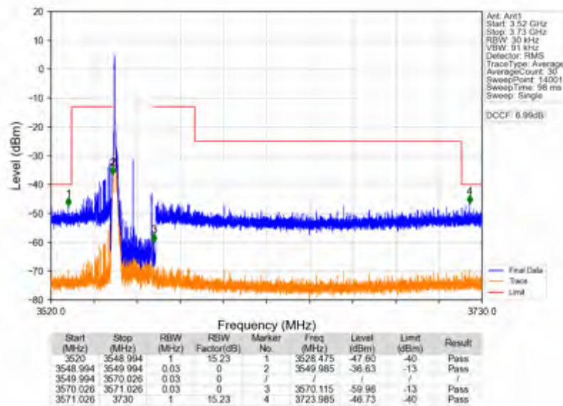
n78d_30kHz_SISO_NTNV_20MHz_DFT-s-OFDM QPSK_3560.01MHz_Edge_1RB_Left
