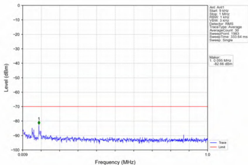
n78d_30kHz_SISO_NTNV_10MHz_DFT-s-OFDM_PI/2_BPSK_3555MHz_Edge_1RB_Left
