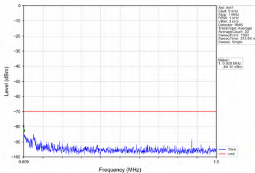
n78d_30kHz_SISO_NTNV_15MHz_DFT-s-OFDM_QPSK_3557.52MHz_Outer_Full
