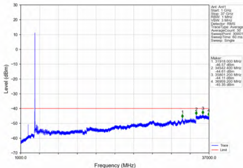
n78d_30kHz_SISO_NTNV_20MHz_DFT-s-OFDM PI/2 BPSK_3690MHz_Outer_Full
