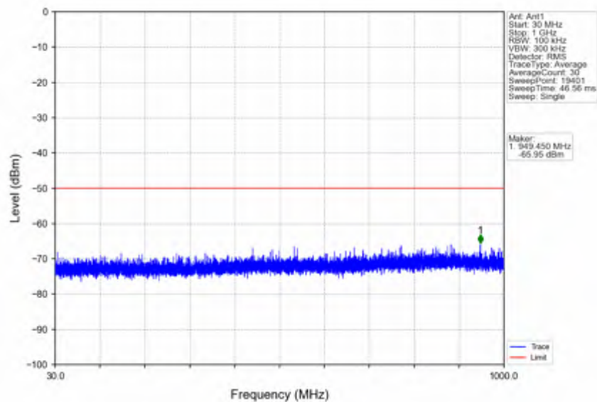
n78d_30kHz_SISO_NTNV_20MHz_CP-OFDM_QPSK_3690MHz_Outer_Full
