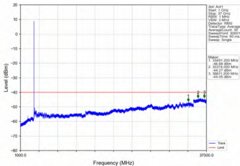
n78d_30kHz_SISO_NTNV_10MHz_DFT-s-OFDM QPSK_3694.98MHz_Edge_1RB_Right
