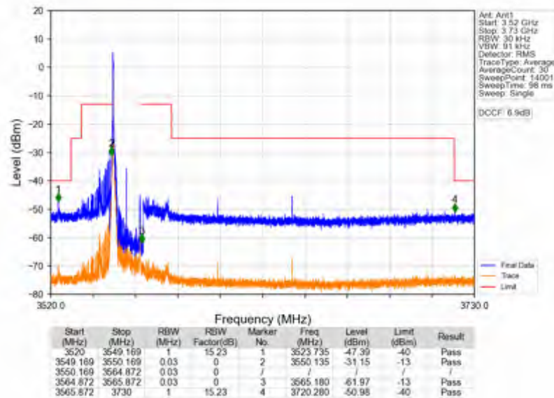
n78d_30kHz_SISO_NTNV_15MHz_DFT-s-OFDM PI/2 BPSK_3557.52MHz_Edge_1RB_Left
