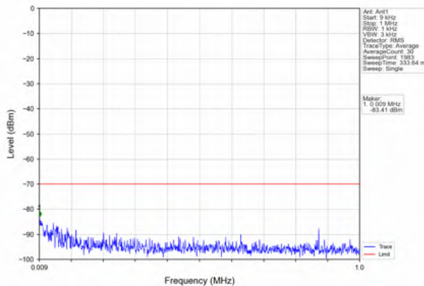
n78d_30kHz_SISO_NTNV_15MHz_CP-OFDM QPSK_3692.49MHz_Inner_1RB_Right
