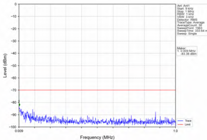
n78d_30kHz_SISO_NTNV_15MHz_CP-OFDM QPSK_3692.49MHz_Edge_1RB_Right
