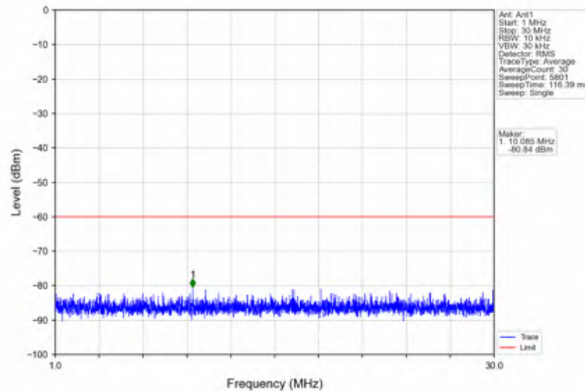
n78d_30kHz_SISO_NTNV_10MHz_CP-OFDM QPSK_3694.98MHz_Edge_1RB_Right
