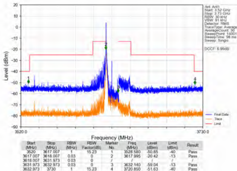
n78d_30kHz_SISO_NTV_15MHz_CP-OFDM QPSK_3624.99MHz_Edge_1RB_Left
