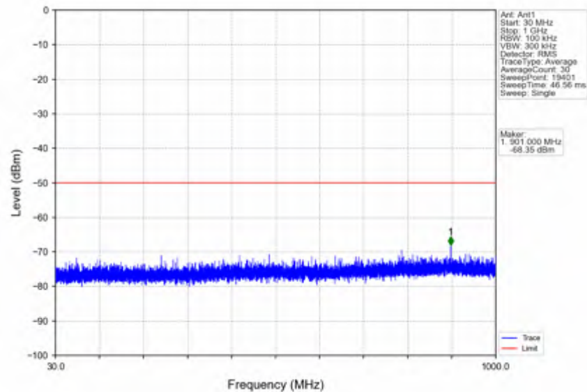
n78d_30kHz_SISO_NTNV_15MHz_DFT-s-OFDM_QPSK_3692.49MHz_Inner_1RB_Right
