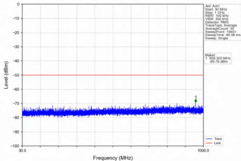
n78d_30kHz_SISO_NTNV_10MHz_DFT-s-OFDM_QPSK_3694.98MHz_Edge_1RB_Right
