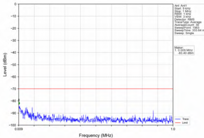
n78d_30kHz_SISO_NTNV_10MHz_CP-OFDM QPSK_3694.98MHz_Edge_1RB_Right
