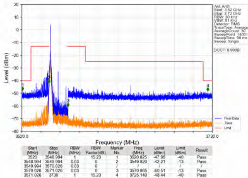
n78d_30kHz_SISO_NTNV_20MHz_DFT-s-OFDM_QPSK_3560.01MHz_Inner_1RB_Left
