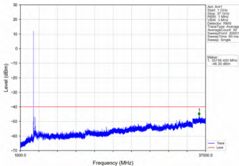
n78d_30kHz_SISO_NTNV_10MHz_CP-OFDM QPSK_3555MHz_Outer_Full
