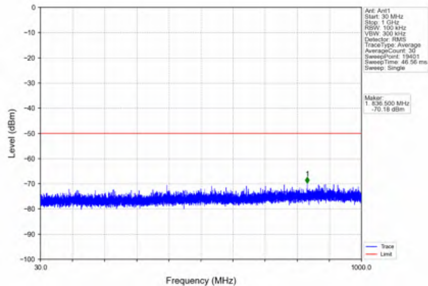
n78d_30kHz_SISO_NTNV_10MHz_CP-OFDM QPSK_3694.98MHz_Outer_Full
