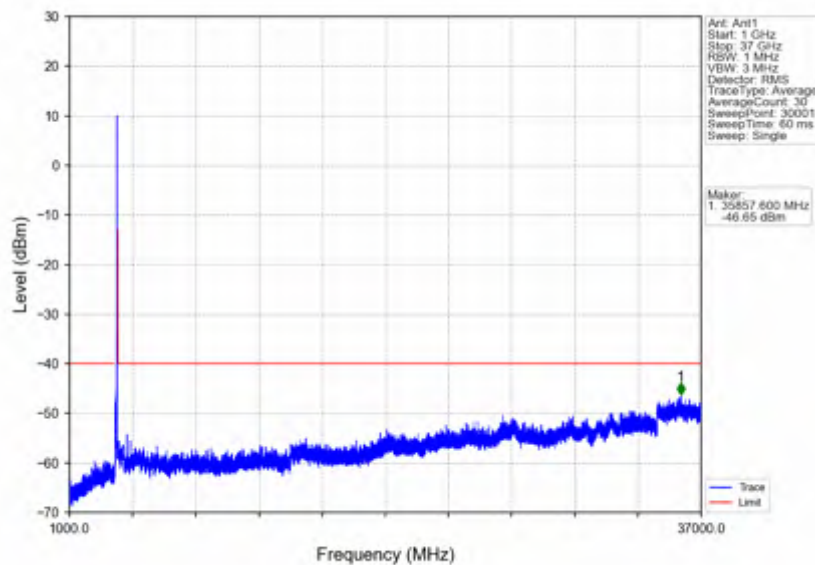
n78d_15kHz_SISO_NTNV_50MHz_CP-OFDM QPSK_3675MHz_Outer_Full
