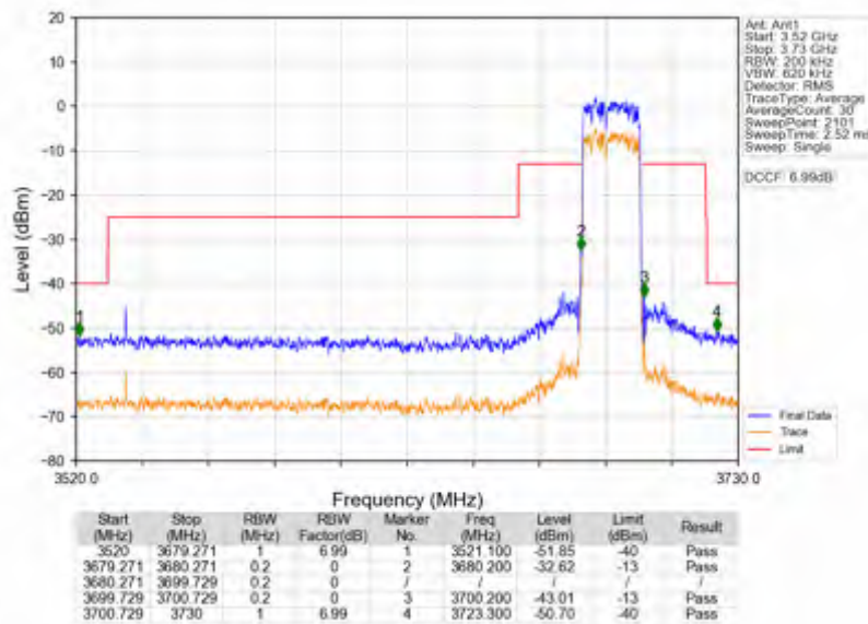
n78d_30kHz_SISO_NTNV_20MHz_DFT-s-OFDM PI/2 BPSK_3690MHz_Outer_Full
