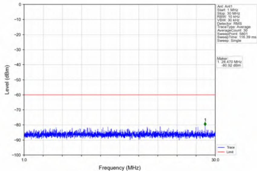
n78d_30kHz_SISO_NTNV_10MHz_DFT-s-OFDM QPSK_3694.98MHz_Edge_1RB_Right
