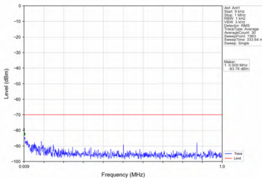
n78d_30kHz_SISO_NTNV_10MHz_DFT-s-OFDM_QPSK_3694.98MHz_Outer_Full
