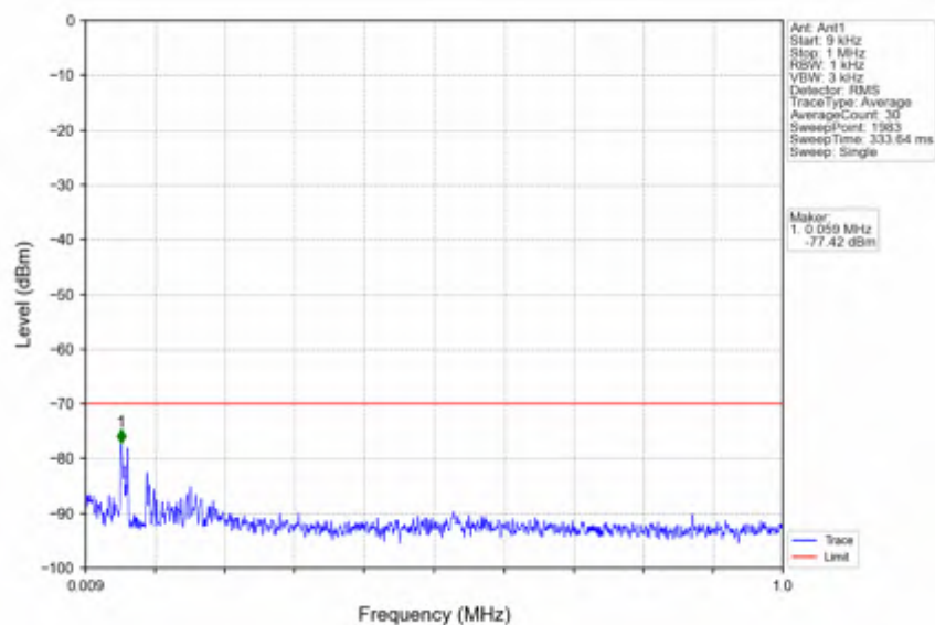
n78d_30kHz_SISO_NTNV_15MHz_DFT-s-OFDM PI/2 BPSK_3557.52MHz_Edge_1RB_Left
