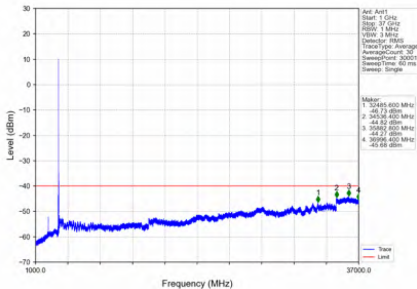
n78d_30kHz_SISO_NTNV_20MHz_DFT-s-OFDM PI/2 BPSK_3560.01MHz_Outer_Full
