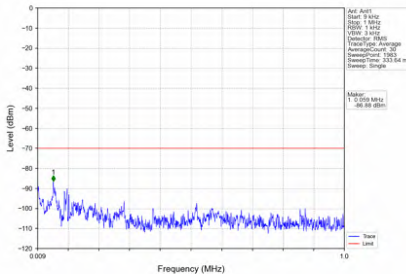
n78d_30kHz_SISO_NTNV_20MHz_DFT-s-OFDM_QPSK_3560.01MHz_Outer_Full
