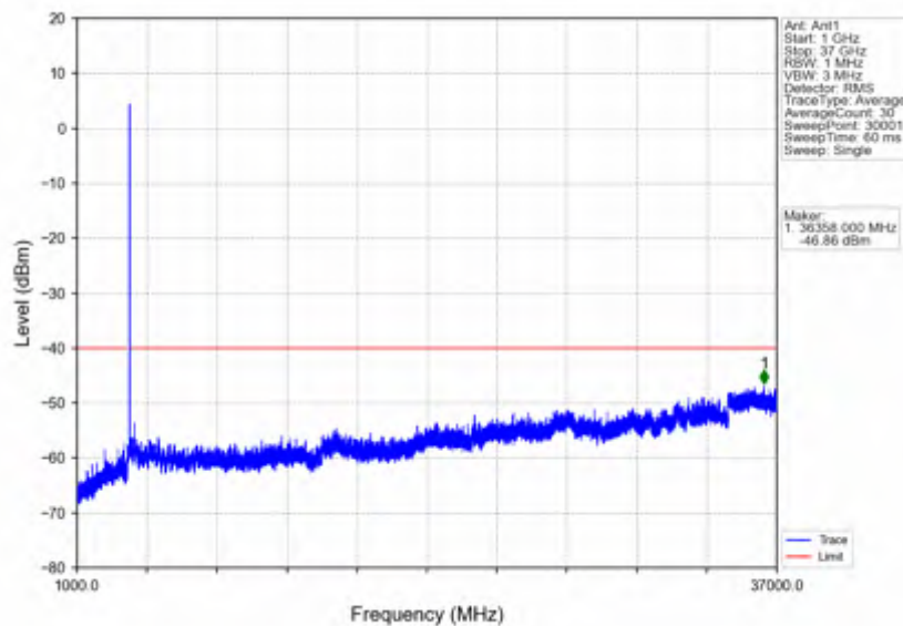
n78d_30kHz_SISO_NTNV_10MHz_DFT-s-OFDM QPSK_3694.98MHz_Inner_1RB_Right
