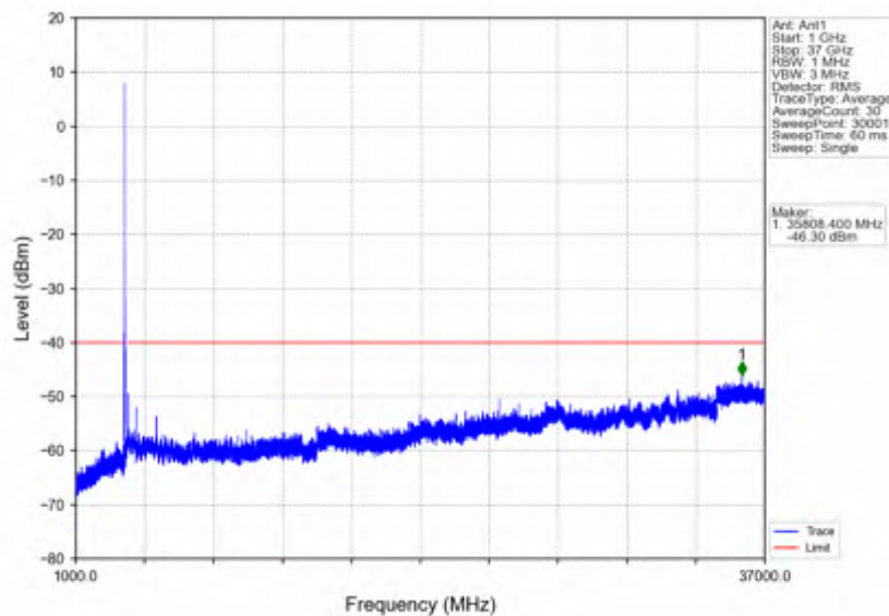
n78d_30kHz_SISO_NTV_15MHz_CP-OFDM QPSK_3557.52MHz_Outer_Full
