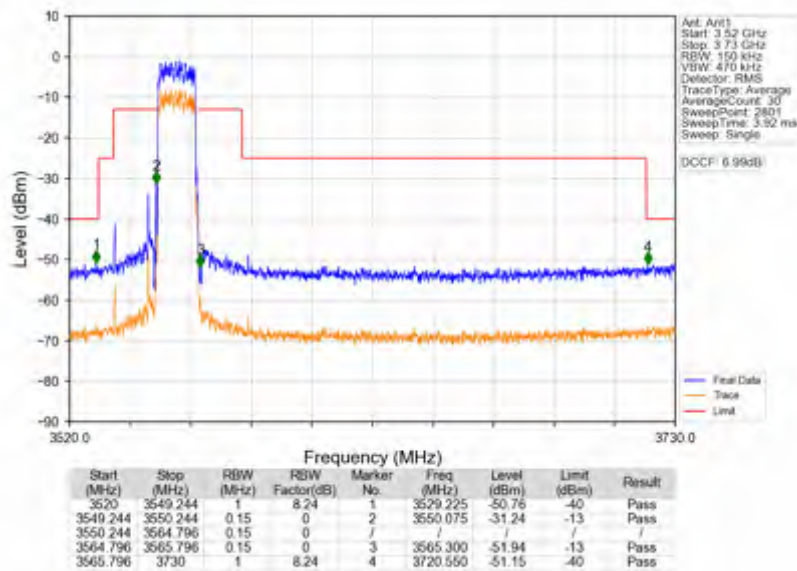
n78d 30kHz SISO NTNV 15MHz DFT-s-OFDM PI/2 BPSK 3557.52MHz Outer Full
