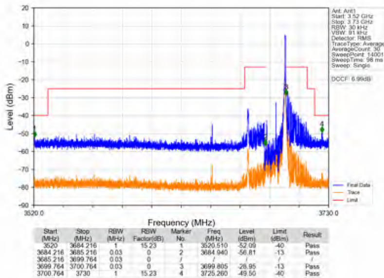
n78d_30kHz_SISO_NTNV_15MHz_DFT-s-OFDM QPSK_3692.49MHz_Edge_1RB_Right
