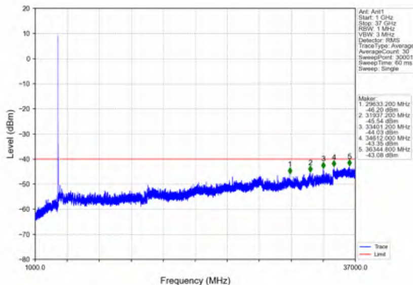
n78d_30kHz_SISO_NTNV_20MHz_CP-OFDM QPSK_3560.01MHz_Outer_Full
