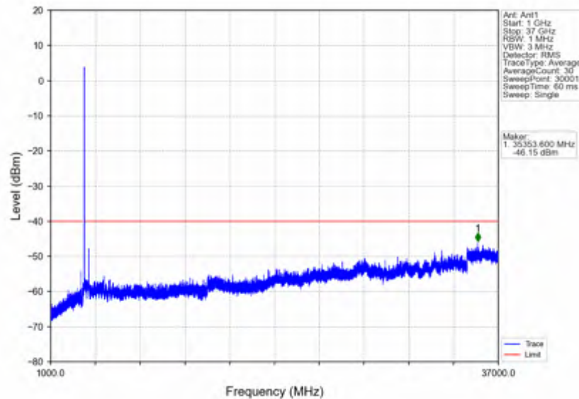
n78d_30kHz_SISO_NTNV_10MHz_CP-OFDM QPSK_3694.98MHz_Outer_Full
