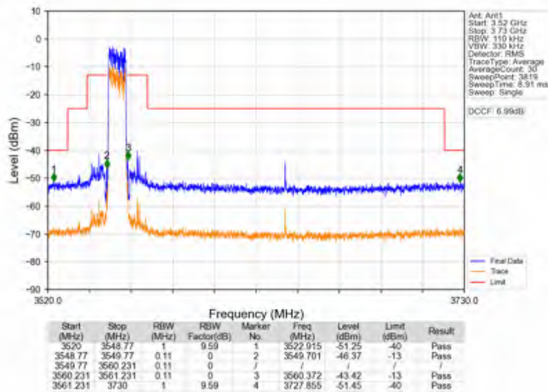
n78d_30kHz_SISO_NTNV_10MHz_DFT-s-OFDM_PI/2_BPSK_3555MHz_Outer_Full
