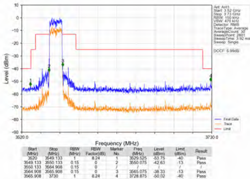
n78d_30kHz_SISO_NTV_15MHz_CP-OFDM QPSK_3557.52MHz_Outer_Full
