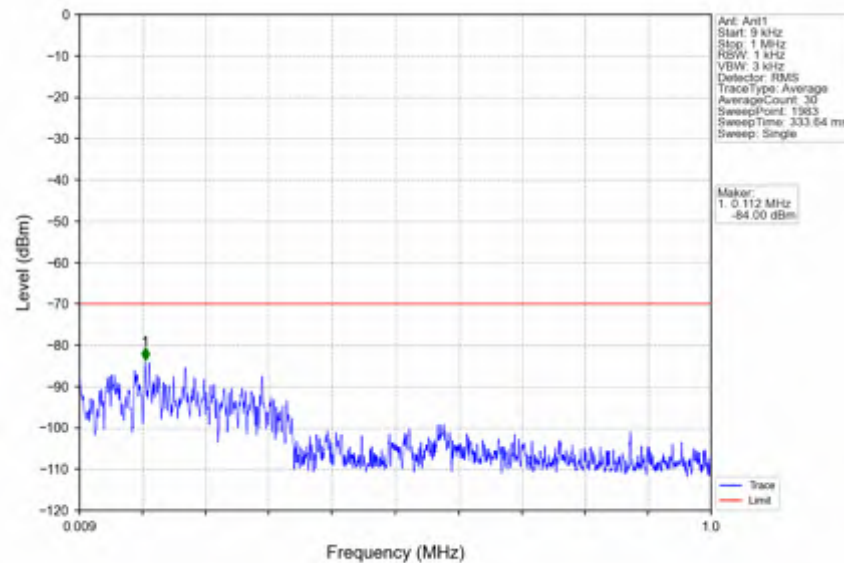
n78d_30kHz_SISO_NTNV_20MHz_DFT-s-OFDM QPSK_3690MHz_Edge_1RB_Right
