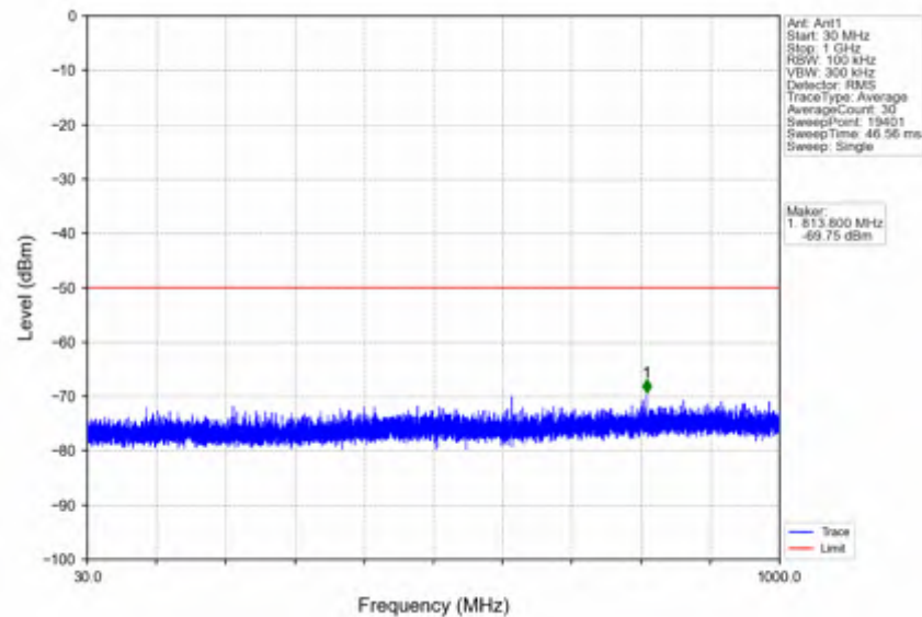
n78d_30kHz_SISO_NTNV_10MHz_DFT-s-OFDM_QPSK_3694.98MHz_Outer_Full
