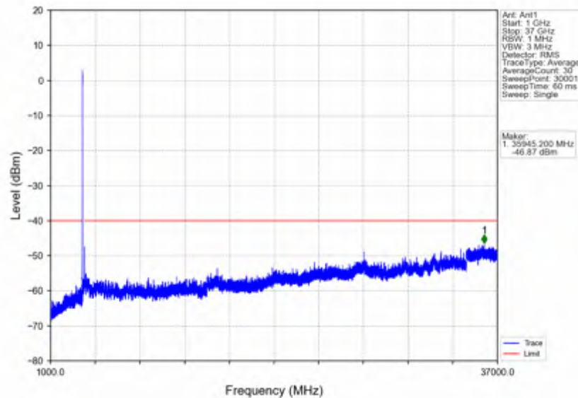
n78d_30kHz_SISO_NTNV_15MHz_CP-OFDM QPSK_3557.52MHz_Outer_Full
