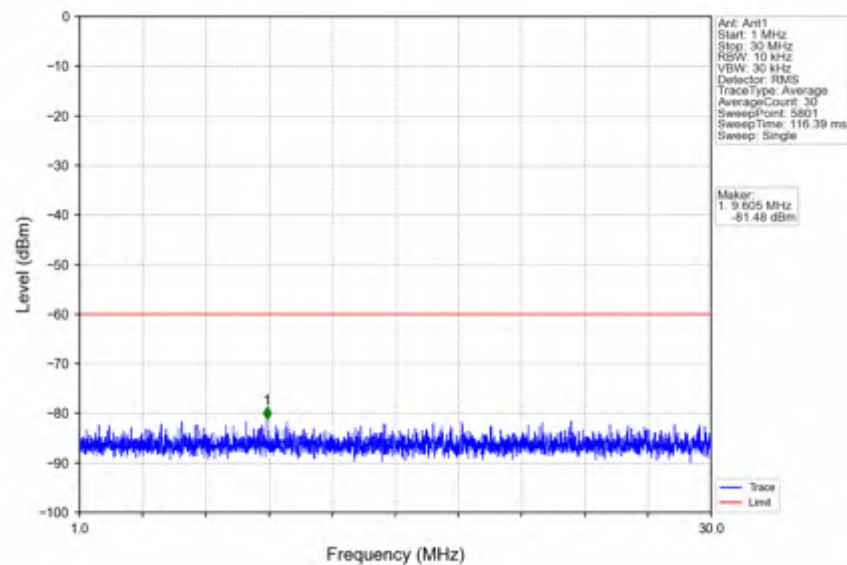
n78d_30kHz_SISO_NTNV_10MHz_CP-OFDM QPSK_3694.98MHz_Inner_1RB_Right
