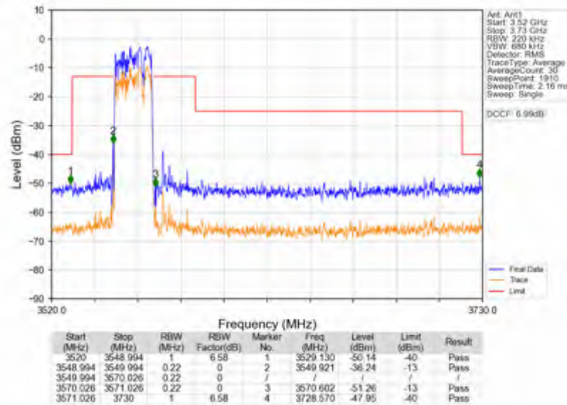
n78d_30kHz_SISO_NTNV_20MHz_DFT-s-OFDM_QPSK_3560.01MHz_Outer_Full
