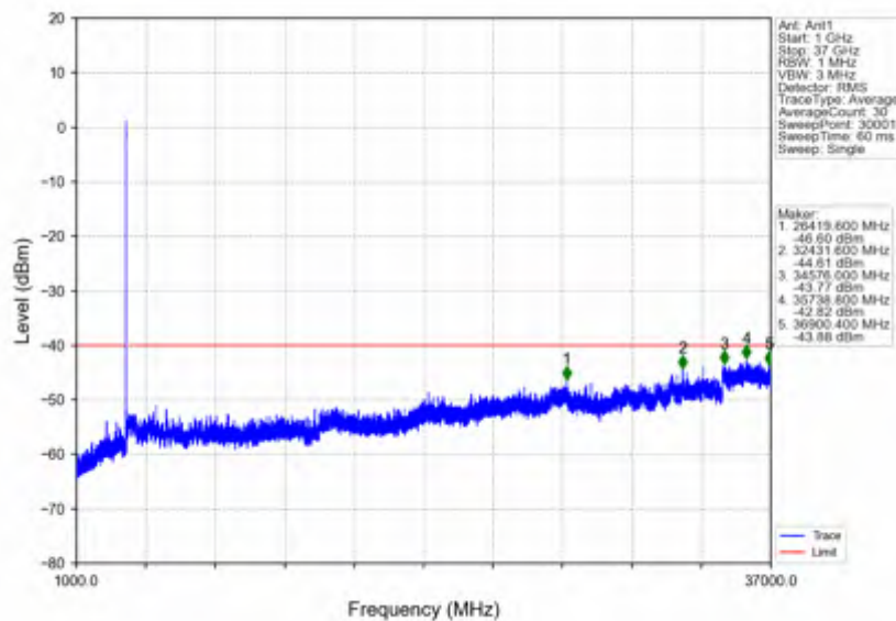
n78d_30kHz_SISO_NTNV_20MHz_DFT-s-OFDM_QPSK_3560.01MHz_Inner_1RB_Left
