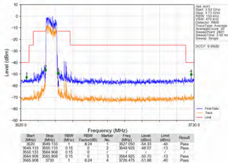
n78d_30kHz_SISO_NTNV_15MHz_DFT-s-OFDM_QPSK_3557.52MHz_Outer_Full
