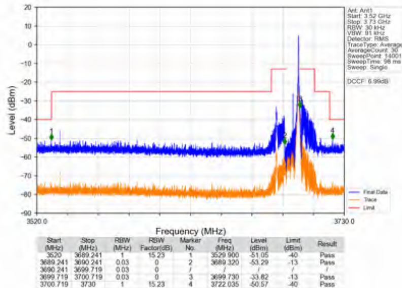
n78d_30kHz_SISO_NTNV_10MHz_CP-OFDM_QPSK_3694.98MHz_Inner_1RB_Right
