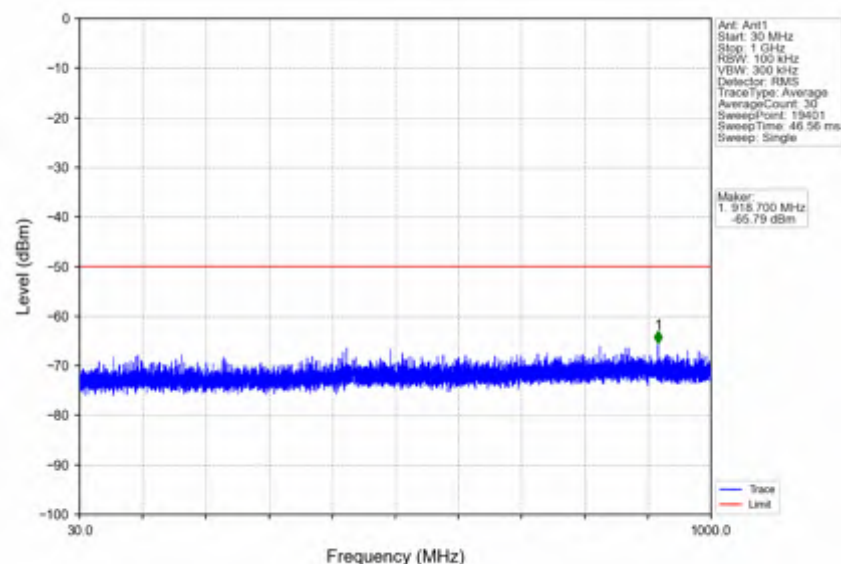
n78d_30kHz_SISO_NTNV_20MHz_DFT-s-OFDM_QPSK_3690MHz_Outer_Full
