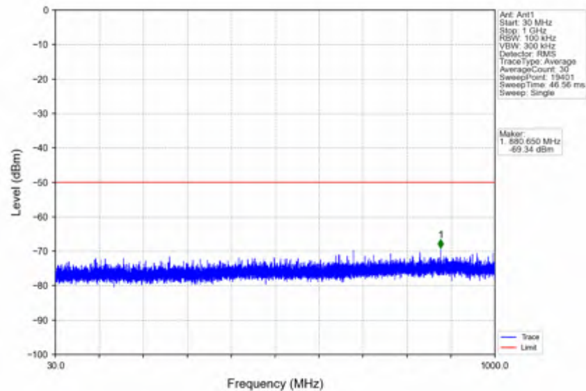
n78d_30kHz_SISO_NTNV_15MHz_CP-OFDM QPSK_3557.52MHz_Outer_Full
