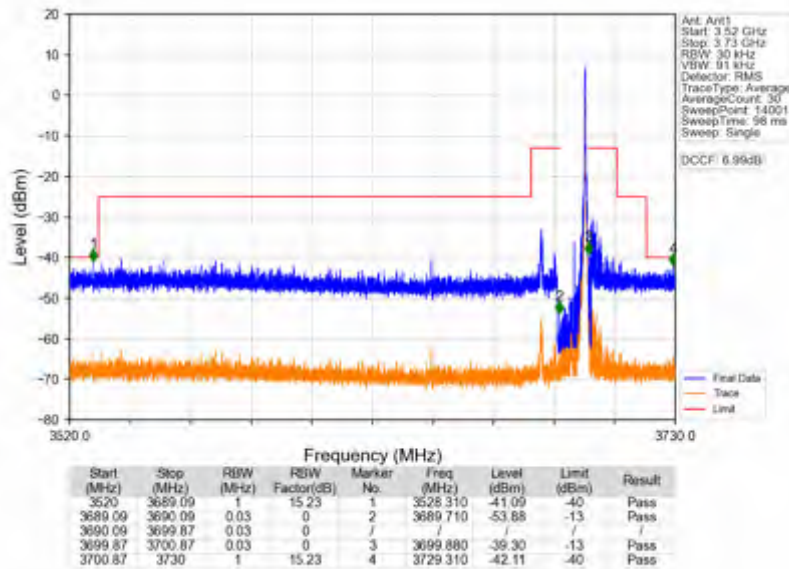
n78d_30kHz_SISO_NTNV_10MHz_DFT-s-OFDM QPSK_3694.98MHz_Inner_1RB_Right
