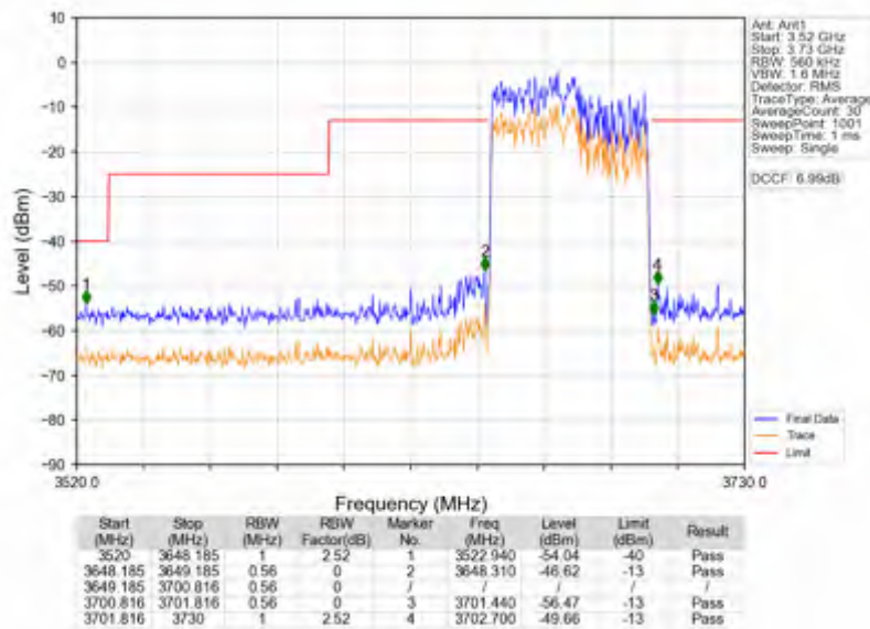
n78d_15kHz_SISO_NTNV_50MHz_CP-OFDM QPSK_3675MHz_Outer_Full
