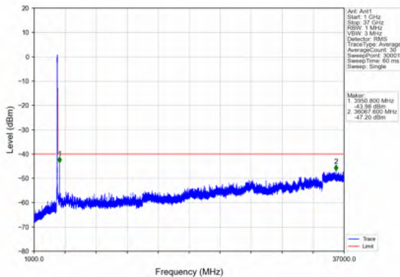
n78d 15kHz SISO NTN 50MHz CP-OFDM QPSK 3675MHz Outer Full
