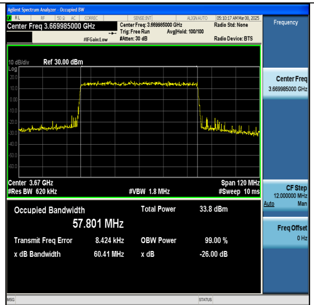
NTNV-n48-PC3-30-60-H-DFT-QPSK-Outer_Full-Ant1- PASS
