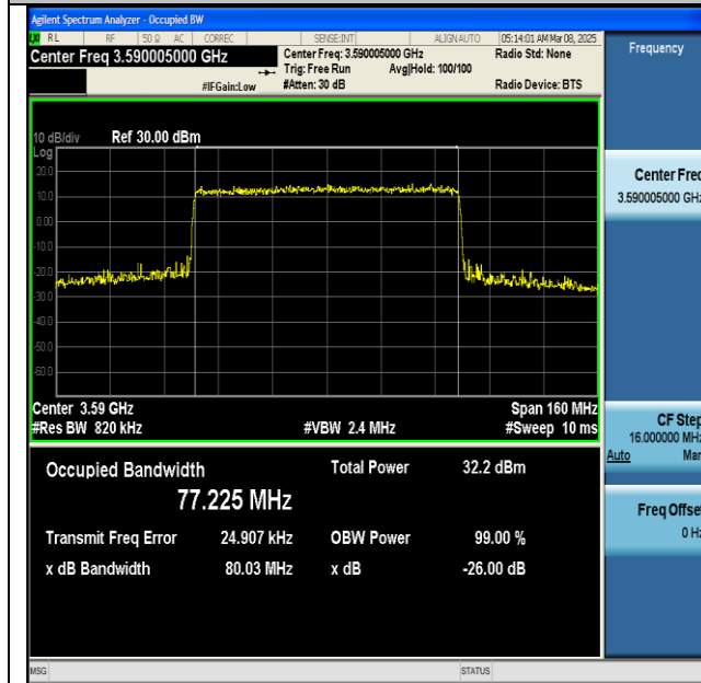
NTNV-n48-PC3-30-80-L-CP-QPSK-Outer_Full-Ant1-PASS
