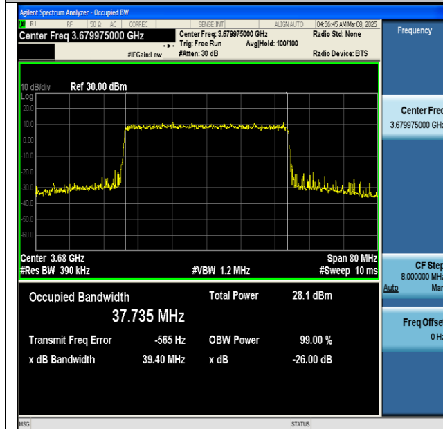
NTNV-n48-PC3-30-40-H-CP-256QAM-Outer_Full-Ant1- PASS
