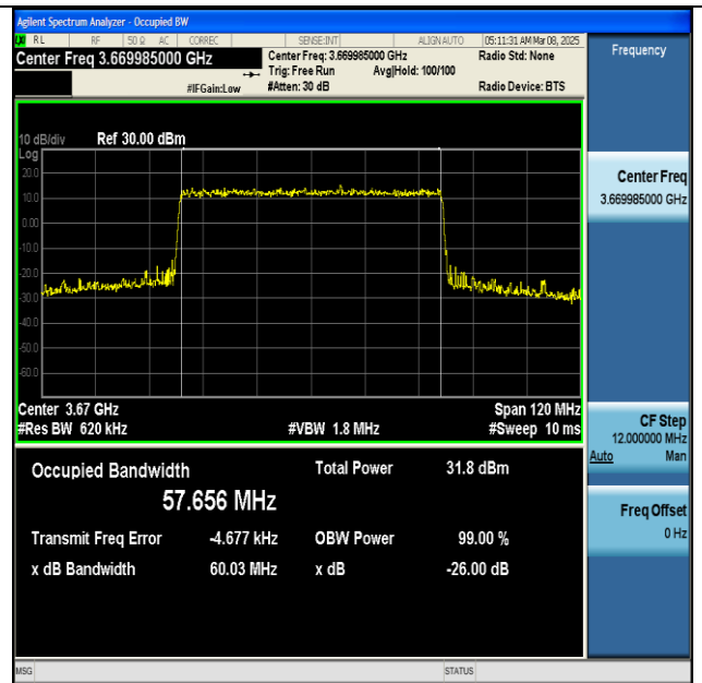
NTNV-n48-PC3-30-60-H-CP-QPSK-Outer_Full-Ant1-PASS
