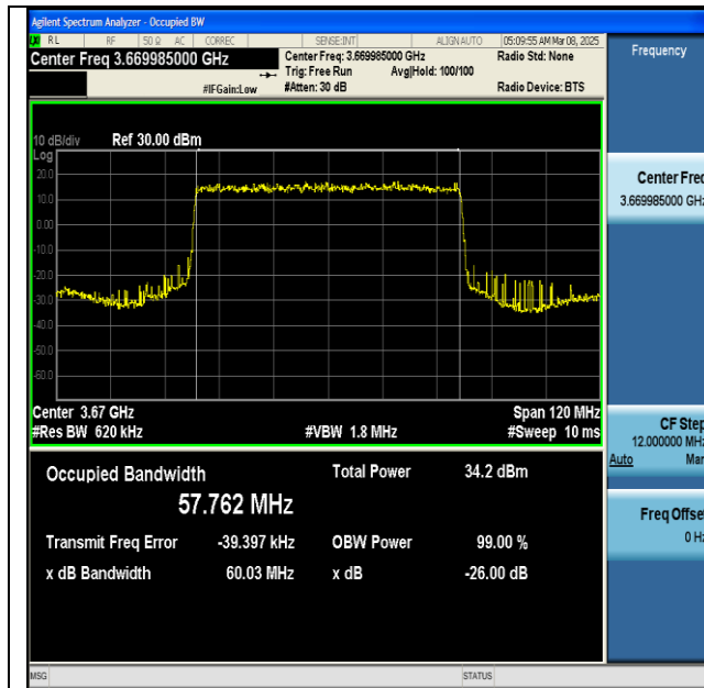
NTNV-n48-PC3-30-60-H-DFT-BPSK-Outer_Full-Ant1- PASS
