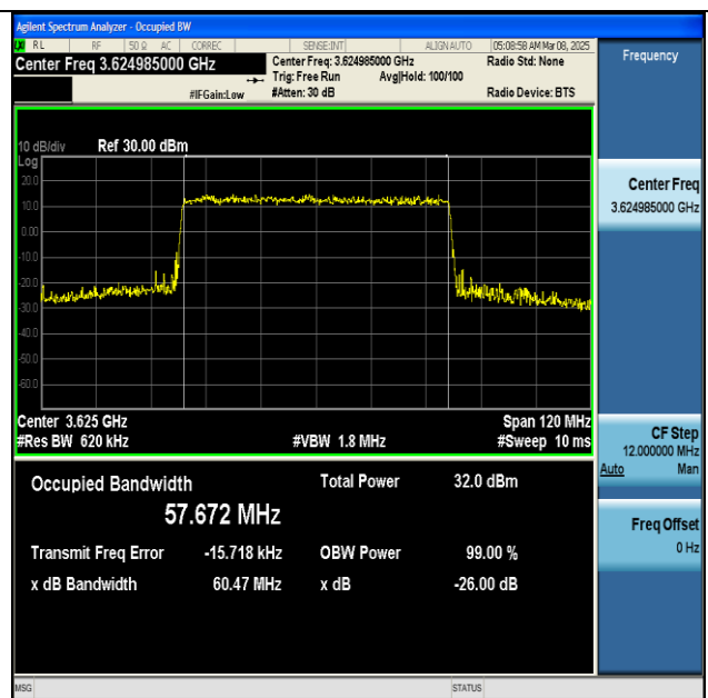
NTNV-n48-PC3-30-60-M-CP-16QAM-Outer_Full-Ant1- PASS
