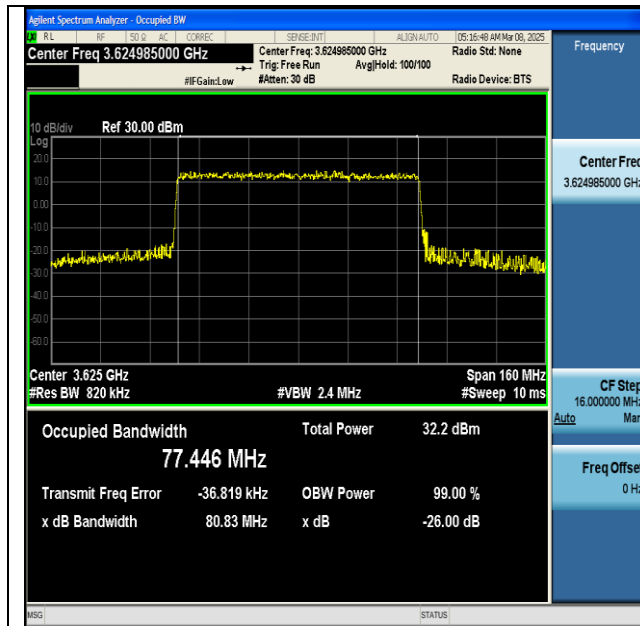
NTNV-n48-PC3-30-80-M-CP-16QAM-Outer_Full-Ant1- PASS
