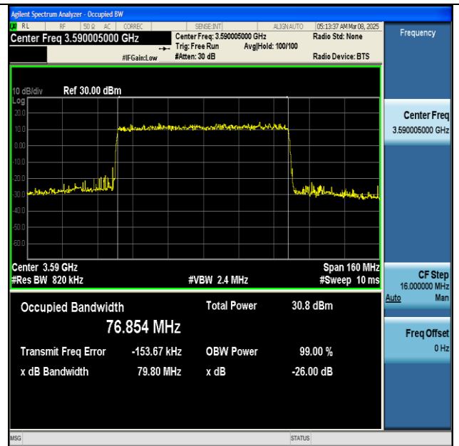
NTNV-n48-PC3-30-80-L-DFT-256QAM-Outer_Full-Ant1- PASS
