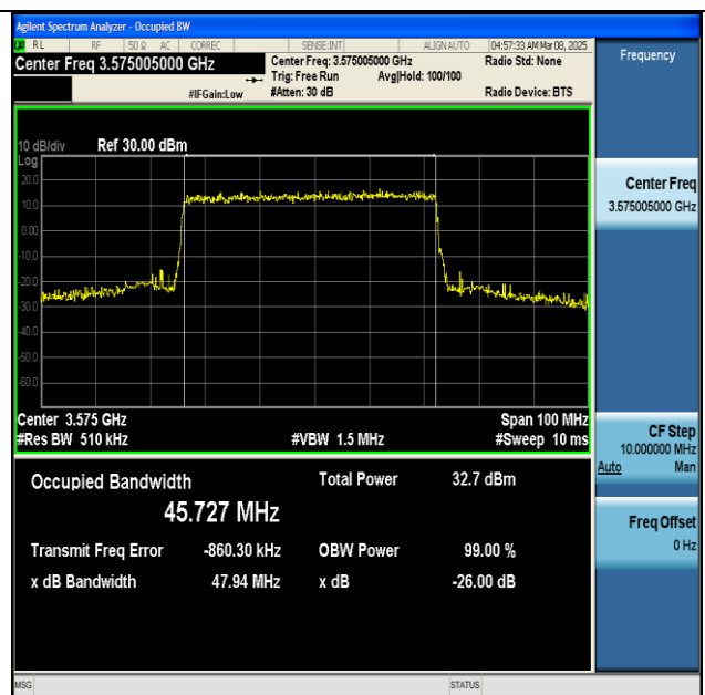
NTNV-n48-PC3-30-50-L-DFT-16QAM-Outer_Full-Ant1- PASS
