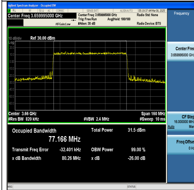
NTNV-n48-PC3-30-80-H-CP-64QAM-Outet_Full-Ant1-PASS
