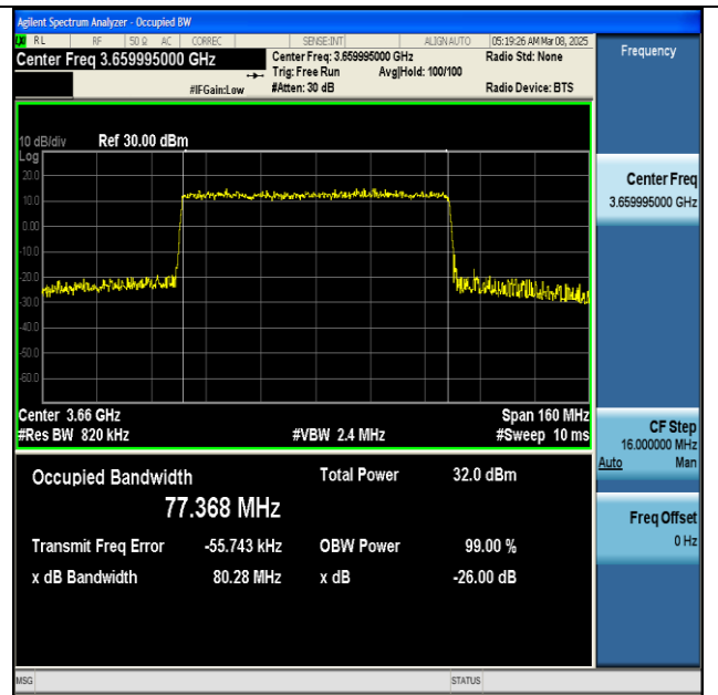
NTNV-n48-PC3-30-80-H-CP-16QAM-Outet_Full-Ant1-PASS
