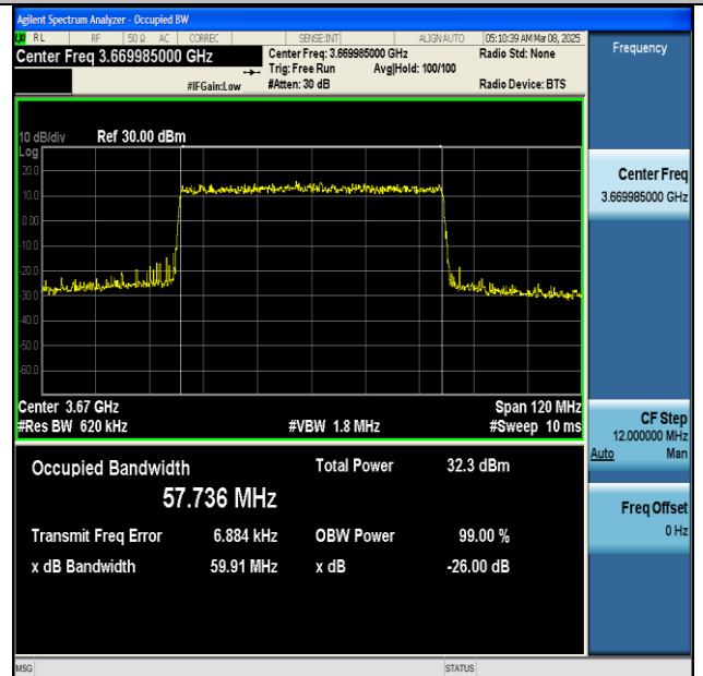
NTNV-n48-PC3-30-60-H-DFT-64QAM-Outer_Full-Ant1- PASS
