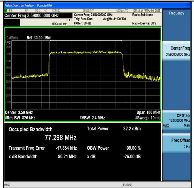
NTNV-n48-PC3-30-80-L-CP-16QAM-Outer_Full-Ant1- PASS
