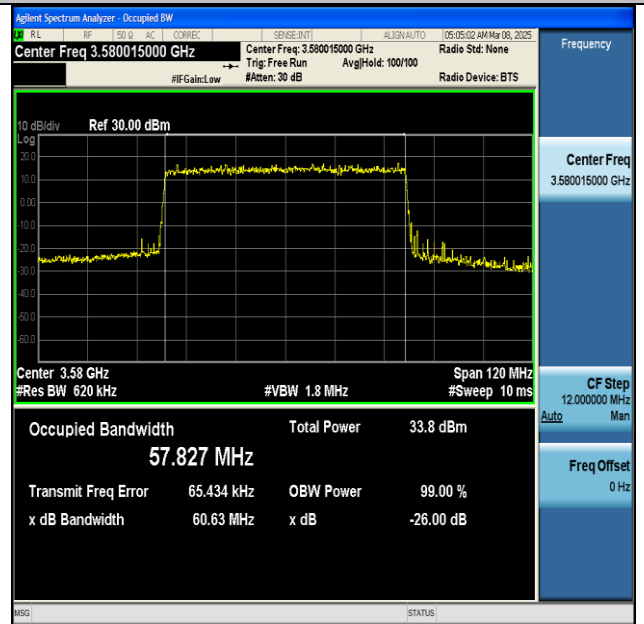
NTNV-n48-PC3-30-60-L-DFT-QPSK-Outer_Full-Ant1- PASS
