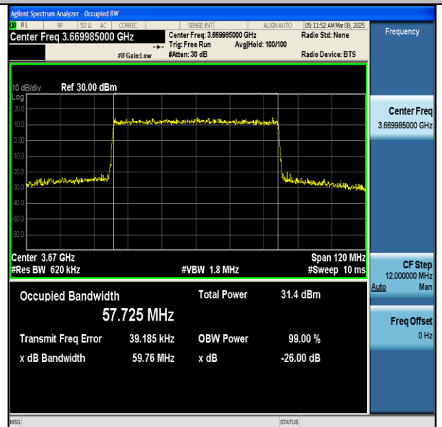
NTNV-n48-PC3-30-60-H-CP-64QAM-Outer_Full-Ant1-PASS
