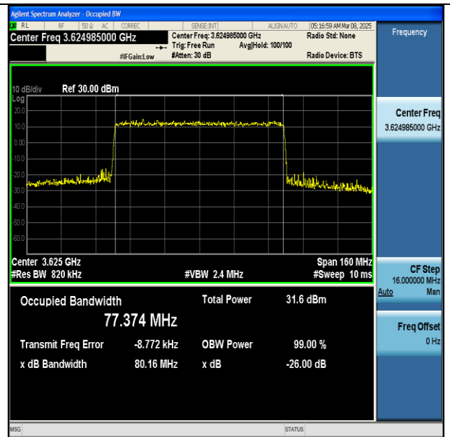
NTNV-n48-PC3-30-80-M-CP-64QAM-Outer_Full-Ant1- PASS
