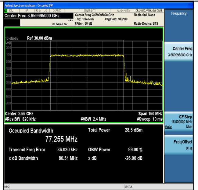
NTNV-n48-PC3-30-80-H-CP-256QAM-Outet_Full-Ant1-PASS
