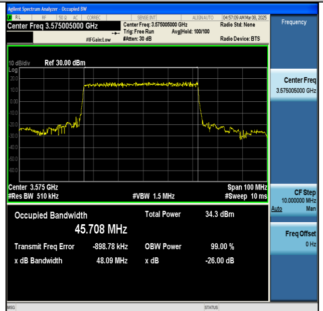
NTNV-n48-PC3-30-50-L-DFT-BPSK-Outer_Full-Ant1- PASS
