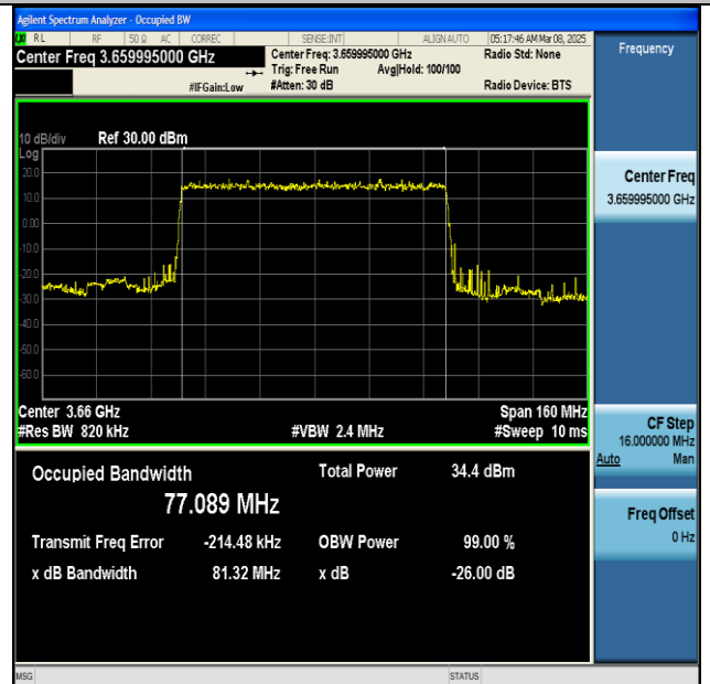
NTNV-n48-PC3-30-80-H-DFT-BPSK-Outer_Full-Ant1- PASS
