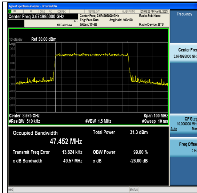
NTNV-n48-PC3-30-50-H-CP-64QAM-Outer_Full-Ant1- PASS
