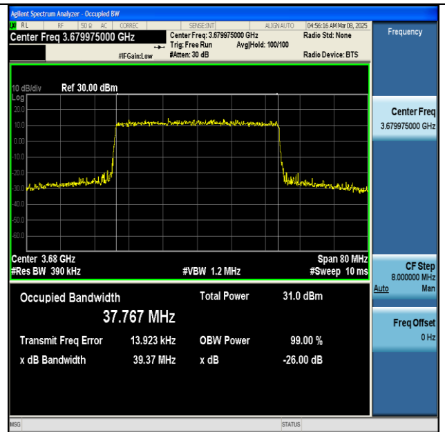
NTNV-n48-PC3-30-40-H-CP-64QAM-Outer_Full-Ant1- PASS
