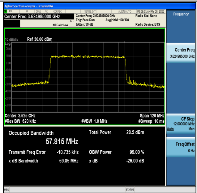
NTNV-n48-PC3-30-60-M-CP-256QAM-Outer_Full-Ant1- PASS
