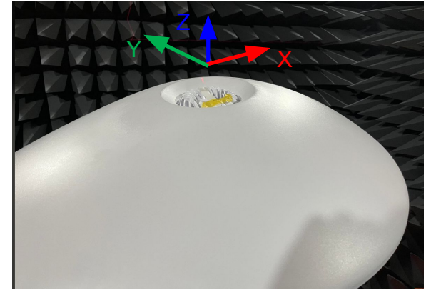
1. Antenna type: printed PCB
