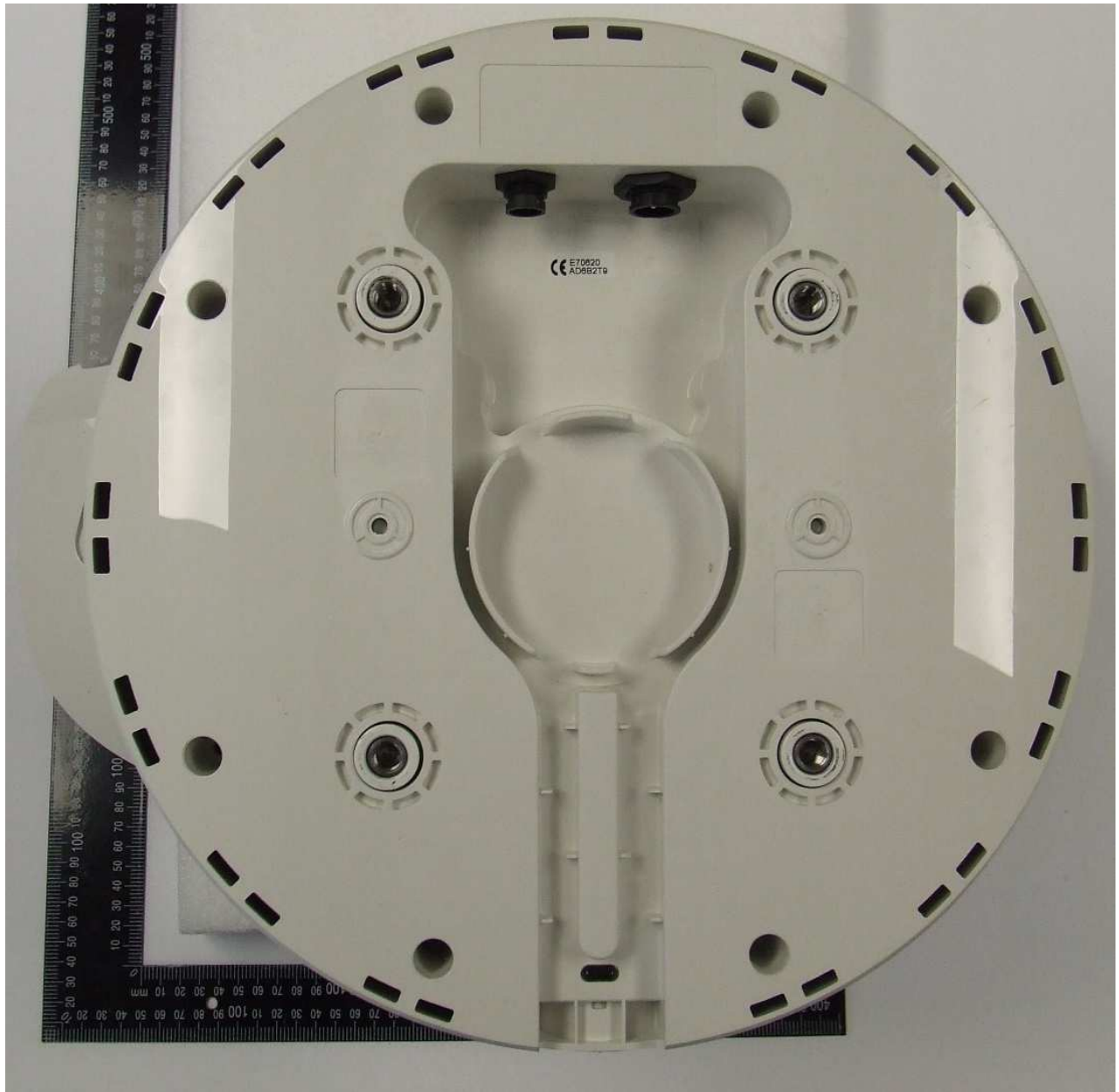
Figure 8 – Pedestal (bottom)
