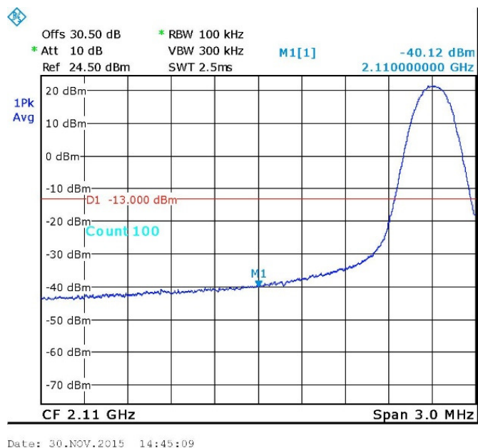
Figure 104. — GSM 2111.2 MHz
