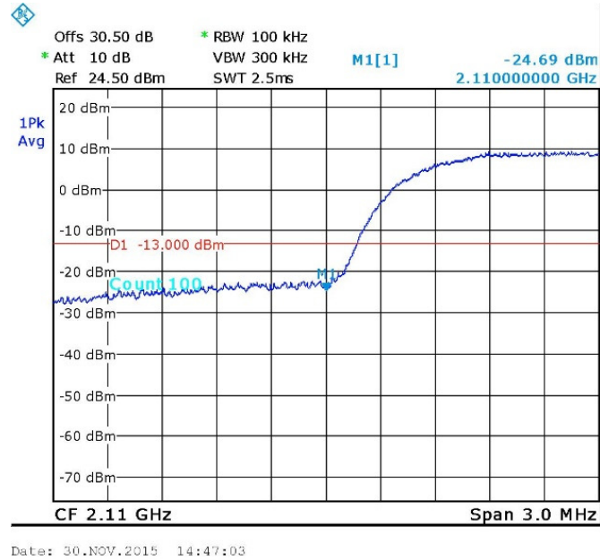
Figure 106. — WCDMA 2112.5 MHz
