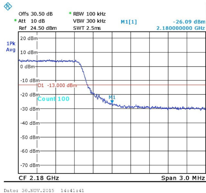
Figure 103. — LTE 64QAM 2175.0 MHz
