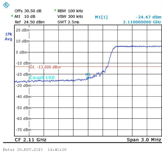
Figure 102. — LTE 64QAM 2115.0 MHz
