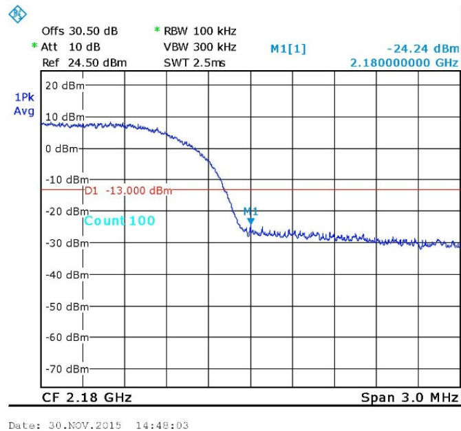
Figure 107. — WCDMA 2177.5 MHz
