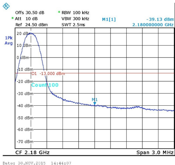
Figure 105. — GSM 2178.8 MHz
