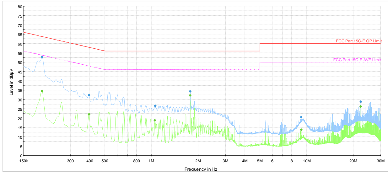
Plot 7-62. AC Line Conducted Plot with 802.11n– Ch.157 (N) with host PC & magnetic charger
