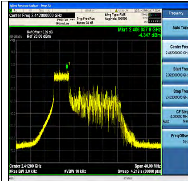
11be20MIMO-Ant1-2412-52Tone-RU37-PASS
