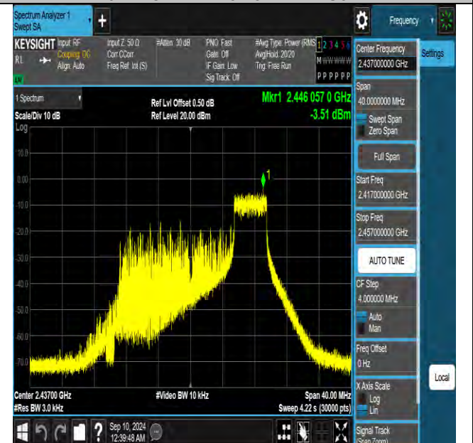
11be20MIMO-Ant2-2437-52Tone-RU40-PASS
