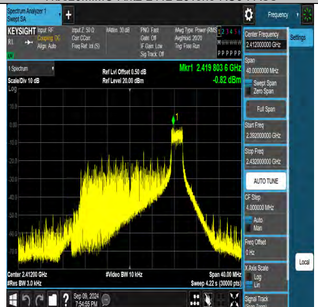
11be20MIMO-Ant2-2412-26Tone-RU8-PASS
