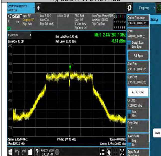
11g-CDD-Ant1-2437-PASS
