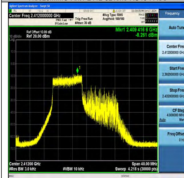
11be20MIMO-Ant2-2412-106Tone-RU53-PASS
