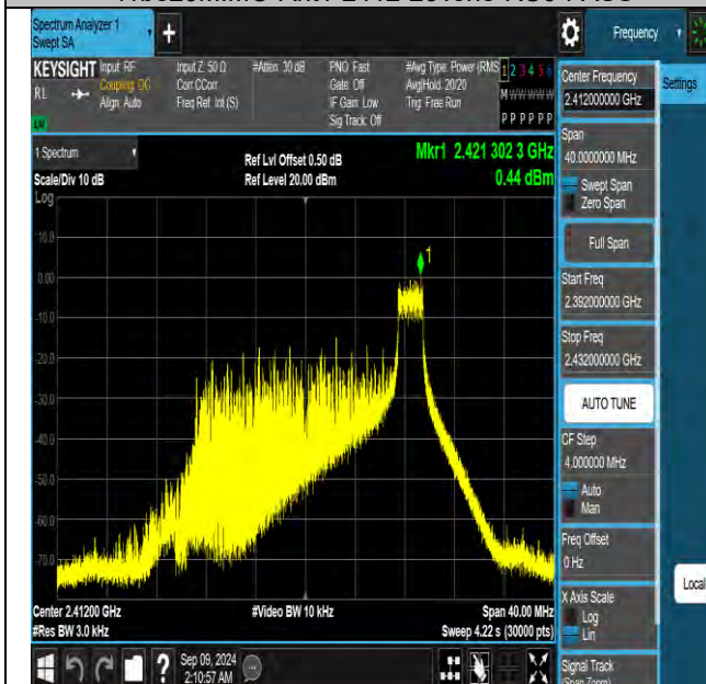
11be20MIMO-Ant1-2412-26Tone-RU8-PASS
