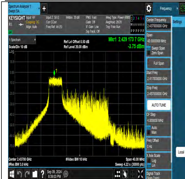
11be20MIMO-Ant1-2437-52Tone-RU37-PASS
