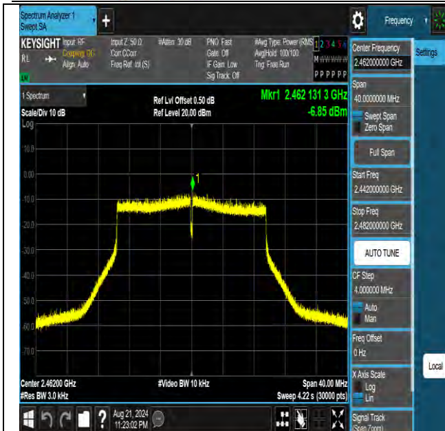
11ax20MIMO-Ant1-2462-PASS
