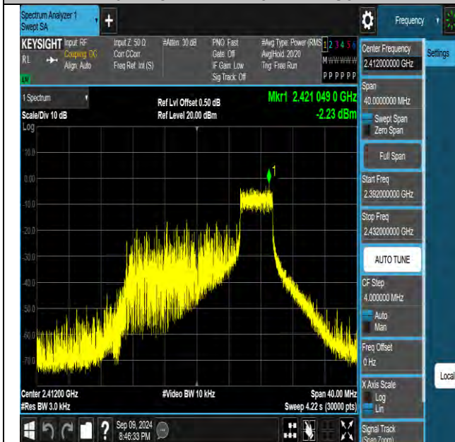
11be20MIMO-Ant1-2412-52Tone-RU40-PASS
