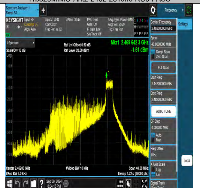
11be20MIMO-Ant2-2462-26Tone-RU8-PASS
