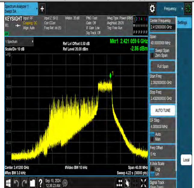
11be20MIMO-Ant2-2412-52Tone-RU40-PASS
