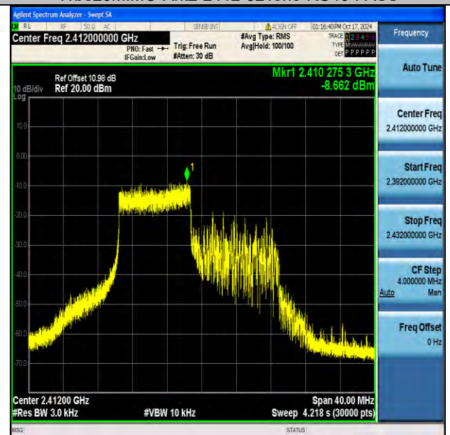
11be20MIMO-Ant1-2412-106Tone-RU53-PASS
