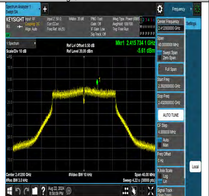
11n20MIMO-Ant2-2412-PASS
