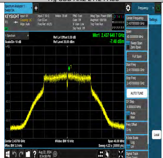
11g-CDD-Ant2-2437-PASS
