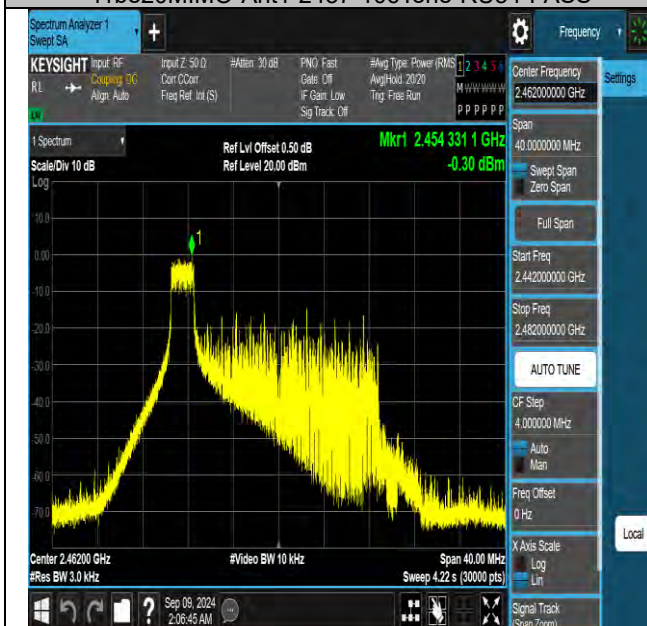
11be20MIMO-Ant1-2462-26Tone-RU0-PASS
