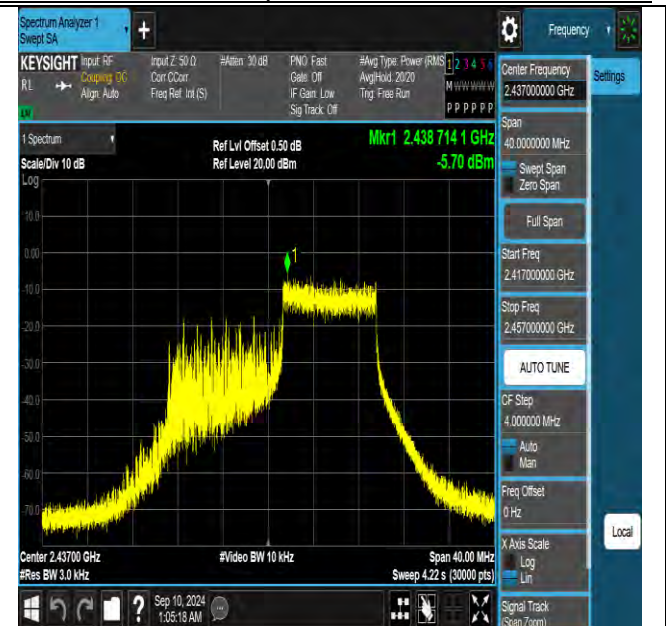
11be20MIMO-Ant2-2437-106Tone-RU54-PASS
