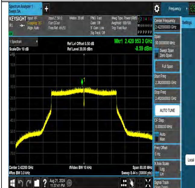
11ax40MIMO-Ant1-2422-PASS
