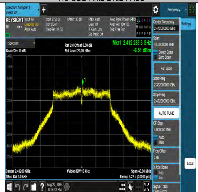
11g-CDD-Ant2-2412-PASS
