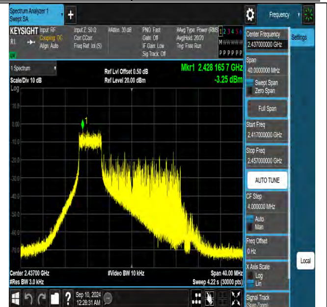
11be20MIMO-Ant2-2437-52Tone-RU37-PASS
