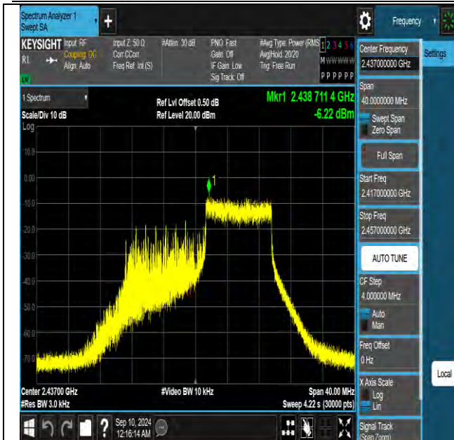
11be20MIMO-Ant1-2437-106Tone-RU54-PASS
