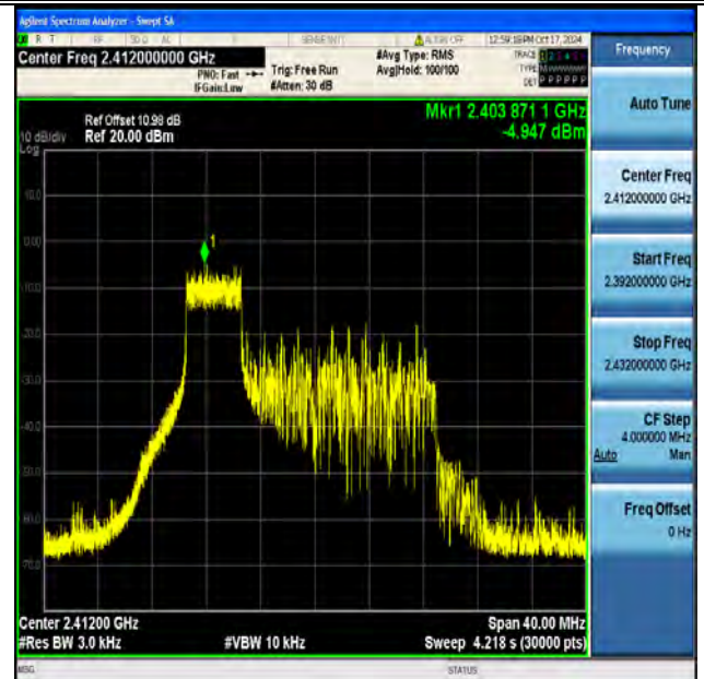
11be20MIMO-Ant2-2412-52Tone-RU37-PASS
