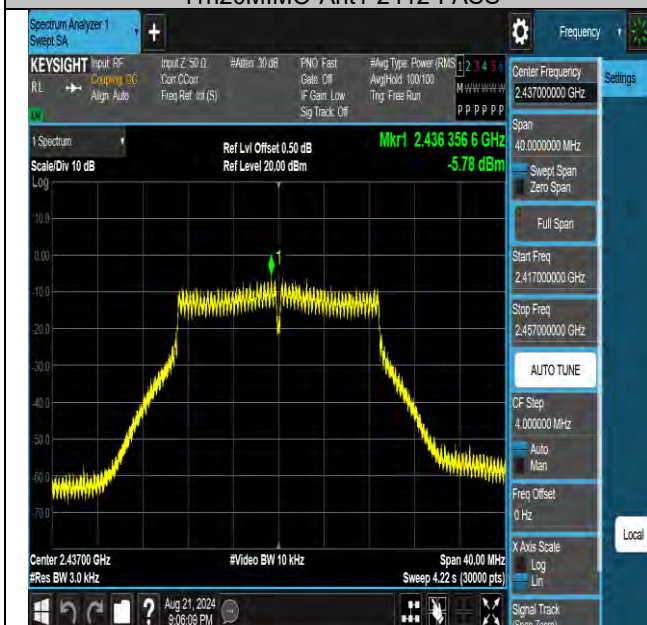
11n20MIMO-Ant1-2437-PASS
