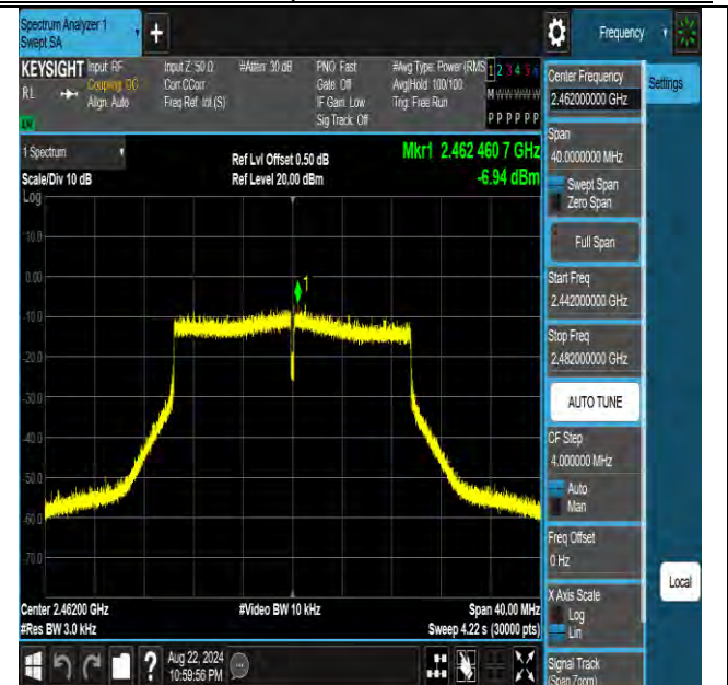
11ax20MIMO-Ant2-2462-PASS
