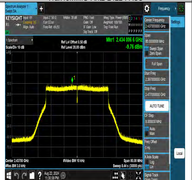
11ax40MIMO-Ant2-2437-PASS
