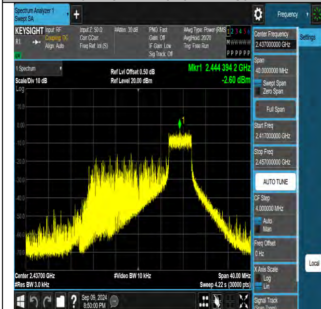
11be20MIMO-Ant1-2437-52Tone-RU40-PASS
