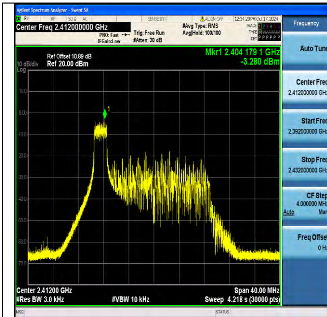
11be20MIMO-Ant1-2412-26Tone-RU0-PASS
