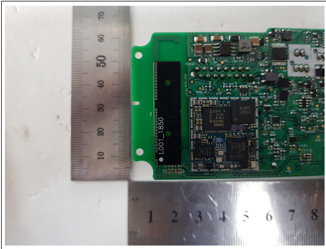
<LTE Main Tx Antenna>
