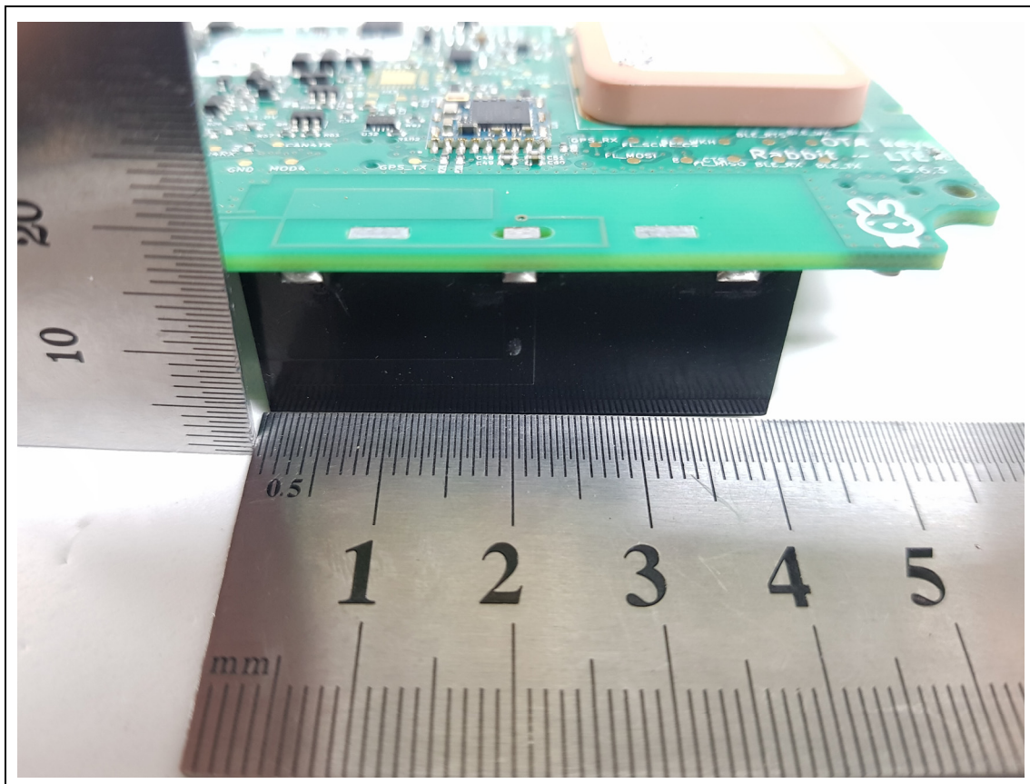
<LTE Rx diversity Antenna>
