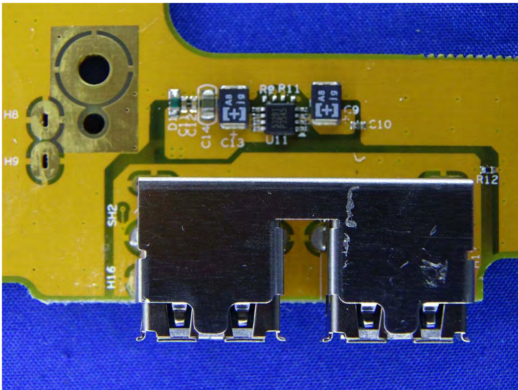
(90) EUT Photo
