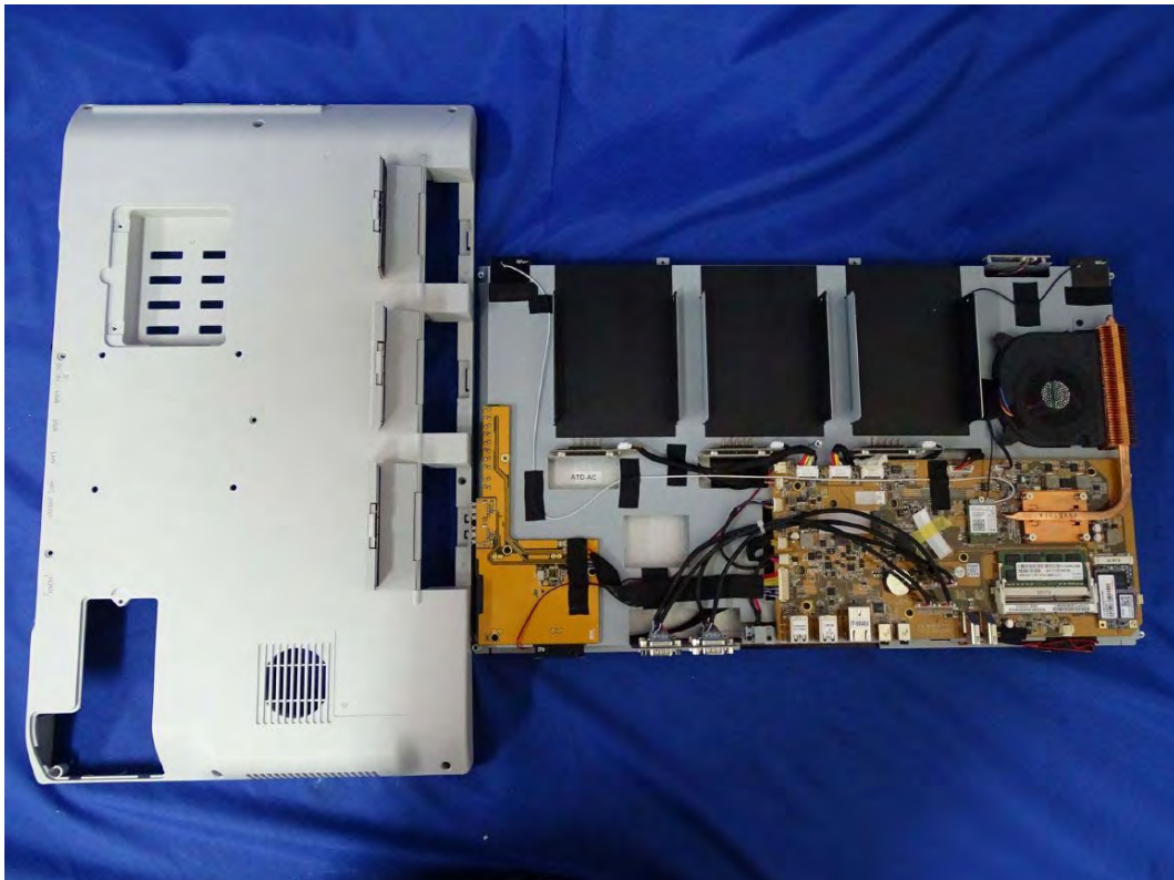
(80) EUT Photo
