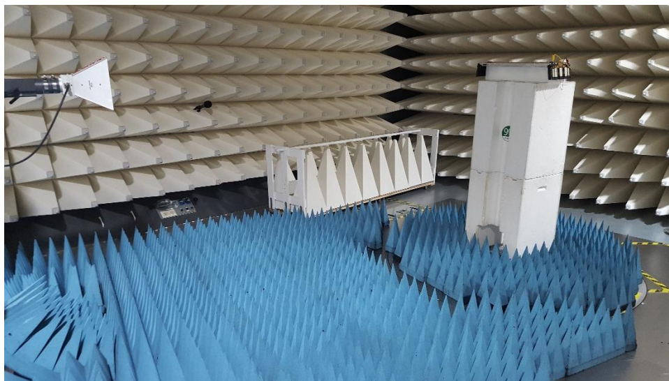
Figure B3. Radiated emission Setup – High Range for DUT
