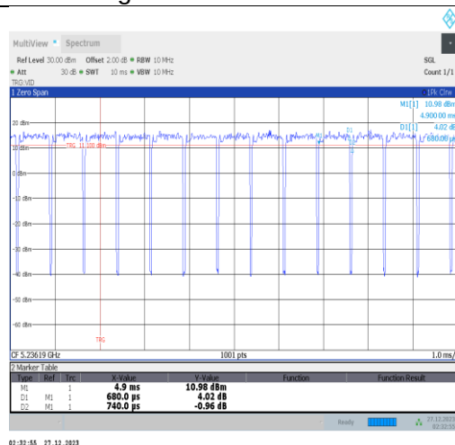
NTNV-11ax40MIMO-Ant2-5230-242Tone-RU62
