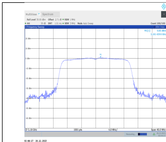
11ax20MIMO-Ant3-5180-PASS
