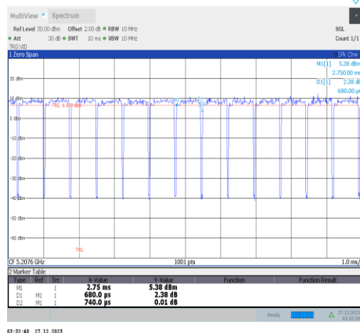
NTNV-11ax80MIMO-Ant1-5210-484Tone-RU65
