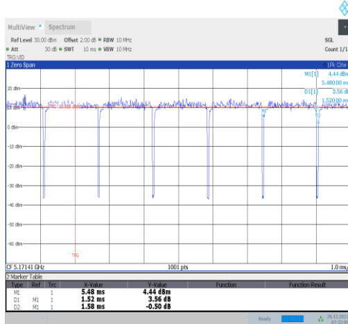
NTNV-11ax20MIMO-Ant3-5180-26Tone-RU0
