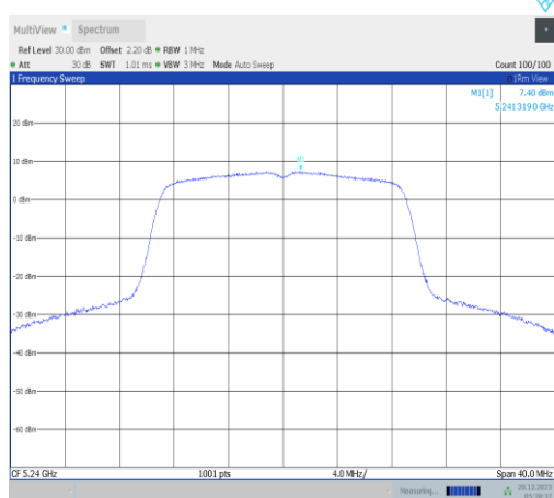
11n20SISO-Ant3-5240-PASS
