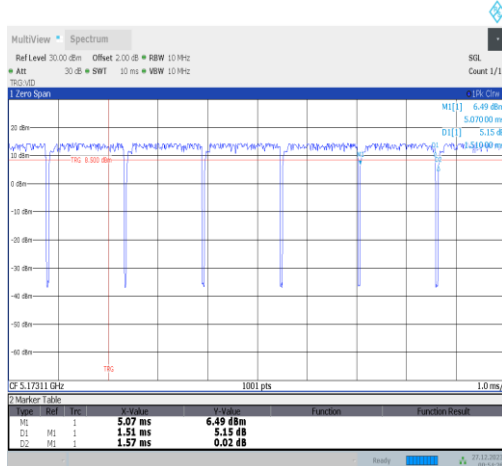
NTNV-11ax20MIMO-Ant4-5180-52Tone-RU37
