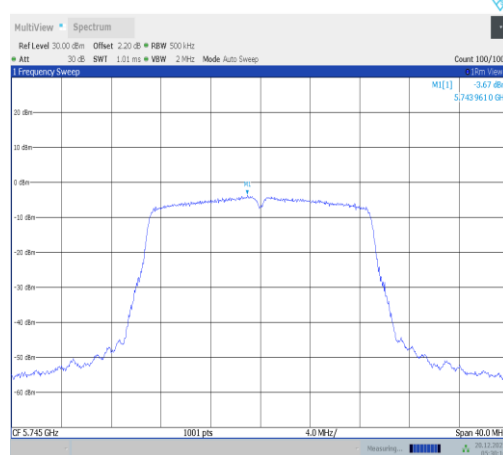
11n20SISO-Ant3-5745-PASS
