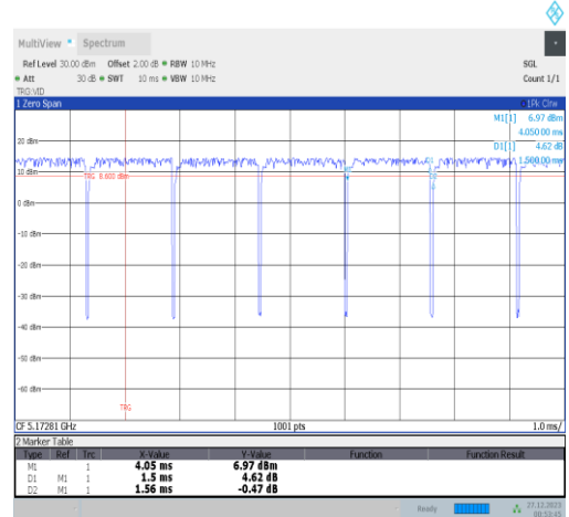
NTNV-11ax20MIMO-Ant3-5180-52Tone-RU37
