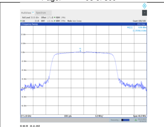
11ax20MIMO-Ant4-5180-PASS
