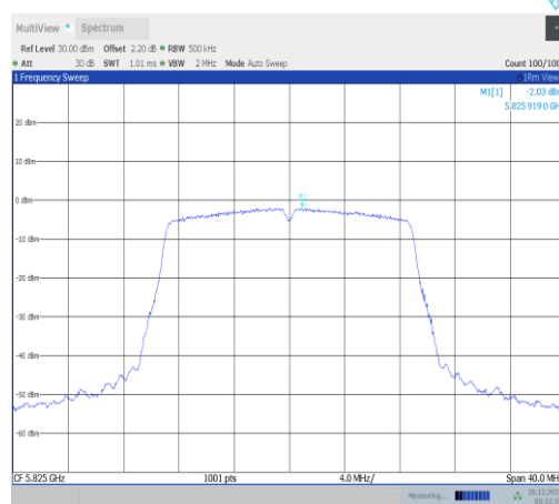
11n20SISO-Ant3-5825-PASS
