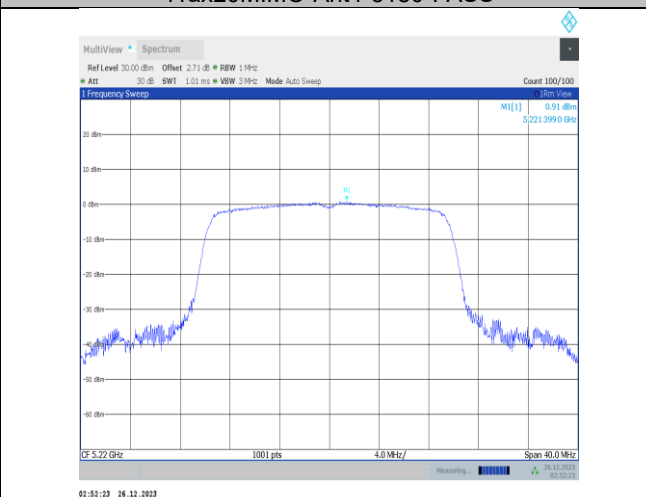
11ax20MIMO-Ant2-5220-PASS
