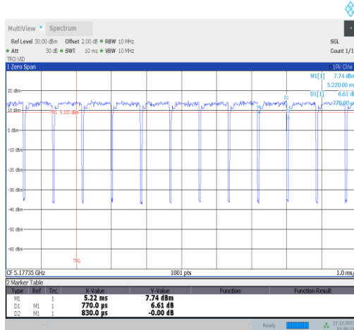
NTNV-11ax20MIMO-Ant3-5180-106Tone-RU53
