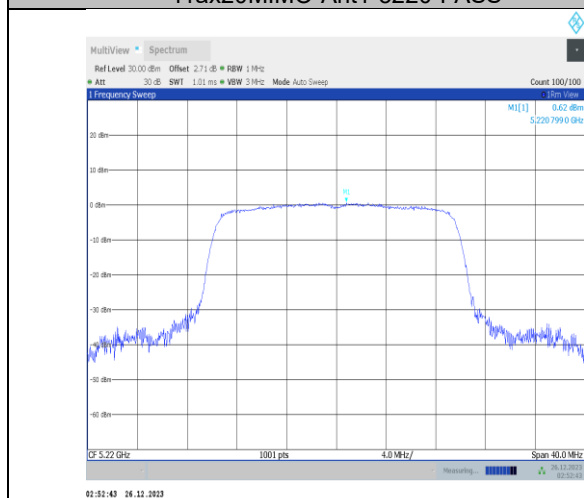
11ax20MIMO-Ant3-5220-PASS
