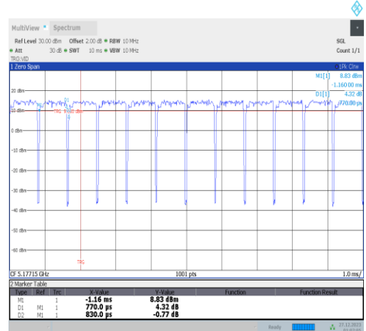
NTNV-11ax20MIMO-Ant4-5180-106Tone-RU53
