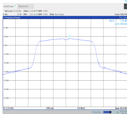
11n20SISO-Ant3-5220-PASS
