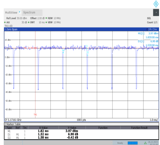
NTNV-11ax20MIMO-Ant4-5180-26Tone-RU0
