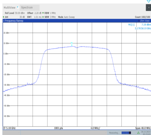
11n20SISO-Ant3-5180-PASS
