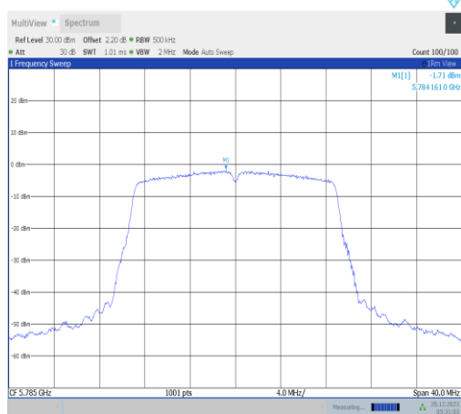
11n20SISO-Ant3-5785-PASS
