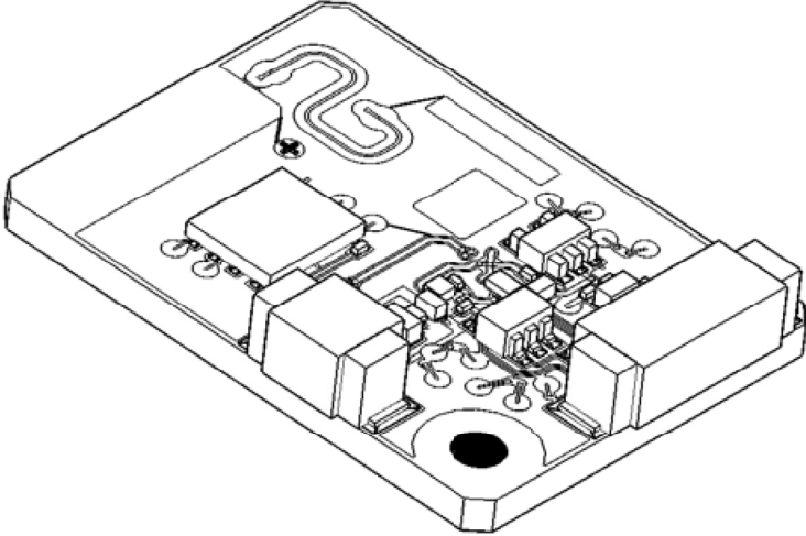
Top – without shielding
