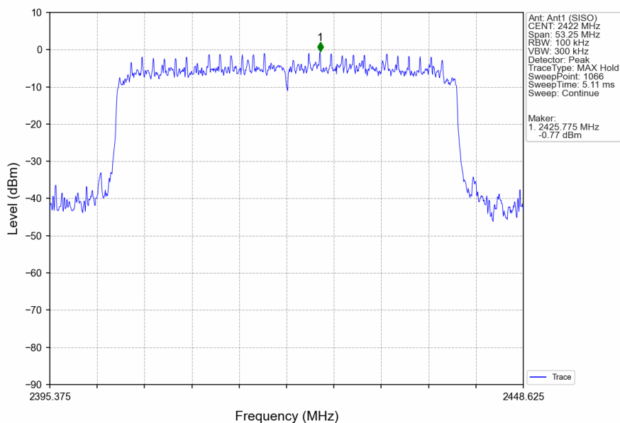
802.11ax(HEW40)_LCH_2422MHz_SU_/_Ant1 (SISO)_NTNV
