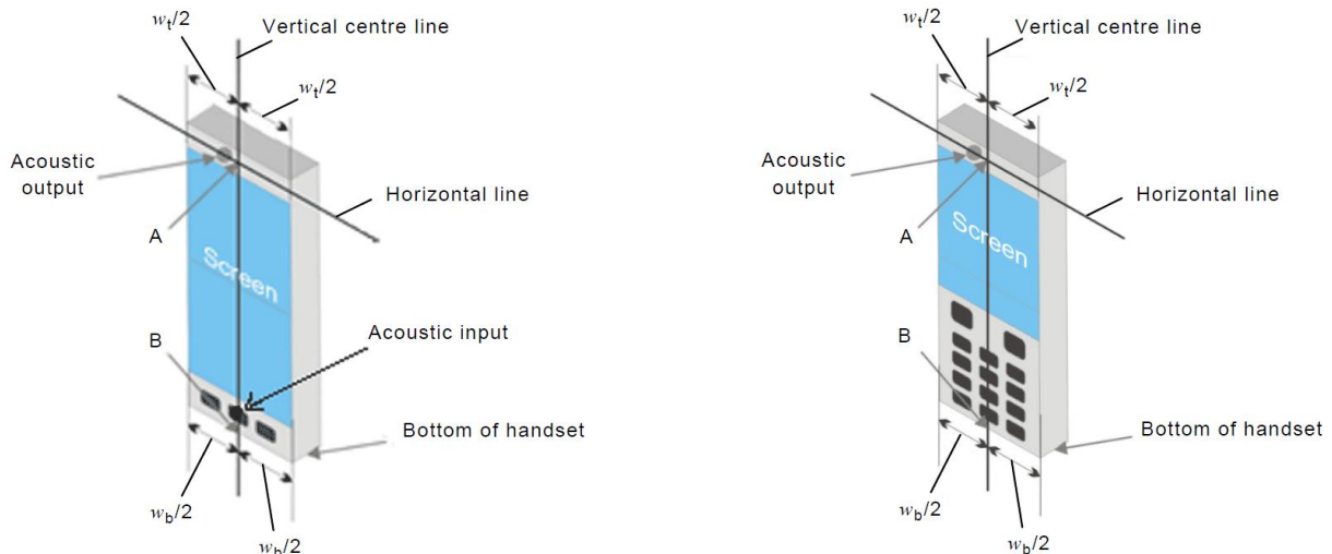
Fig-4.1 Illustration for Handset Vertical and Horizontal Reference Lines
