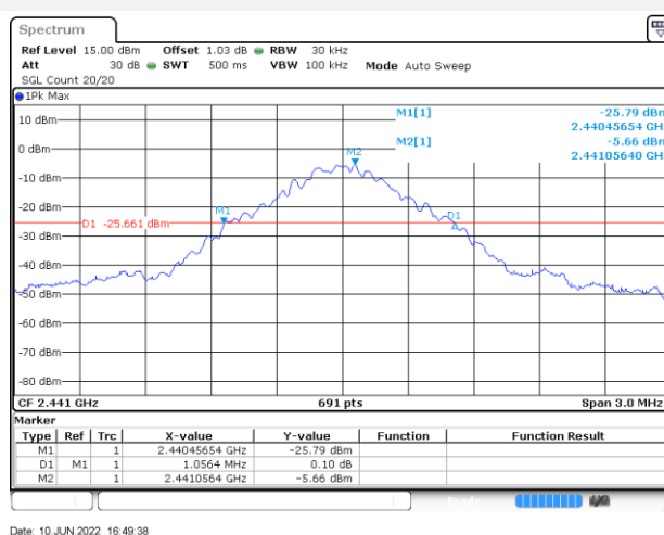
GFSK MIDDLE CHANNEL
