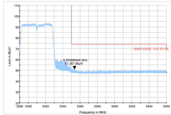
802.11ac HT40-Channel 62: Average
