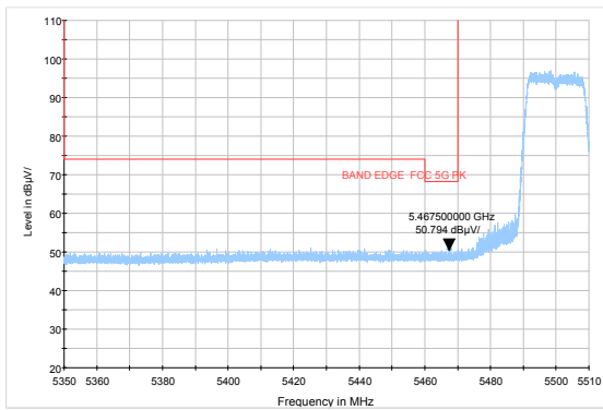
802.11ac HT20-Channel 100: Average
