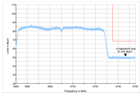
802.11ac HT80 –Channel 138: Peak
