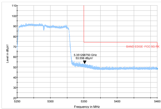
802.11ac HT80 -Channel 58: Peak
