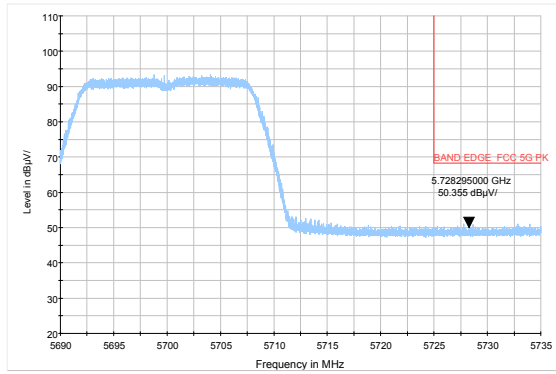
802.11a-Channel 140: Peak
