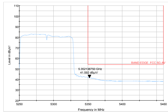
802.11ac HT80- Channel 58: Average
