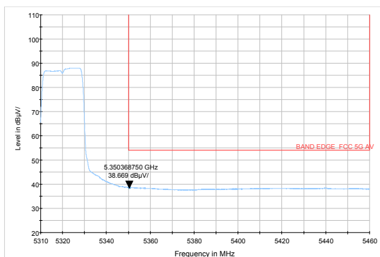
802.11ac HT20 -Channel 64: Average
