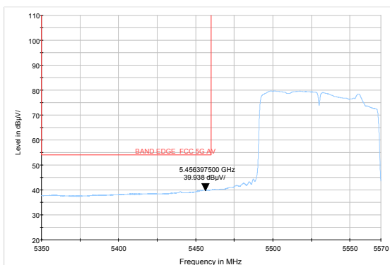
802.11ac HT80- Channel 106: Average
