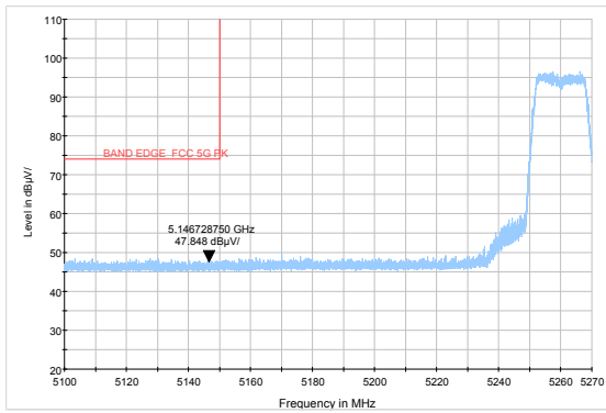
802.11a-Channel 52: Average
