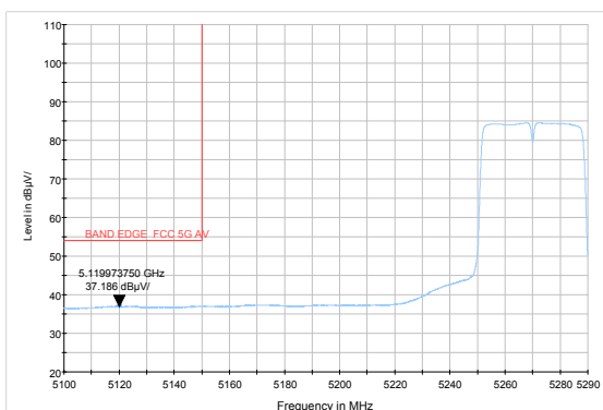
802.11ac HT20 -Channel 52: Peak
