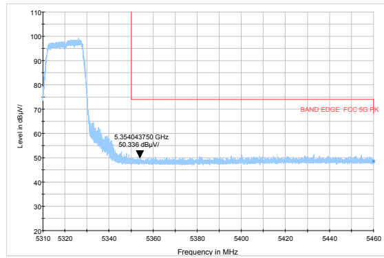
802.11a-Channel 64: Average
