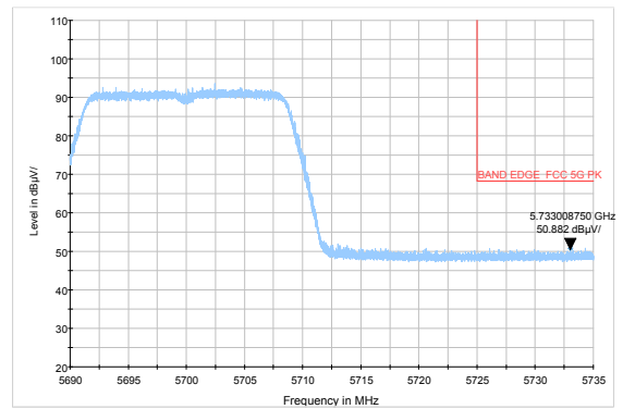
802.11ac HT20 -Channel 140: Peak
