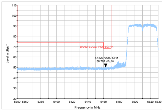
802.11ac HT40-Channel 102: Average
