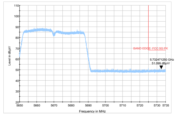
802.11ac HT40-Channel 134: Peak
