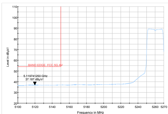
802.11ac HT20-Channel 52: Average
