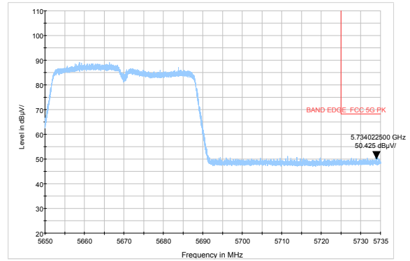
802.11n HT40-Channel 134: Peak
