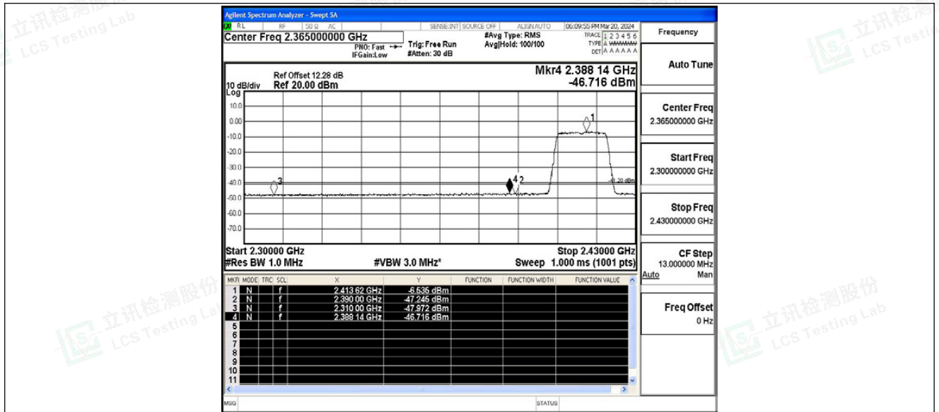
11G_Ant1_Low_2412_Peak
