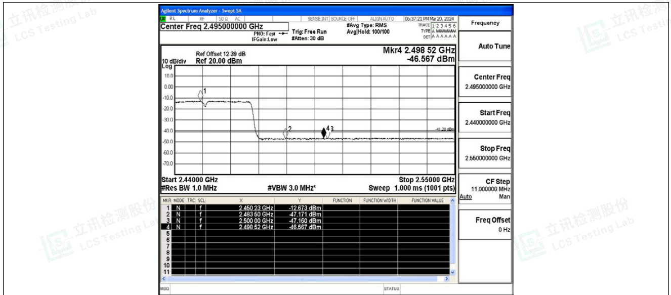
11N40SISO_Ant1_High_2452_Peak
