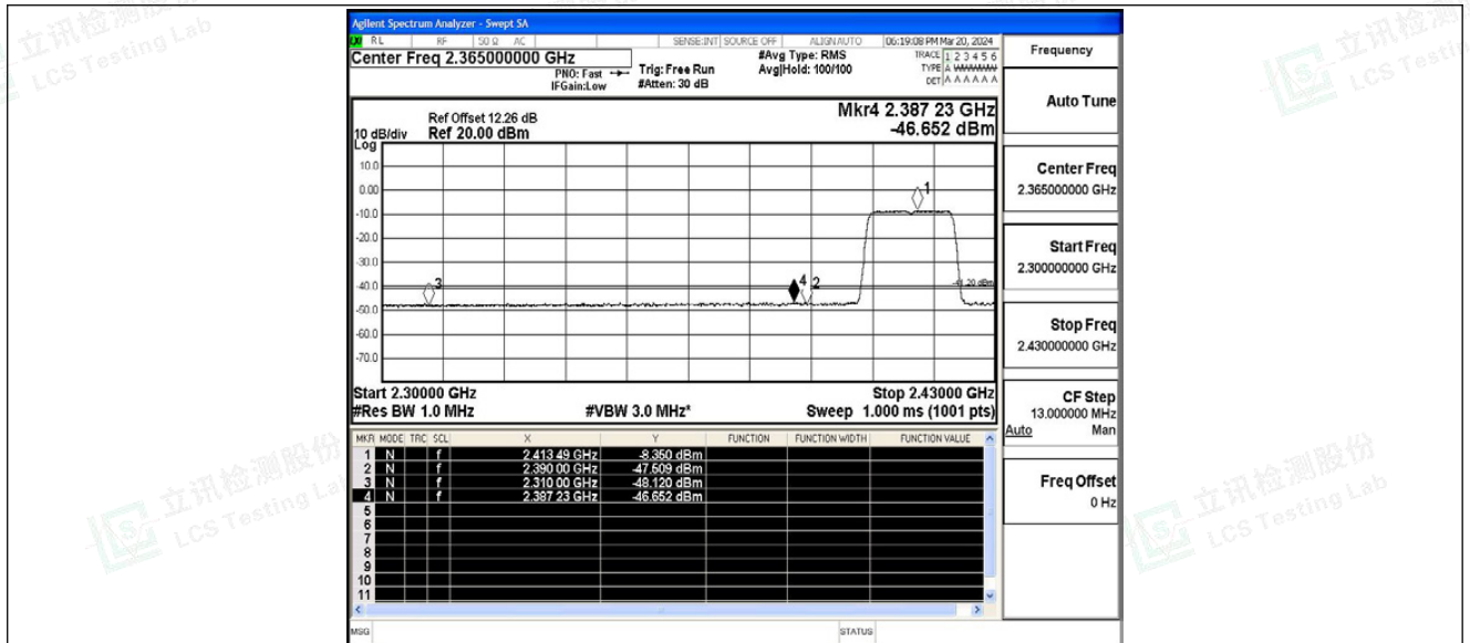
11N20SISO_Ant1_Low_2412_Peak
