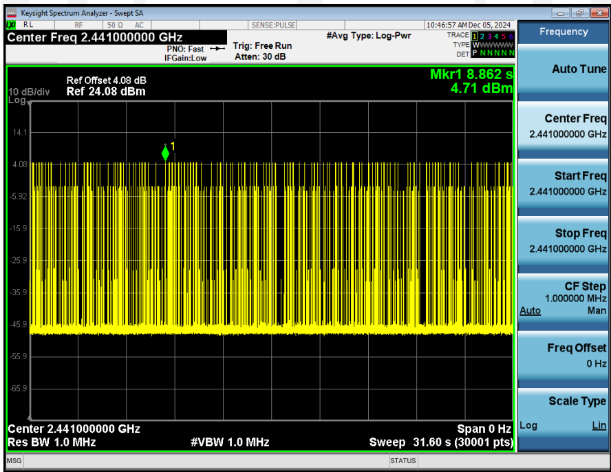
Dwell_Time_(Hopping)_NVNT_ANT1_1-DH3_2441_00_Accumulated
