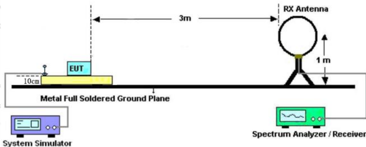
Figure 1. Below 30MHz
