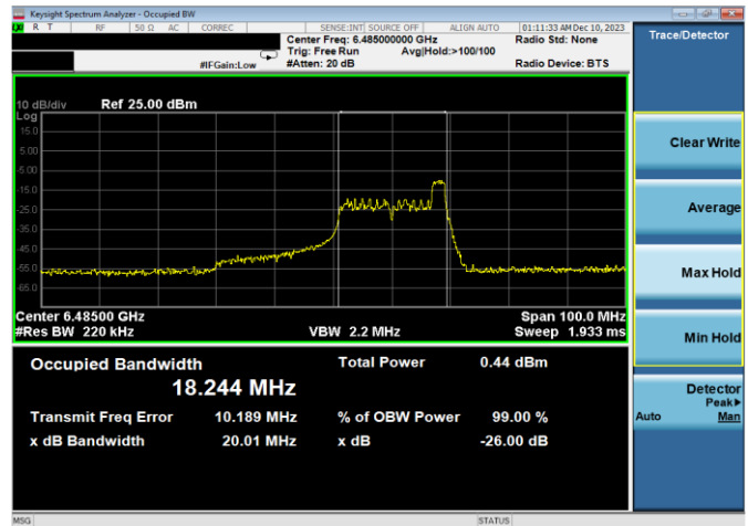
Plot 7-23. 26dB & 99% Bandwidth Plot Antenna WF8 (40MHz 802.11ax RU26 (UNII Band 6) – Ch. 107)
