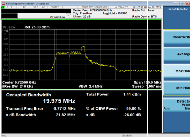
Plot 7-38. 26dB & 99% Bandwidth Plot Antenna WF8 (40MHz 802.11ax RU26 (UNII Band 7) – Ch. 155)
