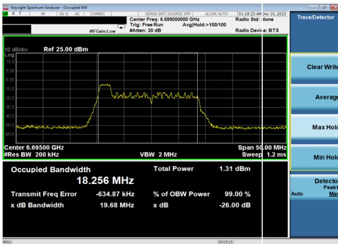
Plot 7-33. 26dB & 99% Bandwidth Plot Antenna WF8 (20MHz 802.11ax RU26 (UNII Band 7) – Ch. 149)
