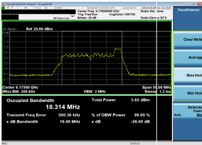
Plot 7-67. 26dB & 99% Bandwidth Plot Antenna WF7a (20MHz 802.11ax RU26 (UNII Band 5) – Ch. 45)
