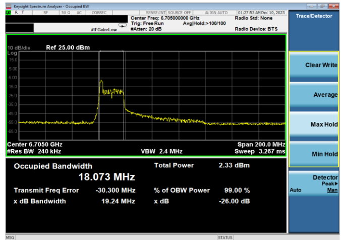
Plot 7-41. 26dB & 99% Bandwidth Plot Antenna WF8 (80MHz 802.11ax RU26 (UNII Band 7) – Ch. 151)
