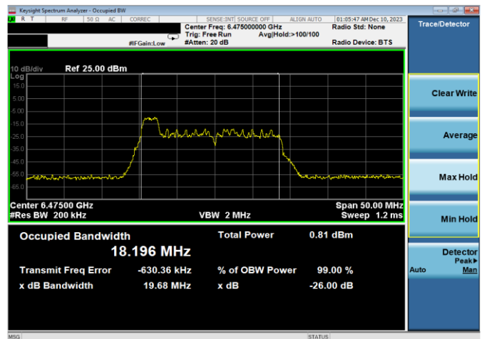
Plot 7-17. 26dB & 99% Bandwidth Plot Antenna WF8 (20MHz 802.11ax RU26 (UNII Band 6) – Ch. 105)
