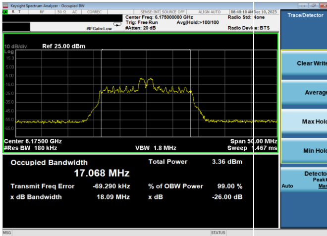
Plot 7-66. 26dB & 99% Bandwidth Plot Antenna WF7a (20MHz 802.11ax RU26 (UNII Band 5) – Ch. 45)
