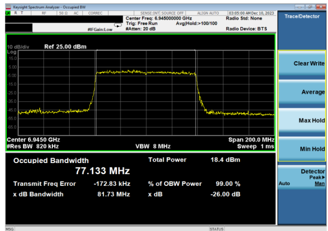
Plot 7-60. 26dB & 99% Bandwidth Plot Antenna WF8 (80MHz 802.11ax RU996 (UNII Band 8) – Ch. 199)
