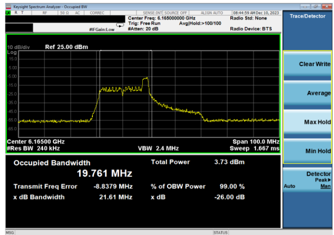
Plot 7-70. 26dB & 99% Bandwidth Plot Antenna WF7a (40MHz 802.11ax RU26 (UNII Band 5) – Ch. 43)
