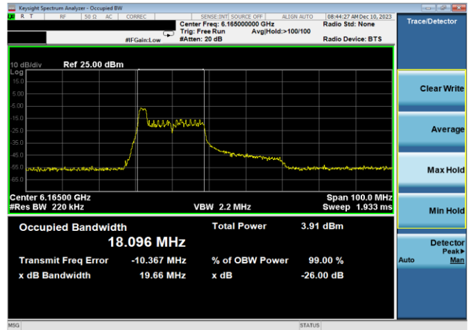
Plot 7-69. 26dB & 99% Bandwidth Plot Antenna WF7a (40MHz 802.11ax RU26 (UNII Band 5) – Ch. 43)
