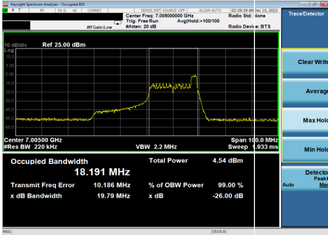
Plot 7-55. 26dB & 99% Bandwidth Plot Antenna WF8 (40MHz 802.11ax RU26 (UNII Band 8) – Ch. 211)
