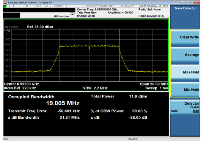
Plot 7-52. 26dB & 99% Bandwidth Plot Antenna WF8 (20MHz 802.11ax RU242 (UNII Band 8) – Ch. 209)
