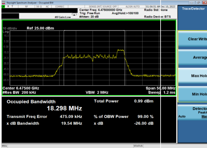
Plot 7-19. 26dB & 99% Bandwidth Plot Antenna WF8 (20MHz 802.11ax RU26 (UNII Band 6) – Ch. 105)
