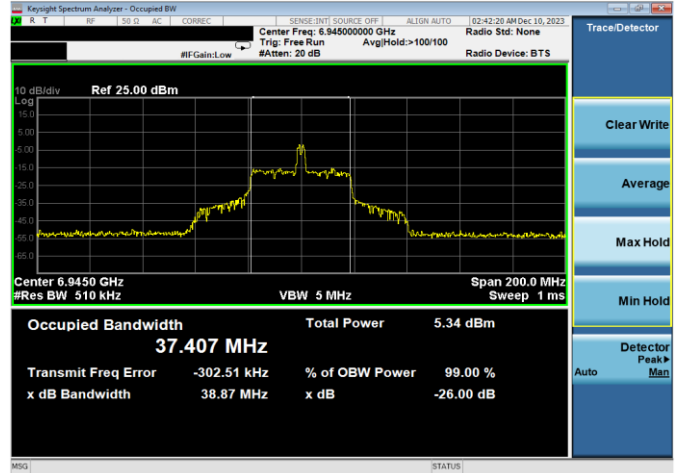
Plot 7-58. 26dB & 99% Bandwidth Plot Antenna WF8 (80MHz 802.11ax RU26 (UNII Band 8) – Ch. 199)
