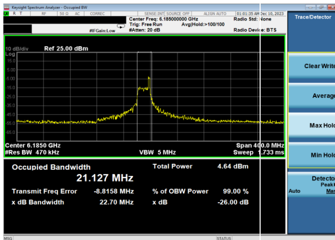
Plot 7-14. 26dB & 99% Bandwidth Plot Antenna WF8 (160MHz 802.11ax RU26 (UNII Band 5) – Ch. 47)
