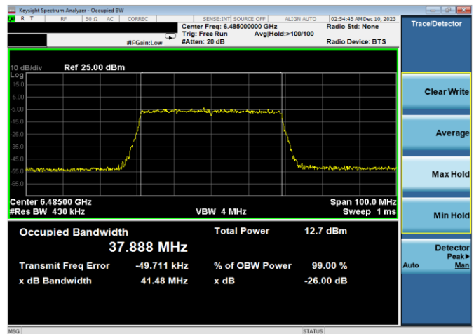
Plot 7-24. 26dB & 99% Bandwidth Plot Antenna WF8 (40MHz 802.11ax RU484 (UNII Band 6) – Ch. 107)
