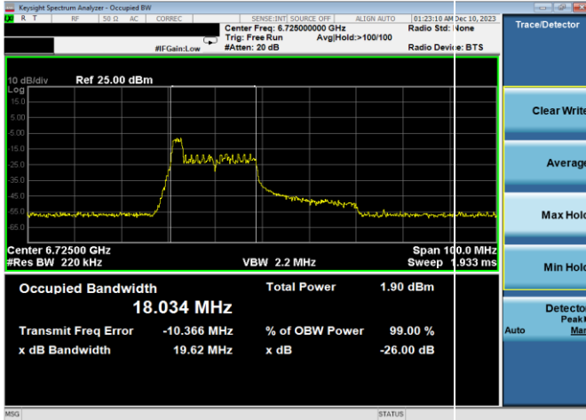
Plot 7-37. 26dB & 99% Bandwidth Plot Antenna WF8 (40MHz 802.11ax RU26 (UNII Band 7) – Ch. 155)
