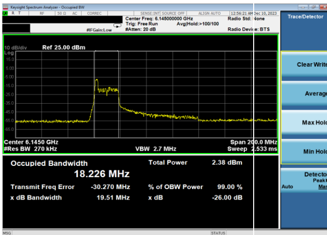
Plot 7-9. 26dB & 99% Bandwidth Plot Antenna WF8 (80MHz 802.11ax RU26 (UNII Band 5) – Ch. 39)
