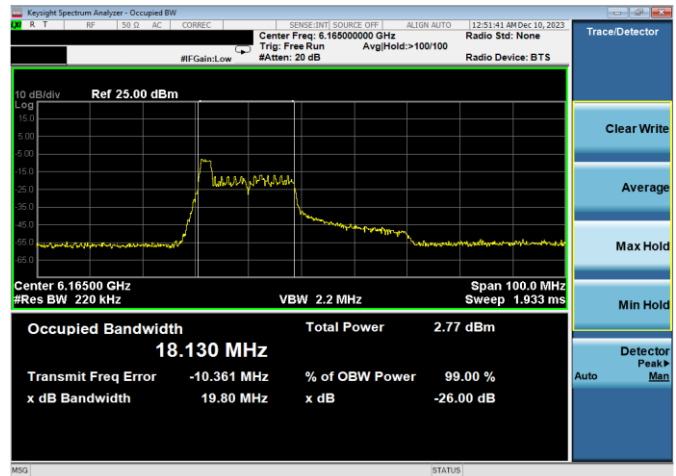
Plot 7-5. 26dB & 99% Bandwidth Plot Antenna WF8 (40MHz 802.11ax RU26 (UNII Band 5) – Ch. 43)
