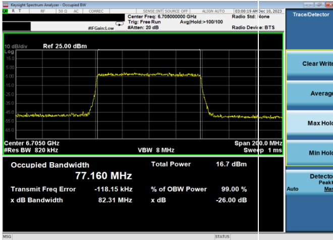
Plot 7-44. 26dB & 99% Bandwidth Plot Antenna WF8 (80MHz 802.11ax RU996 (UNII Band 7) - Ch. 151)
