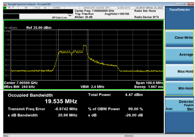
Plot 7-54. 26dB & 99% Bandwidth Plot Antenna WF8 (40MHz 802.11ax RU26 (UNII Band 8) – Ch. 211)
