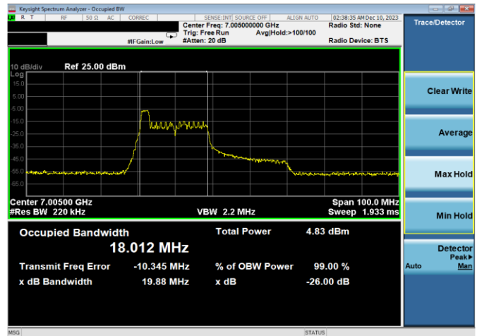
Plot 7-53. 26dB & 99% Bandwidth Plot Antenna WF8 (40MHz 802.11ax RU26 (UNII Band 8) – Ch. 211)
