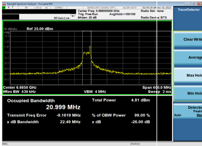
Plot 7-62. 26dB & 99% Bandwidth Plot Antenna WF8 (160MHz 802.11ax RU26 (UNII Band 8) – Ch. 207)
