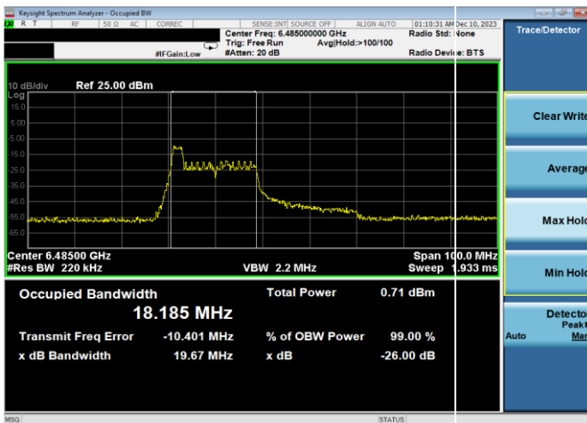
Plot 7-21. 26dB & 99% Bandwidth Plot Antenna WF8 (40MHz 802.11ax RU26 (UNII Band 6) – Ch. 107)
