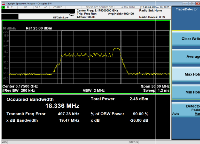
Plot 7-3. 26dB & 99% Bandwidth Plot Antenna WF8 (20MHz 802.11ax RU26 (UNII Band 5) – Ch. 45)
