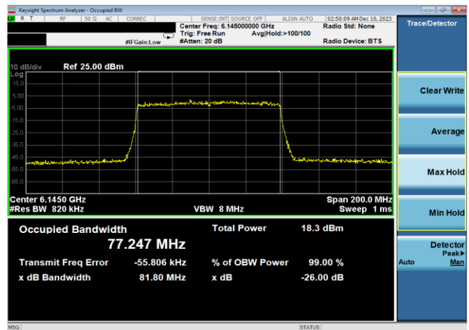
Plot 7-12. 26dB & 99% Bandwidth Plot Antenna WF8 (80MHz 802.11ax RU996 (UNII Band 5) – Ch. 39)
