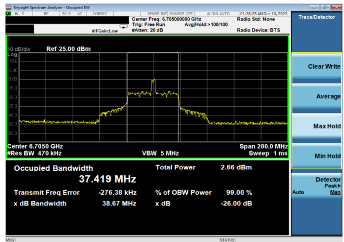
Plot 7-42. 26dB & 99% Bandwidth Plot Antenna WF8 (80MHz 802.11ax RU26 (UNII Band 7) – Ch. 151)
