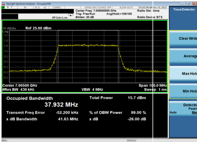
Plot 7-56. 26dB & 99% Bandwidth Plot Antenna WF8 (40MHz 802.11ax RU484 (UNII Band 8) – Ch. 211)
