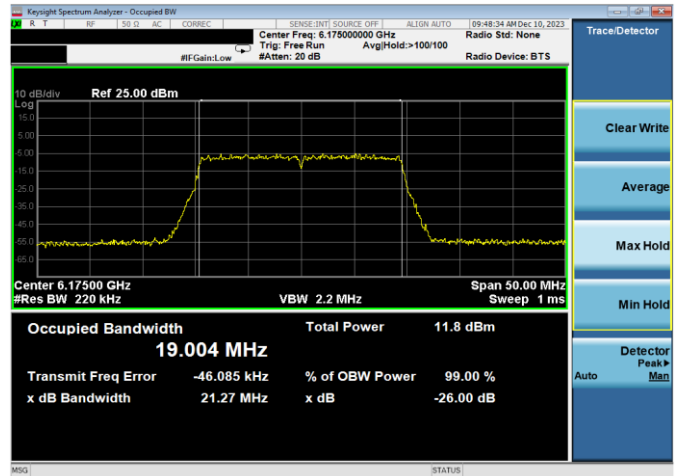
Plot 7-68. 26dB & 99% Bandwidth Plot Antenna WF7a (20MHz 802.11ax RU242 (UNII Band 5) – Ch. 45)
