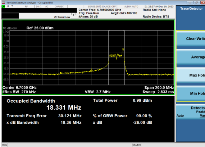
Plot 7-43. 26dB & 99% Bandwidth Plot Antenna WF8 (80MHz 802.11ax RU26 (UNII Band 7) - Ch. 151)
