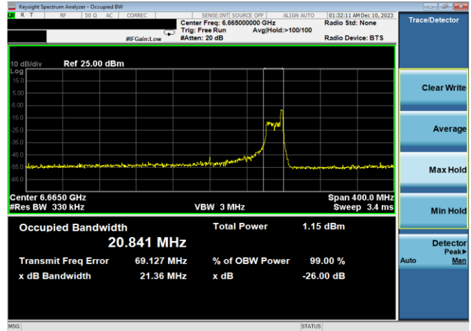
Plot 7-47. 26dB & 99% Bandwidth Plot Antenna WF8 (160MHz 802.11ax RU26 (UNII Band 7) - Ch. 143)
