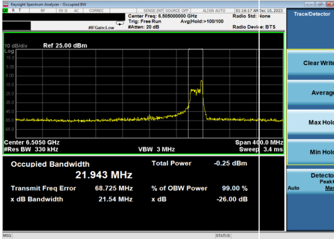
Plot 7-31. 26dB & 99% Bandwidth Plot Antenna WF8 (160MHz 802.11ax RU26 (UNII Band 6) – Ch. 111)
