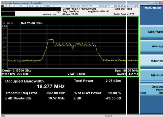
Plot 7-1. 26dB & 99% Bandwidth Plot Antenna WF8 (20MHz 802.11ax RU26 (UNII Band 5) – Ch. 45)
