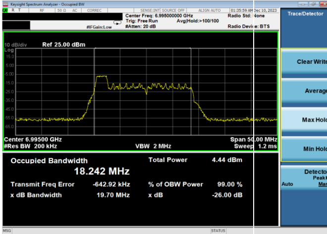
Plot 7-49. 26dB & 99% Bandwidth Plot Antenna WF8 (20MHz 802.11ax RU26 (UNII Band 8) – Ch. 209)
