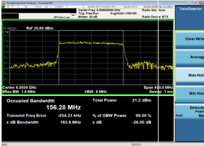
Plot 7-32. 26dB & 99% Bandwidth Plot Antenna WF8 (160MHz 802.11ax RU996x2 (UNII Band 6) – Ch. 111)
