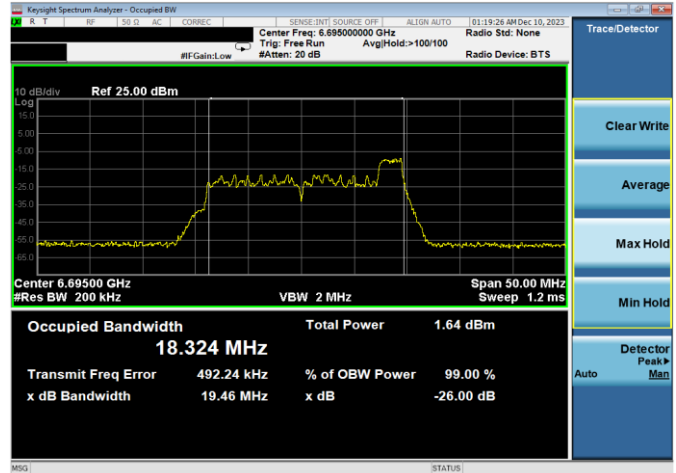
Plot 7-35. 26dB & 99% Bandwidth Plot Antenna WF8 (20MHz 802.11ax RU26 (UNII Band 7) – Ch. 149)
