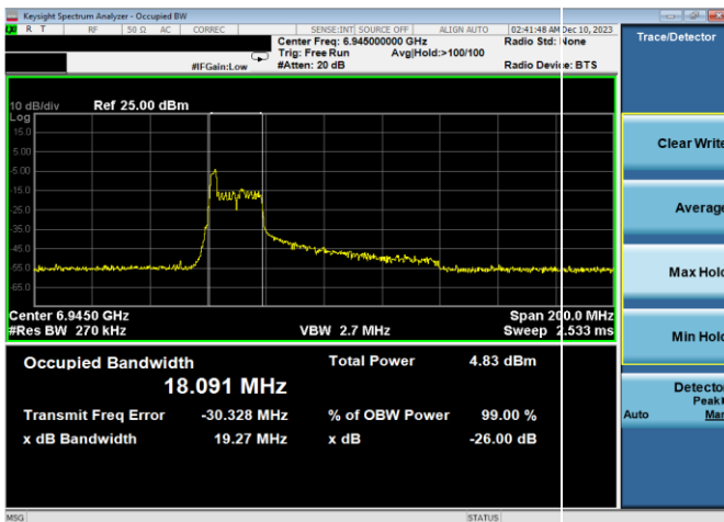
Plot 7-57. 26dB & 99% Bandwidth Plot Antenna WF8 (80MHz 802.11ax RU26 (UNII Band 8) – Ch. 199)
