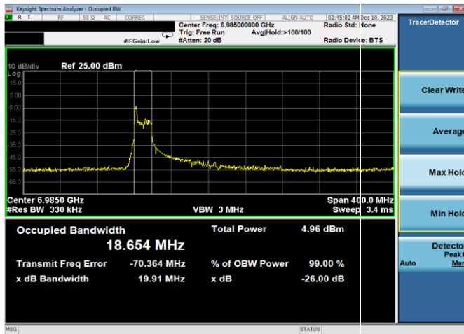
Plot 7-61. 26dB & 99% Bandwidth Plot Antenna WF8 (160MHz 802.11ax RU26 (UNII Band 8) – Ch. 207)
