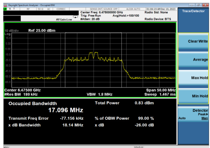
Plot 7-18. 26dB & 99% Bandwidth Plot Antenna WF8 (20MHz 802.11ax RU26 (UNII Band 6) – Ch. 105)
