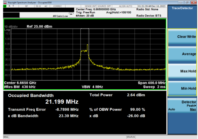
Plot 7-46. 26dB & 99% Bandwidth Plot Antenna WF8 (160MHz 802.11ax RU26 (UNII Band 7) - Ch. 143)
