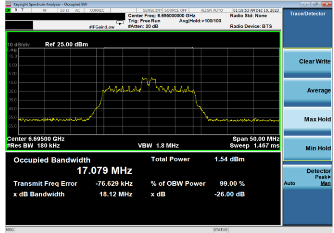
Plot 7-34. 26dB & 99% Bandwidth Plot Antenna WF8 (20MHz 802.11ax RU26 (UNII Band 7) – Ch. 149)
