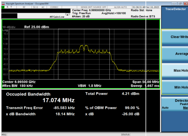
Plot 7-50. 26dB & 99% Bandwidth Plot Antenna WF8 (20MHz 802.11ax RU26 (UNII Band 8) – Ch. 209)
