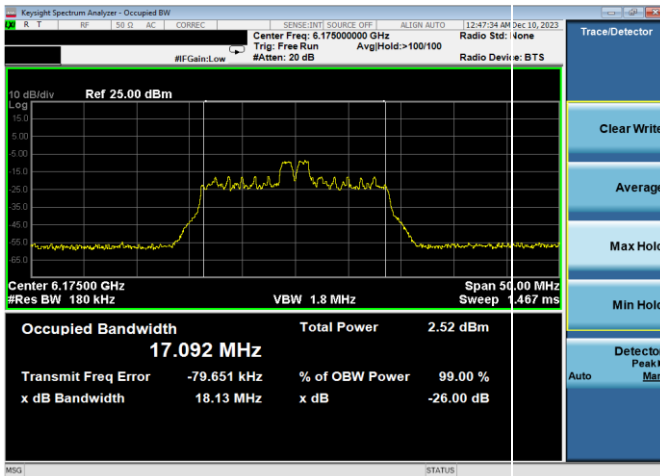
Plot 7-2. 26dB & 99% Bandwidth Plot Antenna WF8 (20MHz 802.11ax RU26 (UNII Band 5) – Ch. 45)
