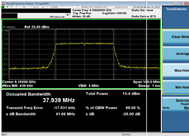
Plot 7-8. 26dB & 99% Bandwidth Plot Antenna WF8 (40MHz 802.11ax RU484 (UNII Band 5) – Ch. 43)
