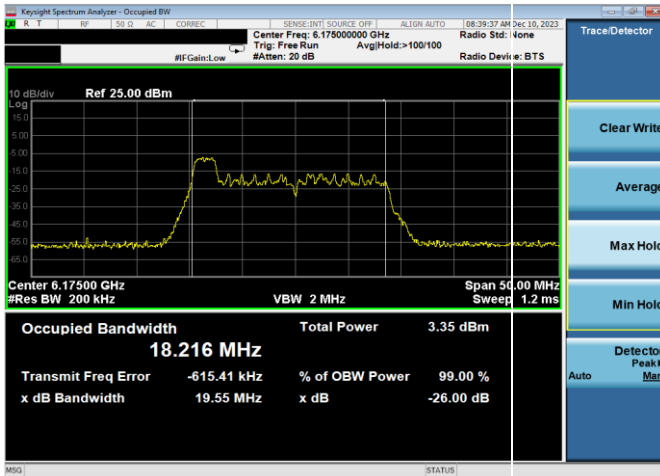
Plot 7-65. 26dB & 99% Bandwidth Plot Antenna WF7a (20MHz 802.11ax RU26 (UNII Band 5) – Ch. 45)
