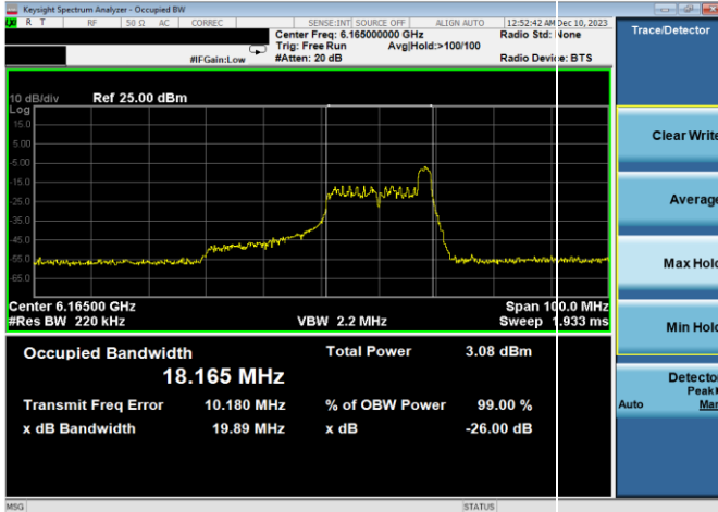
Plot 7-7. 26dB & 99% Bandwidth Plot Antenna WF8 (40MHz 802.11ax RU26 (UNII Band 5) – Ch. 43)
