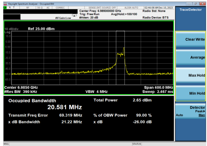
Plot 7-63. 26dB & 99% Bandwidth Plot Antenna WF8 (160MHz 802.11ax RU26 (UNII Band 8) – Ch. 207)
