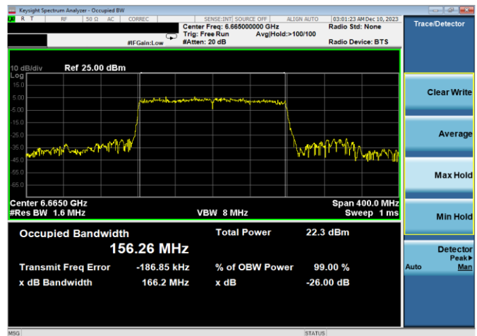
Plot 7-48. 26dB & 99% Bandwidth Plot Antenna WF8 (160MHz 802.11ax RU996x2 (UNII Band 7) - Ch. 143)
