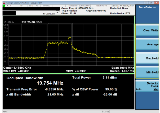
Plot 7-6. 26dB & 99% Bandwidth Plot Antenna WF8 (40MHz 802.11ax RU26 (UNII Band 5) – Ch. 43)
