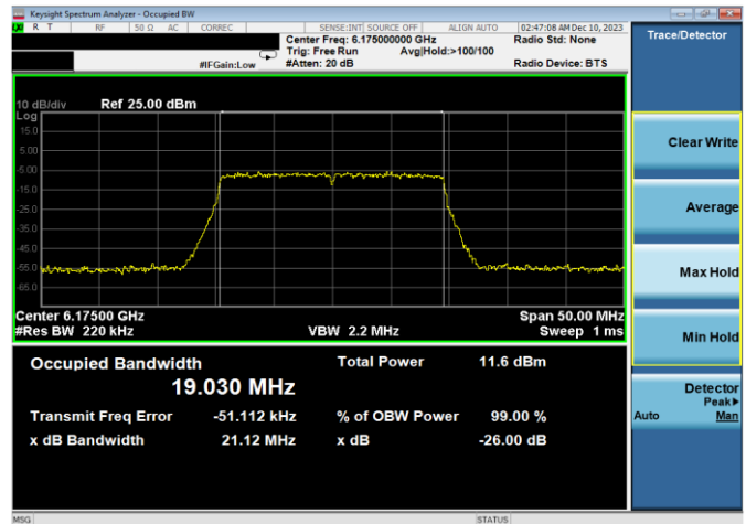
Plot 7-4. 26dB & 99% Bandwidth Plot Antenna WF8 (20MHz 802.11ax RU242 (UNII Band 5) – Ch. 45)
