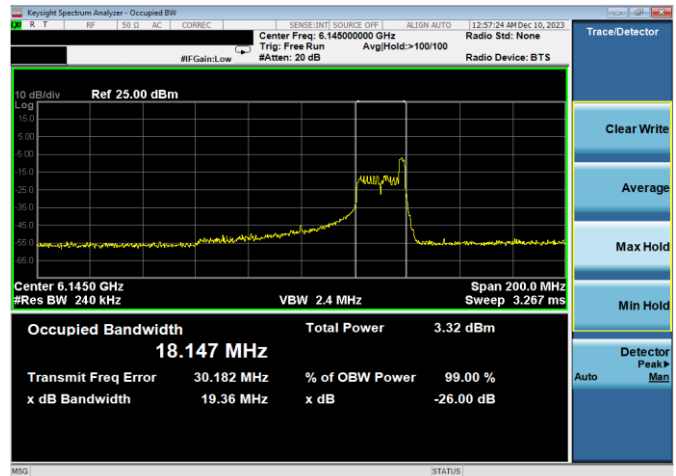
Plot 7-11. 26dB & 99% Bandwidth Plot Antenna WF8 (80MHz 802.11ax RU26 (UNII Band 5) – Ch. 39)
