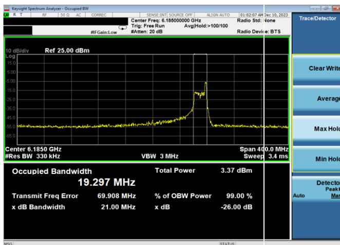
Plot 7-15. 26dB & 99% Bandwidth Plot Antenna WF8 (160MHz 802.11ax RU26 (UNII Band 5) – Ch. 47)
