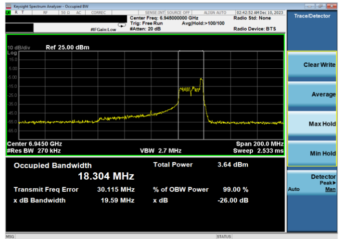
Plot 7-59. 26dB & 99% Bandwidth Plot Antenna WF8 (80MHz 802.11ax RU26 (UNII Band 8) – Ch. 199)
