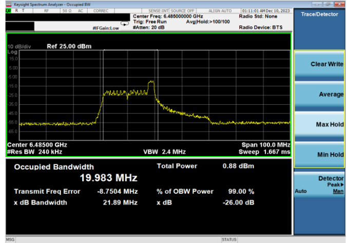
Plot 7-22. 26dB & 99% Bandwidth Plot Antenna WF8 (40MHz 802.11ax RU26 (UNII Band 6) – Ch. 107)
