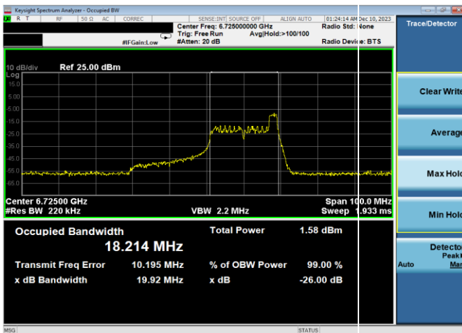
Plot 7-39. 26dB & 99% Bandwidth Plot Antenna WF8 (40MHz 802.11ax RU26 (UNII Band 7) – Ch. 155)
