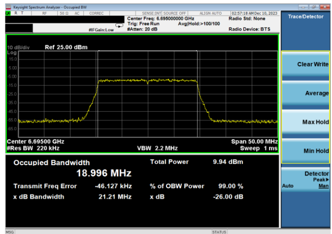
Plot 7-36. 26dB & 99% Bandwidth Plot Antenna WF8 (20MHz 802.11ax RU242 (UNII Band 7) – Ch. 149)
