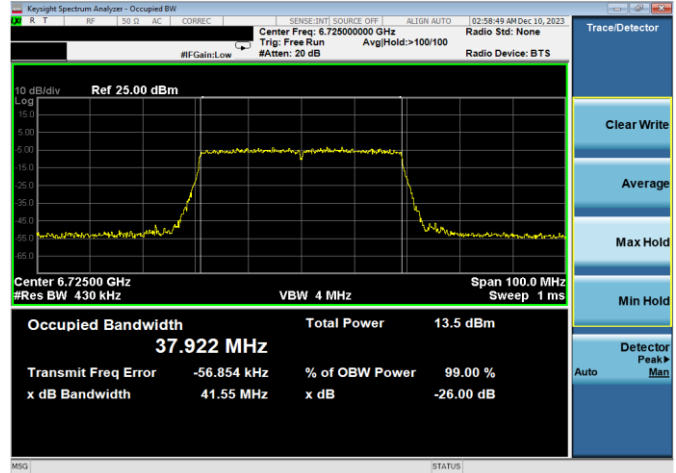
Plot 7-40. 26dB & 99% Bandwidth Plot Antenna WF8 (40MHz 802.11ax RU484 (UNII Band 7) – Ch. 155)
