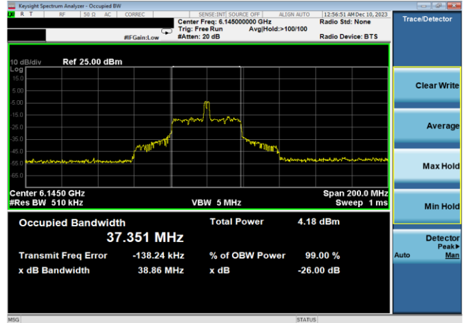
Plot 7-10. 26dB & 99% Bandwidth Plot Antenna WF8 (80MHz 802.11ax RU26 (UNII Band 5) – Ch. 39)
