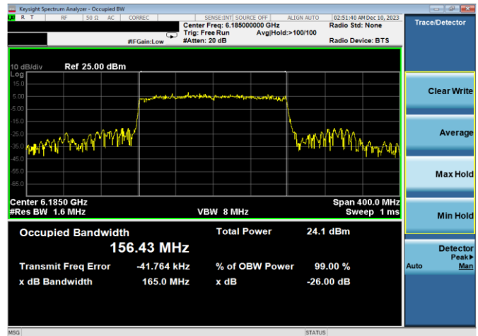
Plot 7-16. 26dB & 99% Bandwidth Plot Antenna WF8 (160MHz 802.11ax RU996x2 (UNII Band 5) – Ch. 47)
