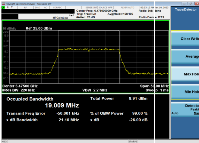
Plot 7-20. 26dB & 99% Bandwidth Plot Antenna WF8 (20MHz 802.11ax RU242 (UNII Band 6) – Ch. 105)
