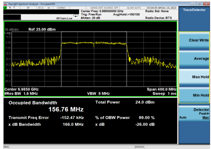
Plot 7-64. 26dB & 99% Bandwidth Plot Antenna WF8 (160MHz 802.11ax RU996x2 (UNII Band 8) – Ch. 207)
