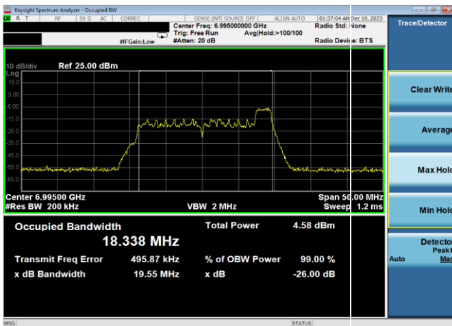
Plot 7-51. 26dB & 99% Bandwidth Plot Antenna WF8 (20MHz 802.11ax RU26 (UNII Band 8) – Ch. 209)
