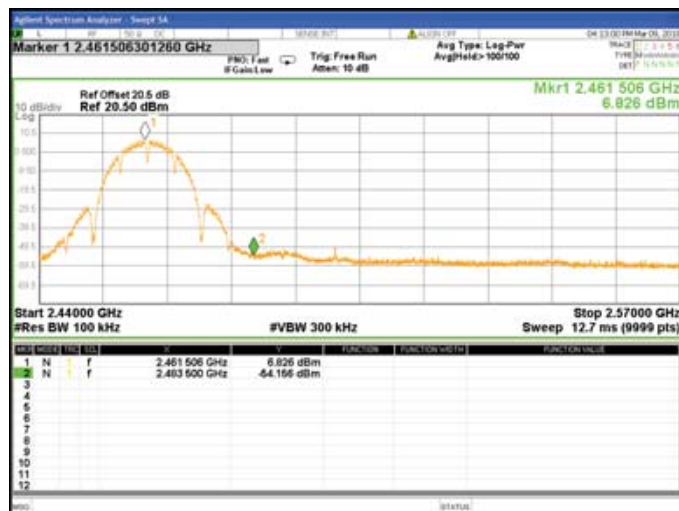
Chain1 : Authorized Band Bandedge @ 802.11b Mode High
