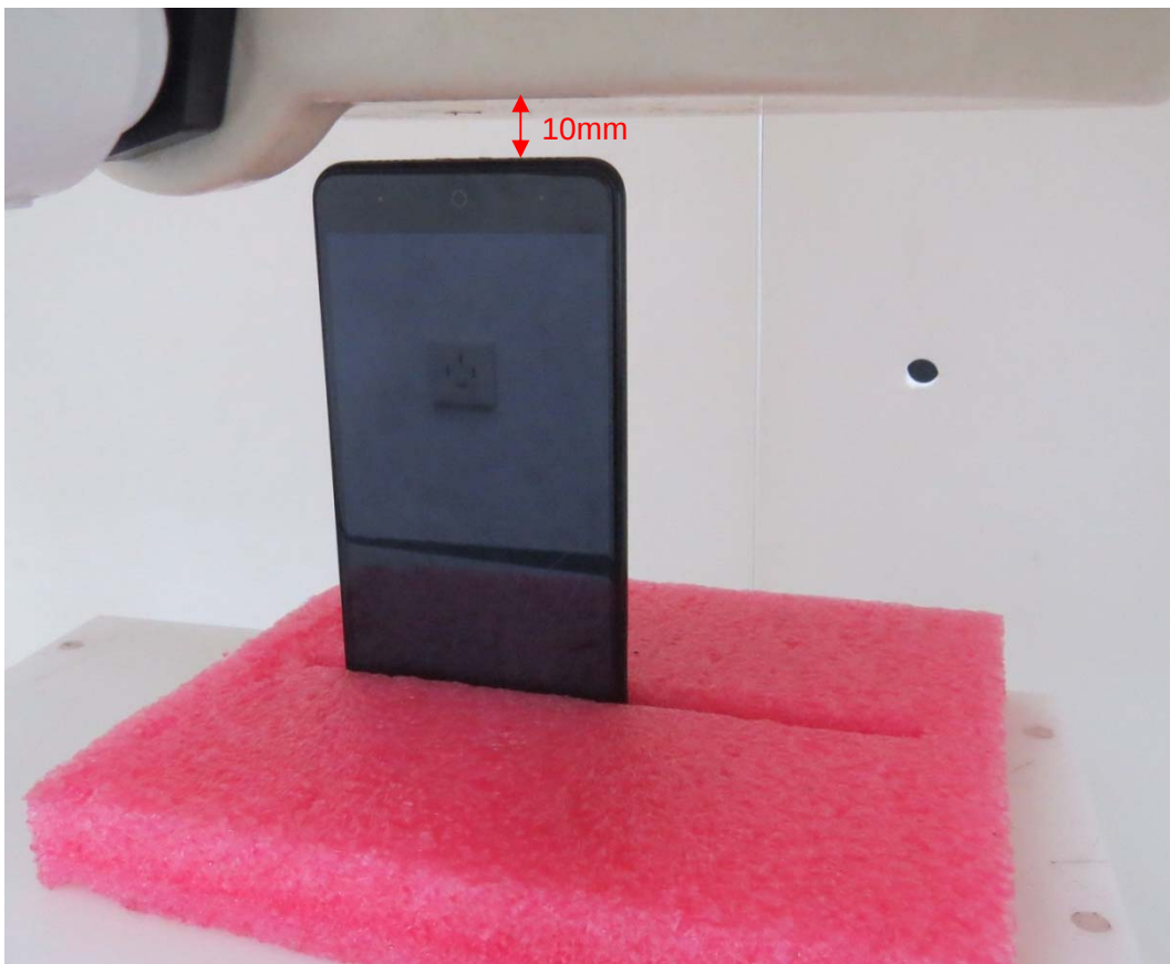
Picture 10: Bottom Edge, the distance from handset to the bottom of the Phantom is 10mm
