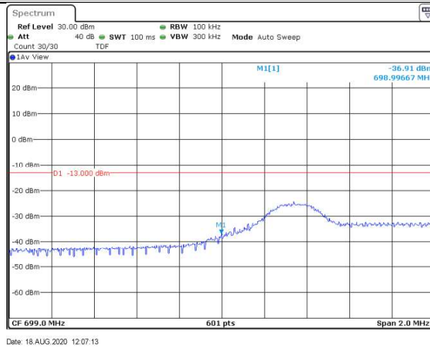
Band12-5MHz-QPSK-23035-1RB#0
