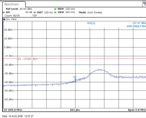
Band12-5MHz-16QAM-23035-25RB#0
