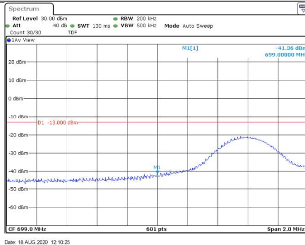
Band12-10MHz-16QAM-23060-50RB#0
