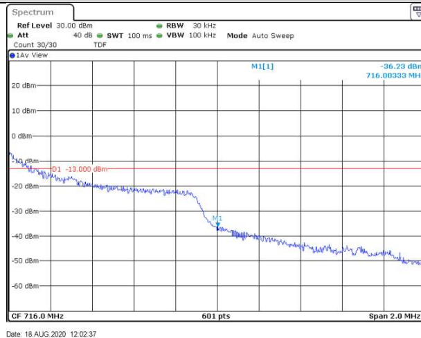
Band12-1.4MHz-16QAM-23173-6RB#0
