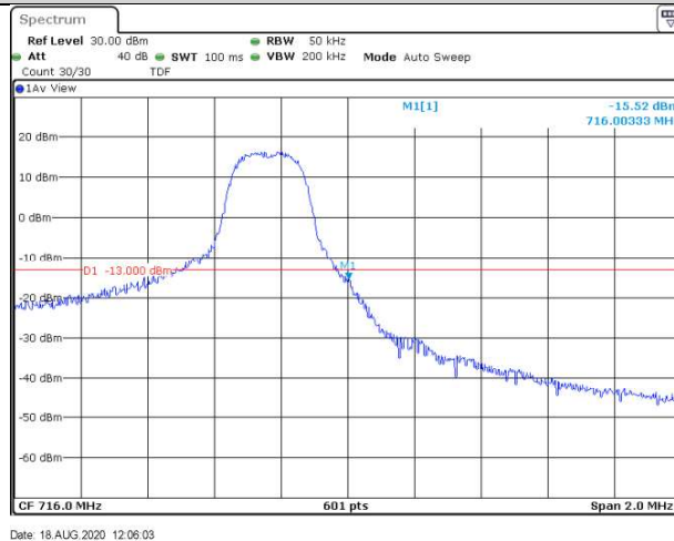
Band12-3MHz-16QAM-23165-15RB#0
