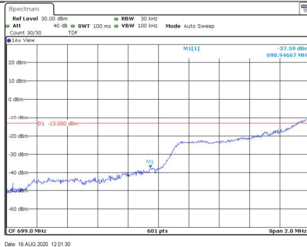
Band12-1.4MHz-16QAM-23017-6RB#0
