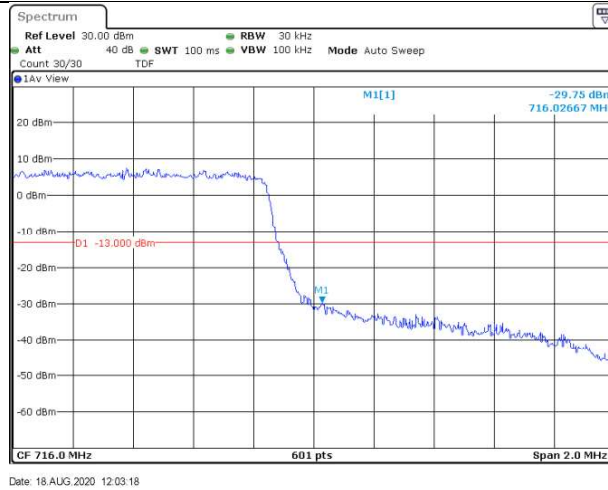
Band12-1.4MHz-16QAM-23017-1RB#0
