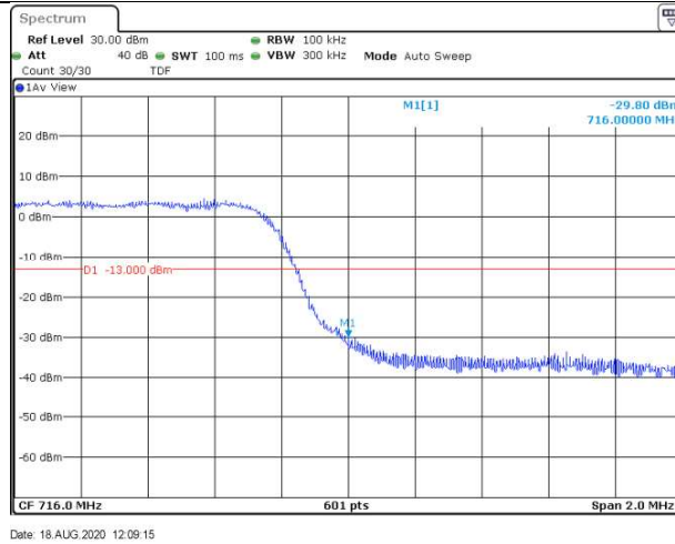
Band12-5MHz-16QAM-23035-1RB#0
