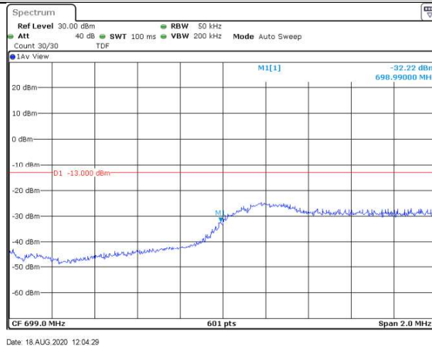
Band12-3MHz-16QAM-23025-15RB#0
