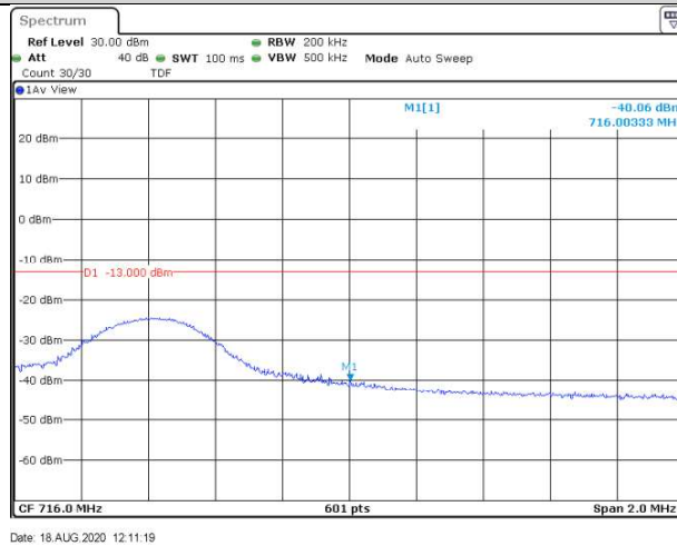
Band12-10MHz-QPSK-23130-1RB#49
