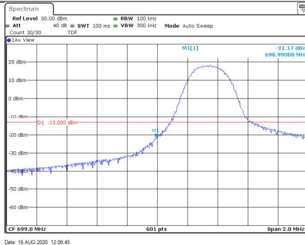
Band12-5MHz-QPSK-23035-25RB#0
