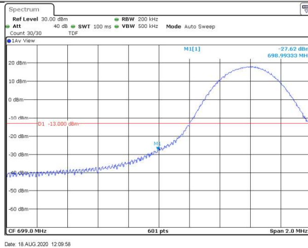
Band12-10MHz-16QAM-23060-1RB#49
