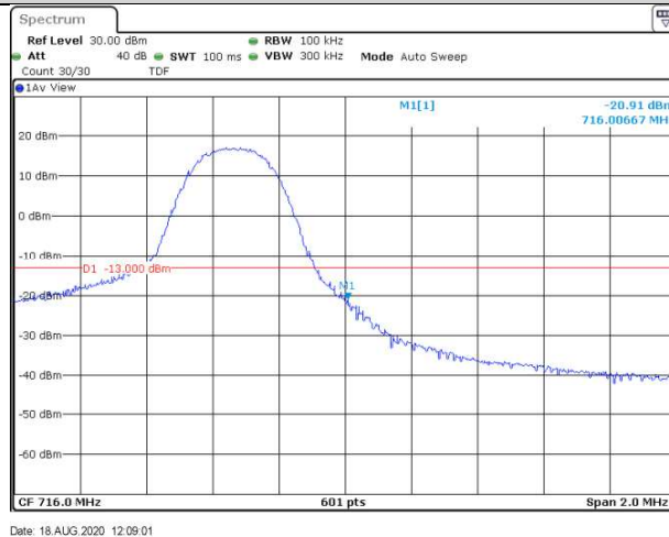
Band12-5MHz-16QAM-23155-25RB#0
