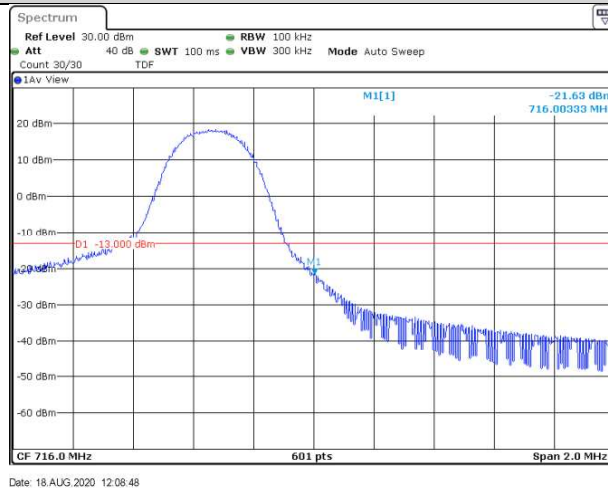
Band12-5MHz-QPSK-23155-25RB#0
