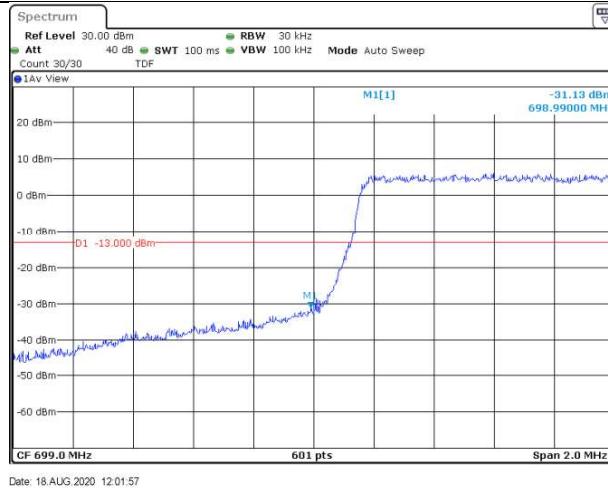
Band12-1.4MHz-16QAM-23173-1RB#5
