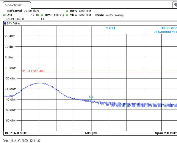
Band12-10MHz-16QAM-23130-50RB#0
