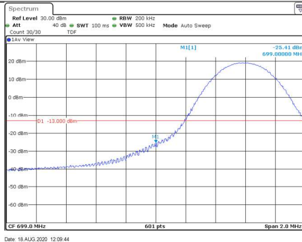
Band12-10MHz-QPSK-23060-50RB#0
