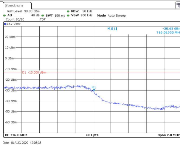
Band12-3MHz-16QAM-23165-1RB#14
