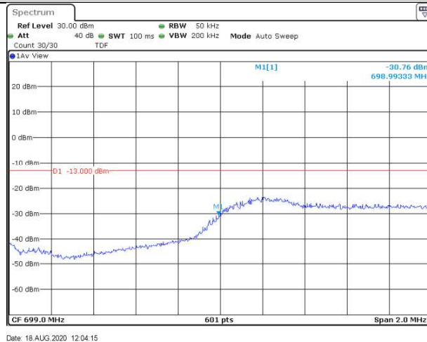
Band12-3MHz-QPSK-23025-15RB#0
