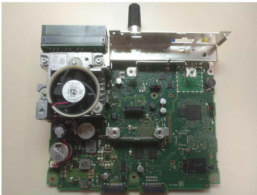
Photo 2: Main PCB front side view
