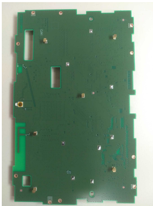
Photo 6: Switch-PCB back side view
