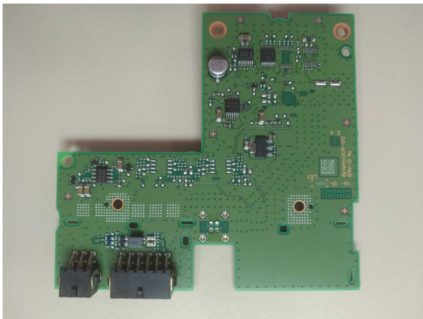
Photo 4: Sub-PCB back side view
