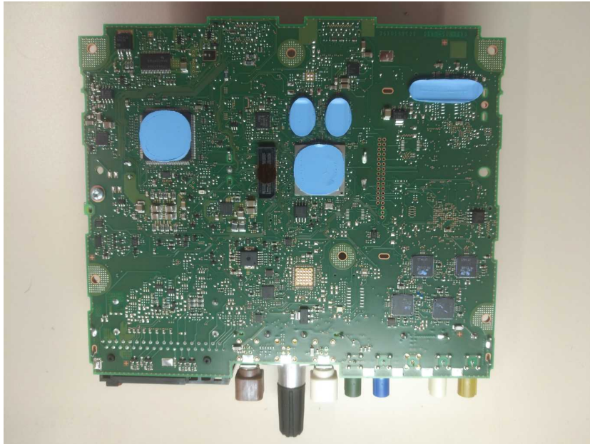
Photo 1: Main PCB back side view
