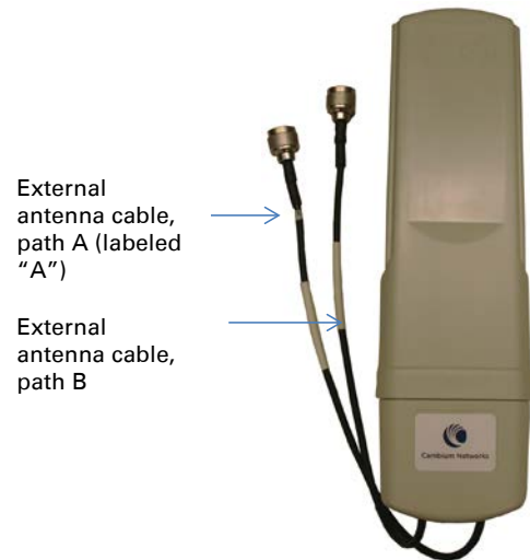
Figure 11 Connectorized SM
