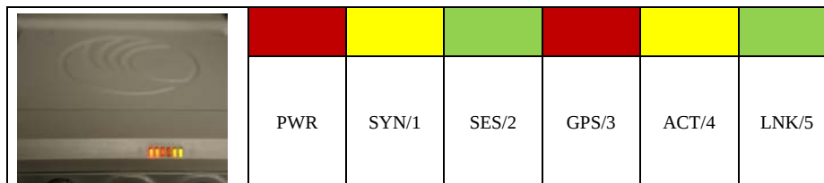
Figure 7 AP diagnostic LEDs, viewed from front of the unit
