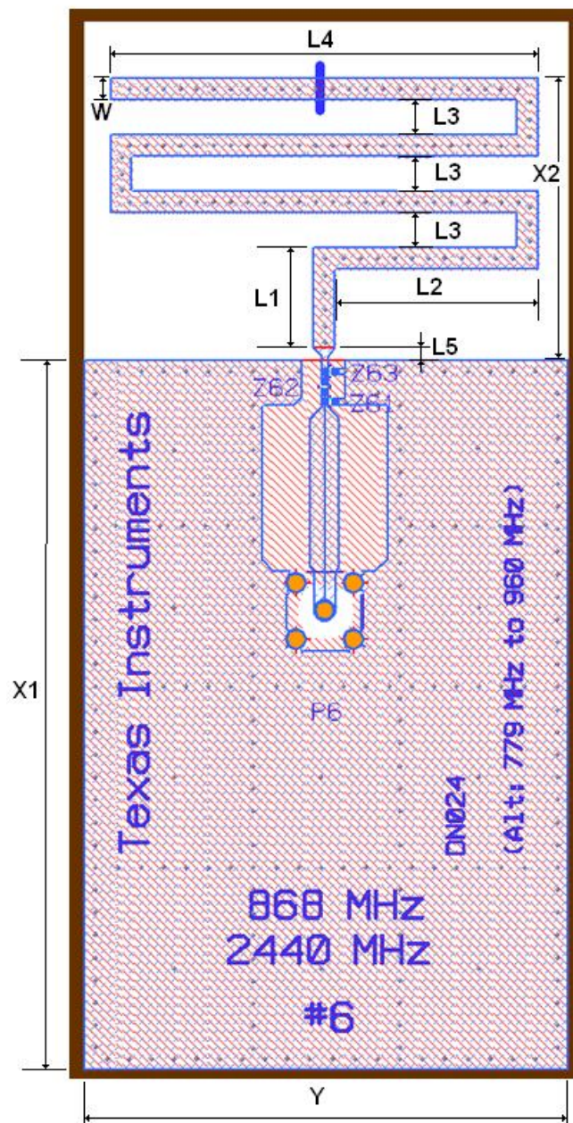
Figure 2. Antenna Dimensions
