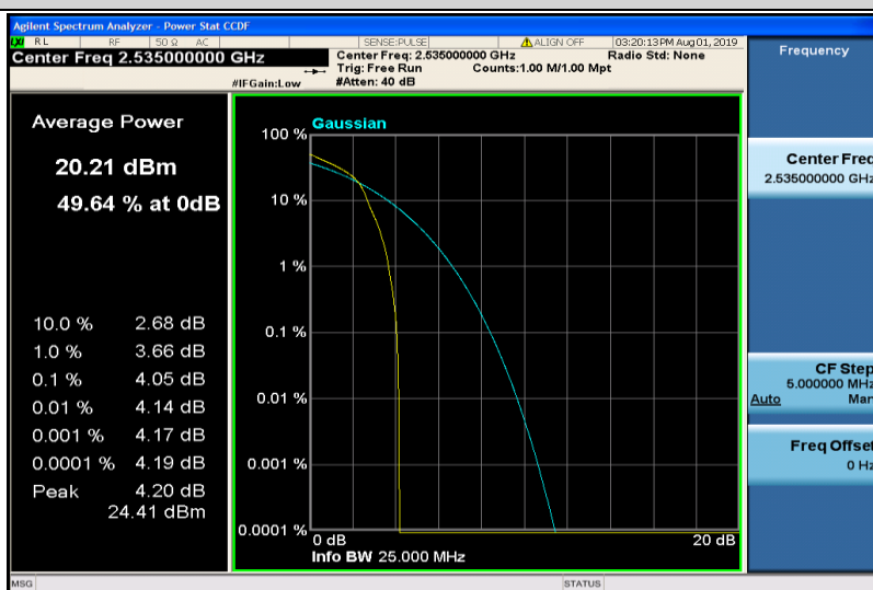
Band7-10MHz-16QAM-21100-1RB#0
