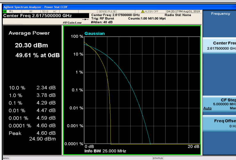
Band38-5MHz-QPSK-38225-25RB#0
