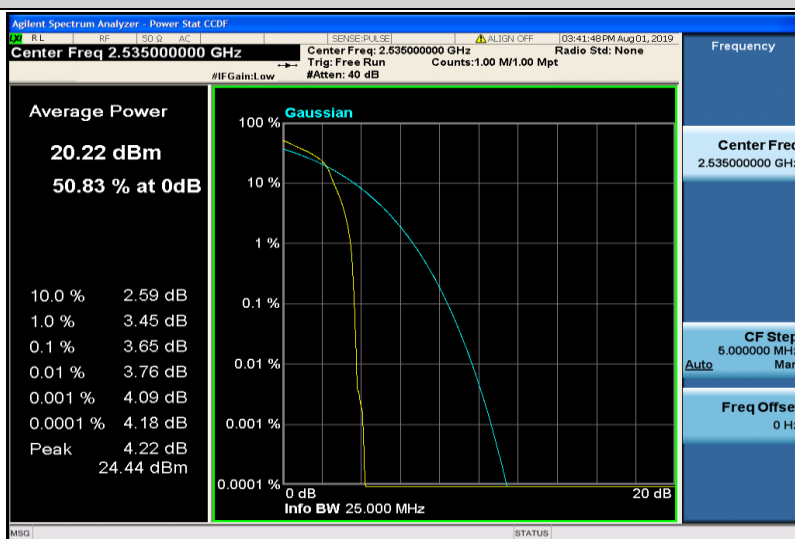
Band7-15MHz-16QAM-21100-1RB#0
