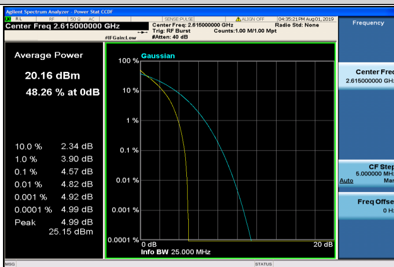
Band38-10MHz-QPSK-38200-50RB#0
