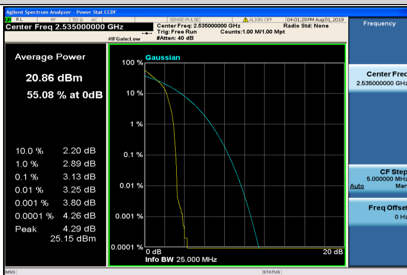
Band7-20MHz-QPSK-21100-1RB#0
