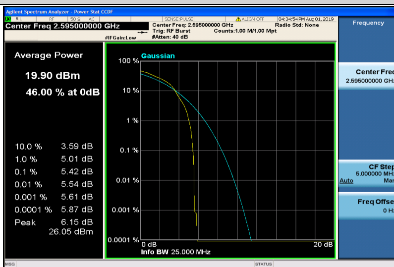
Band38-10MHz-16QAM-38000-1RB#0
