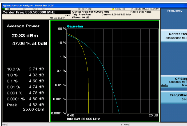
Band5-5MHz-16QAM-20525-1RB#0
