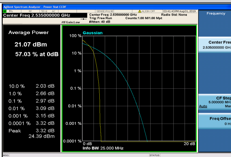
Band7-15MHz-QPSK-21100-1RB#0
