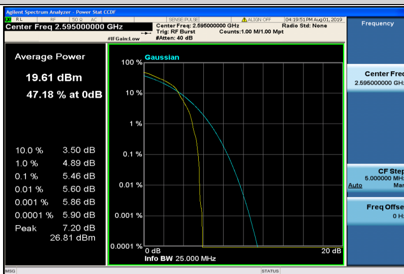
Band38-5MHz-16QAM-38000-1RB#0
