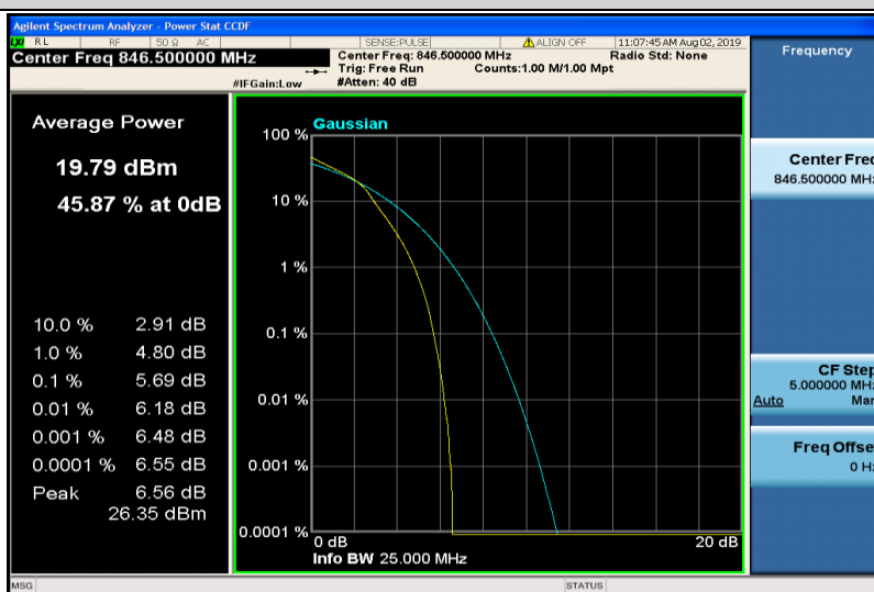
Band5-5MHz-16QAM-20625-25RB#0
