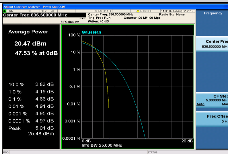
Band5-10MHz-16QAM-20525-1RB#0
