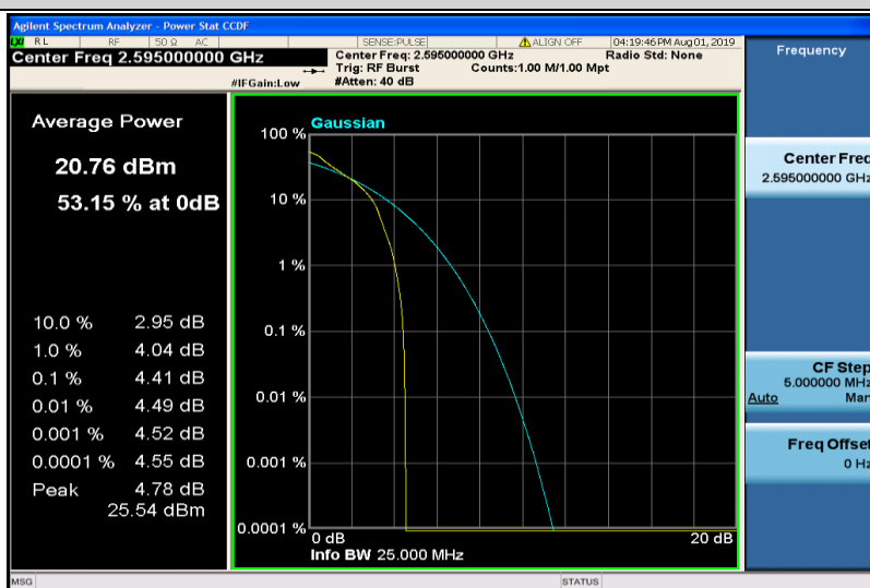
Band38-5MHz-QPSK-38000-1RB#0
