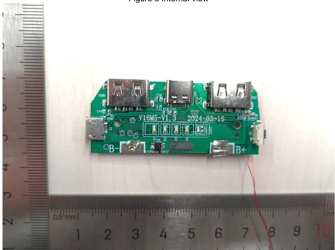
Figure 9 Top view of mainboard
