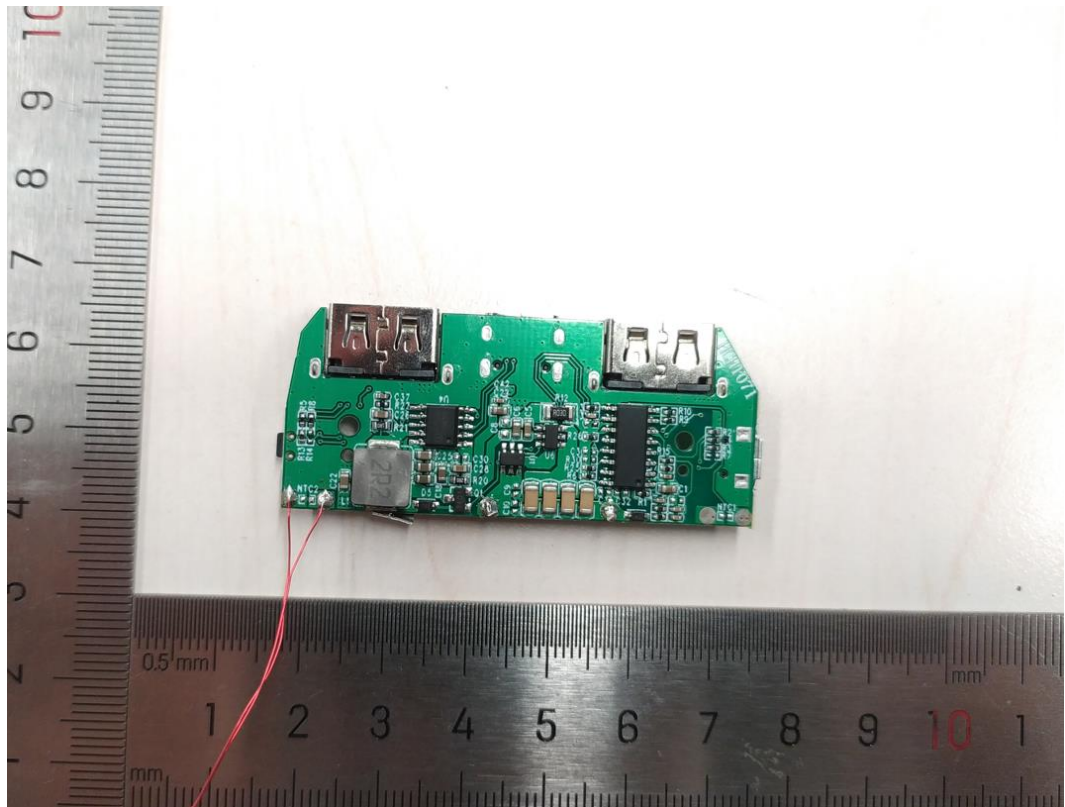
Figure 10 Bottom view of mainboard
