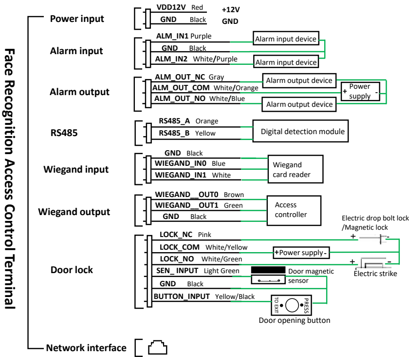
Figure 1-1 Wiring Schematic Diagrams (without Security Module)
