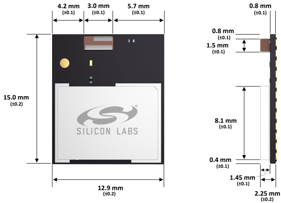
Figure 8.1. Module Dimensions
