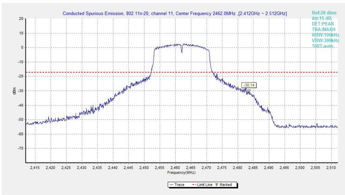
Fig.B.6.1.65 Transmitter Spurious Emission - Conducted (802.11n-HT20, Ch11, Center Frequency)
