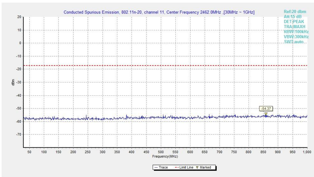
Fig.B.6.1.66 Transmitter Spurious Emission - Conducted (802.11n-HT20, Ch11, 30 MHz-1 GHz)
