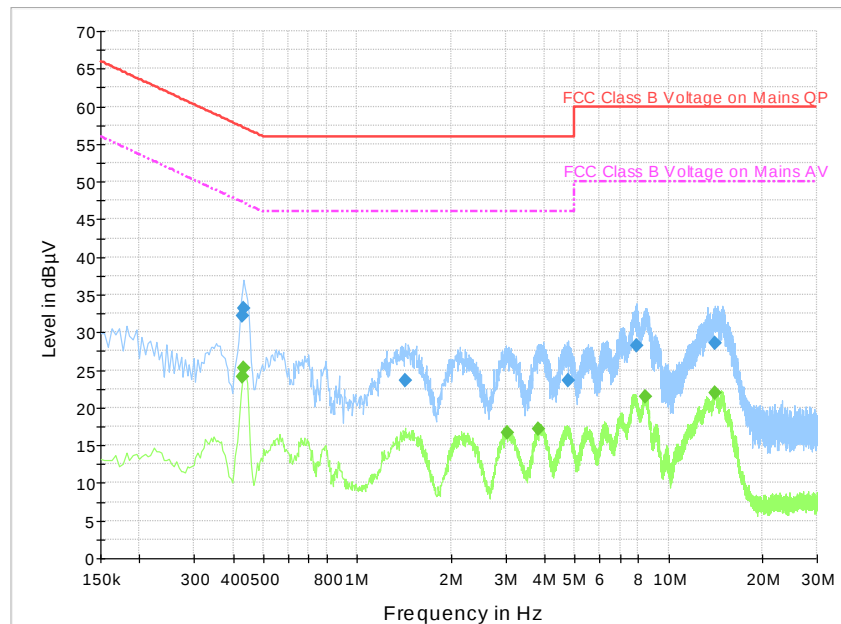
Fig.B.7.2 AC Powerline Conducted Emission-Iidle
