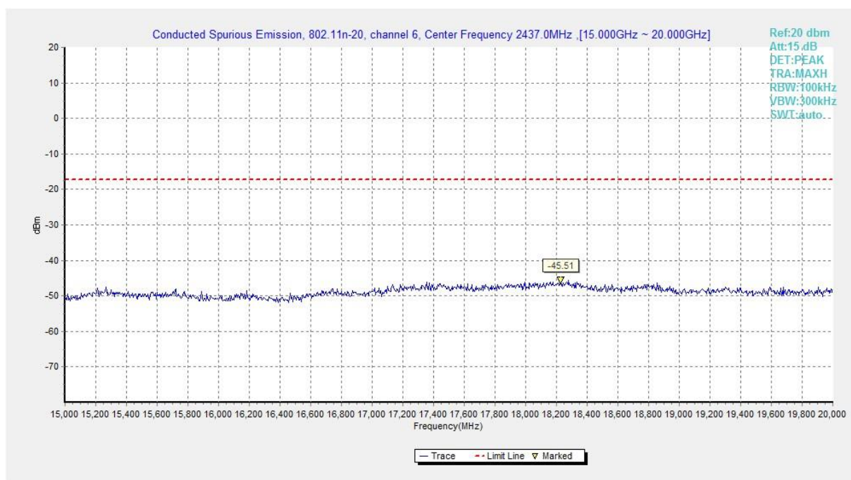
Fig.B.6.1.63 Transmitter Spurious Emission - Conducted (802.11n-HT20, Ch6, 15 GHz-20 GHz)
