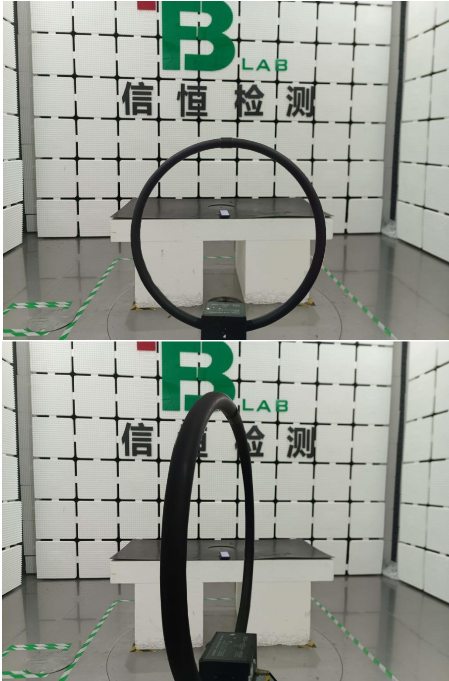
Emissions in restricted frequency bands (0.15-30 MHz)
