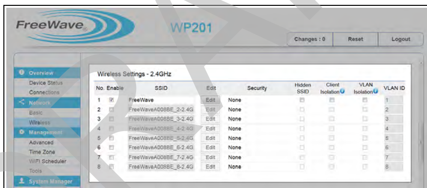
Figure 35: Wireless window - Wireless Settings area
