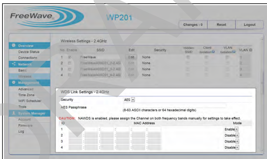
Figure 51: Wireless window - WDS Link Settings area
