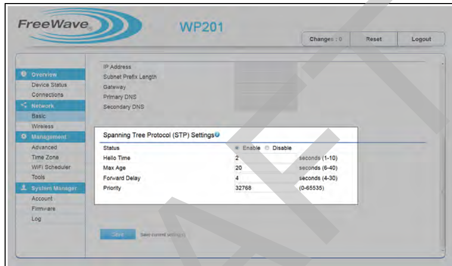
Figure 145: Basic window - Spanning Tree Protocol (STP) Settings area
