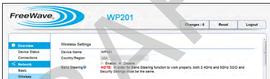
Figure 48: Wireless window - Wireless Settings area
