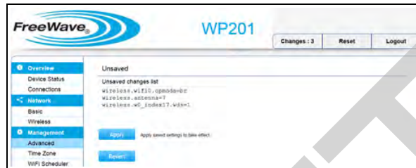
Figure 154: Unsaved window showing changes to apply.
