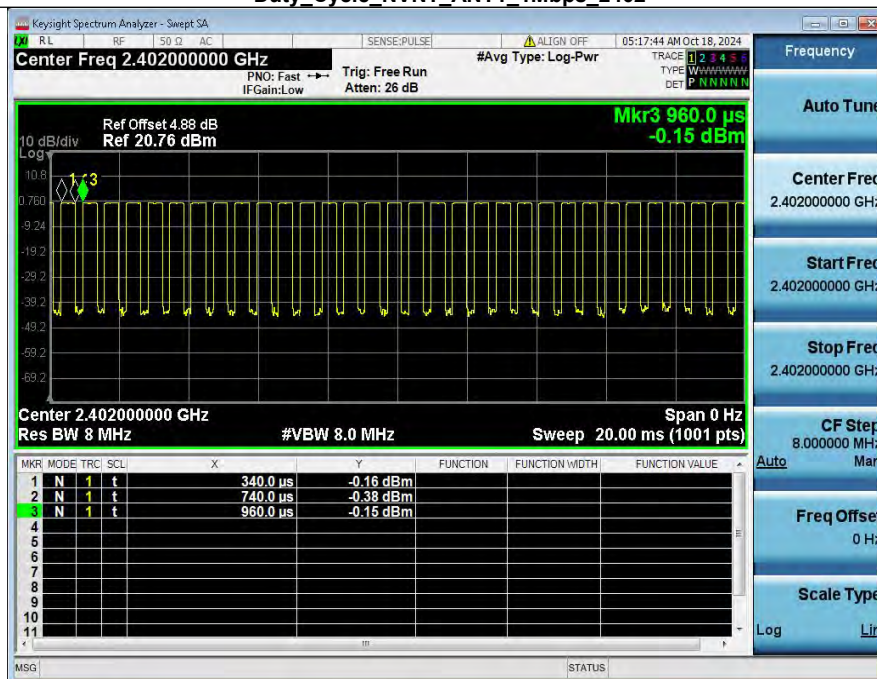
Duty_Cycle_NVNT_ANT1_1Mbps_2402
