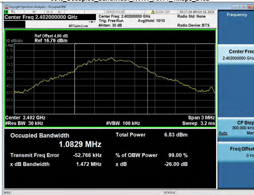
99%_Occupied_Bandwidth_NVNT_ANT1_1Mbps_2402
