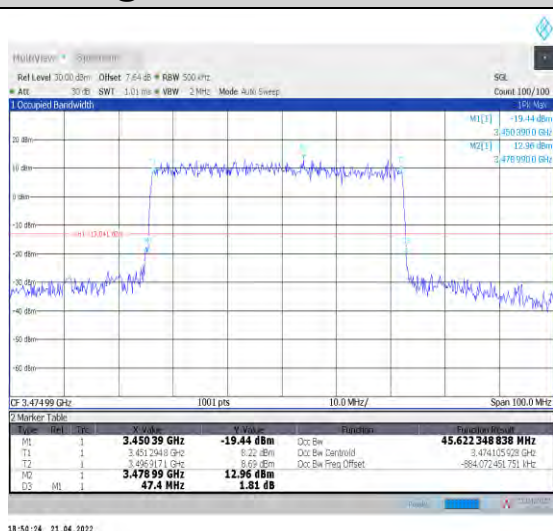
1-N78-3450-3550--30-50-L-4-DFT-64QAM-Out_Ful l-128@0-Ant1-45.622-47.400-≤50-PASS
