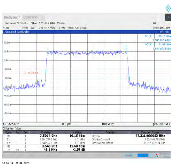
1-N78-3450-3550--30-50-H-8-CP-64QAM-Outer_Full -133@0-Ant1-47.222-49.200-≤50-PASS
