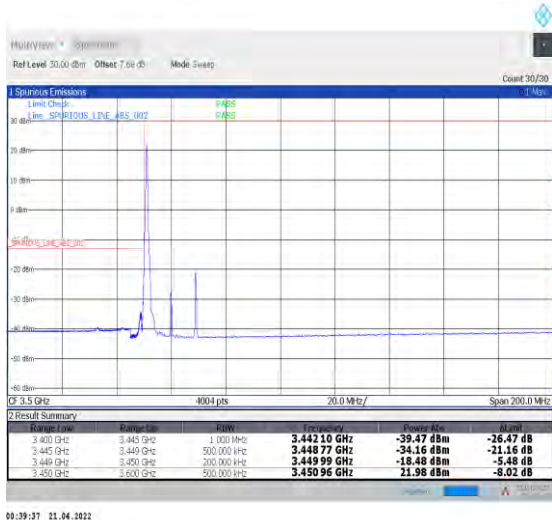
1-N78-3450-3550--30-20-L-4-CP-QPSK-Edge_1RB_L eft-1@0-Ant1-PASS-see graph
