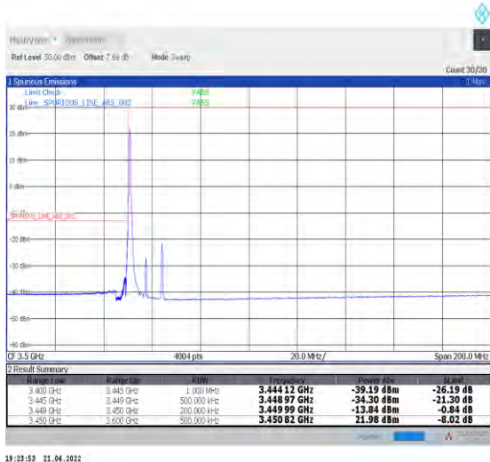
1-N78-3450-3550--30-15-L-4-CP-QPSK-Edge_1RB_L_eff-1@0-Ant1-PASS-see graph
