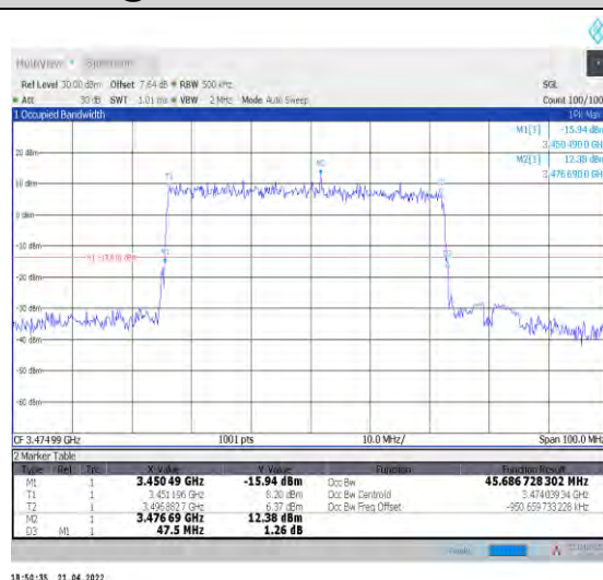
1-N78-3450-3550--30-50-L-5-DFT-256QAM-Out_F ull-128@0-Ant1-45.687-47.500-≤50-PASS
