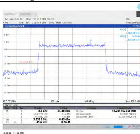
1-N78-3450-3550--30-50-H-9-CP-256QAM-Outer_F ull-133@0-Ant1-47.284-49.600-≤50-PASS
