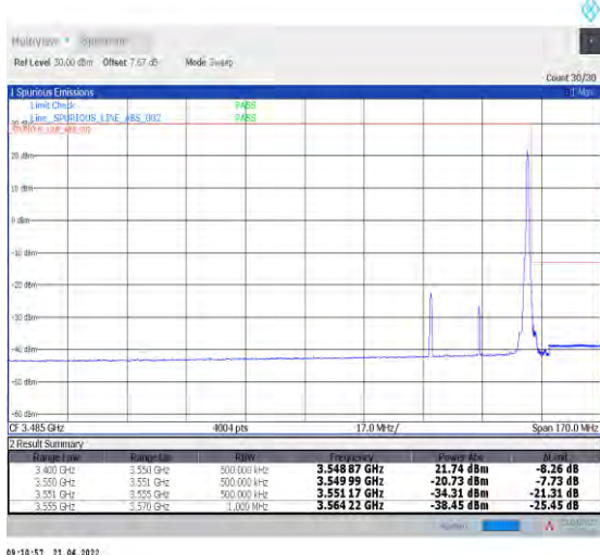
1-N78-3450-3550--30-30-H-5-CP-QPSK-Edge_1RB_R ight-1@77-Ant1-PASS-see graph
