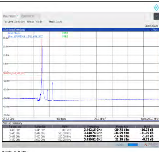
1-N78-3450-3550--30-15-L-1-DFT-PI2BPSK-Edge_1R_B_Left-1@0-Ant1-PASS-see graph
