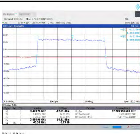
1-N78-3450-3550--30-60-L-1-DFT-QPSK-Outer_Full- 162@0-Ant1-57.79-60.360-≤60-PASS
