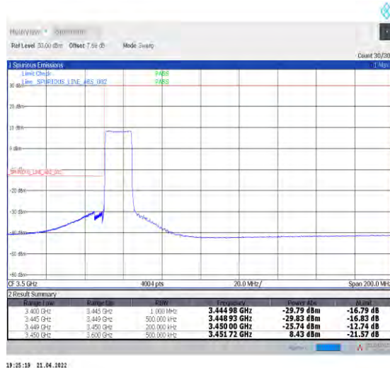
1-N78-3450-3550--30-15-L-6-CP-QPSK-Outer_Ful l-38@0-Ant1-PASS-see graph
