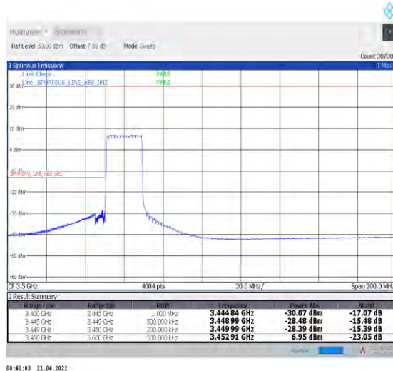
1-N78-3450-3550--30-20-L-6-CP-QPSK-Outer_Ful l-51@0-Ant1-PASS-see graph
