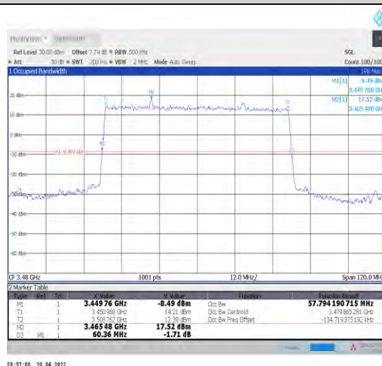
1-N78-3450-3550--30-60-L-2-DFT-PI2BPSK-Outer_ Full-162@0-Ant1-57.794-60.360-≤60-PASS
