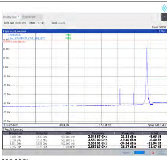
1-N78-3450-3550--30-30-H-2-DFT-PI2BPSK-Edge_1R B_Right-1@77-Ant1-PASS-see graph
