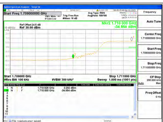
Band66 / 10MHz / Low CH / QPSK / FULL RB
