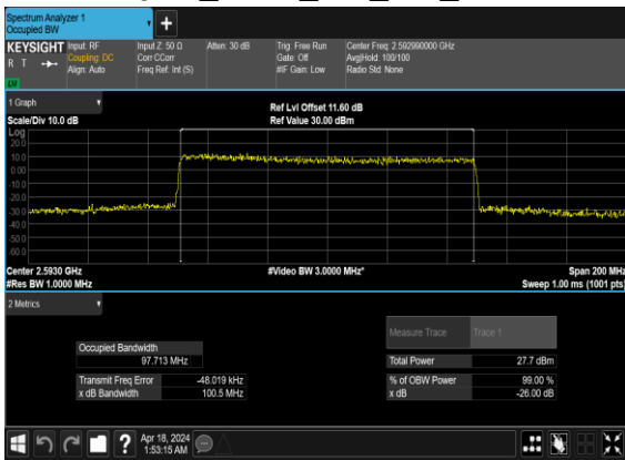
N41(100M)_CP-OFDM_64 QAM_Outer_Full_Mid_CH
