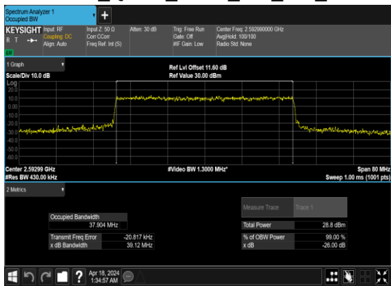
N41(40M)_CP- OFDM_QPSK_Outer_Full_Mid_CH
