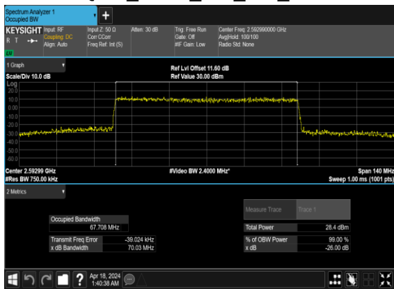
N41(70M)_CP-OFDM_16 QAM_Outer_Full_Mid_CH
