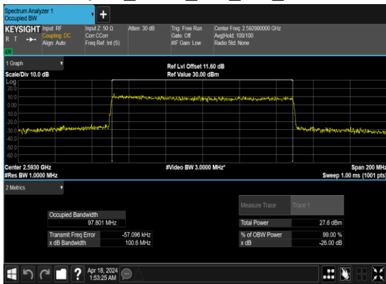
N41(100M)_CP-OFDM_256 QAM_Outer_Full_Mid_CH
