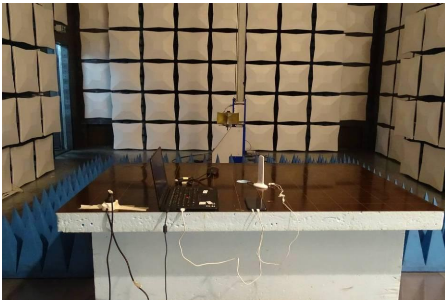
Radiated Disturbance Emissions (1GHz to 18GHz)
