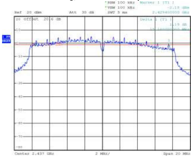
Figure 6-5: 6 dB Bandwidth
