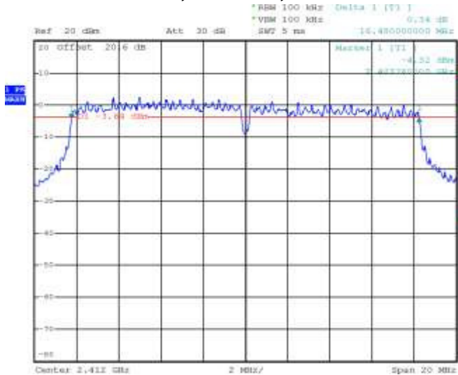
Figure 6-7: 6 dB Bandwidth
