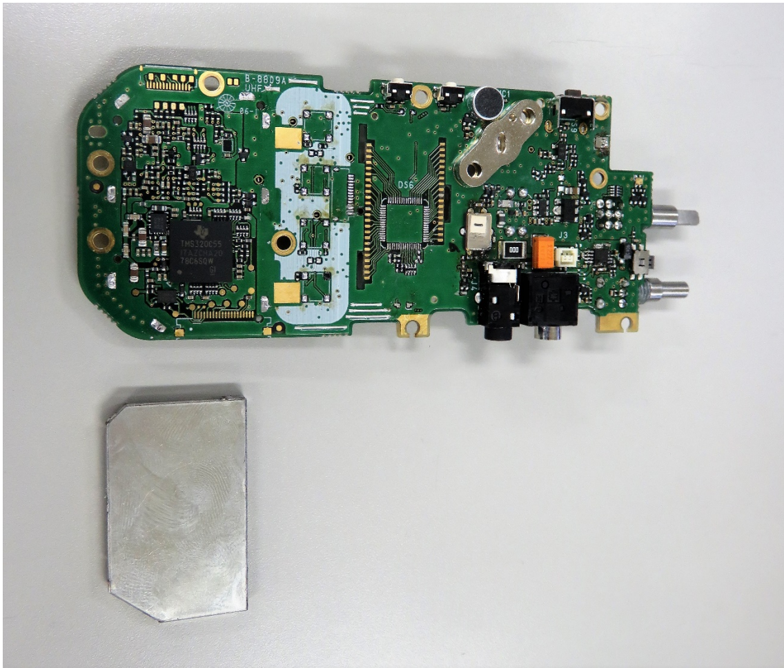
MAIN Board side-B view(IC-F2100D)
