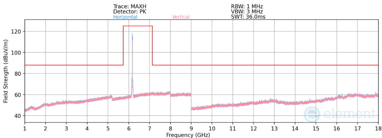
Plot 7-1227. Radiated Spurious Emissions above 1GHz Antenna WF8 (802.11ax – Ch. 45)
