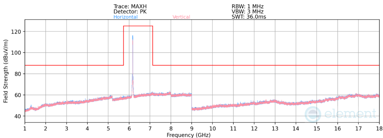
Plot 7-1252. Radiated Spurious Emissions SDM Primary (802.11ax – Ch. 45)
