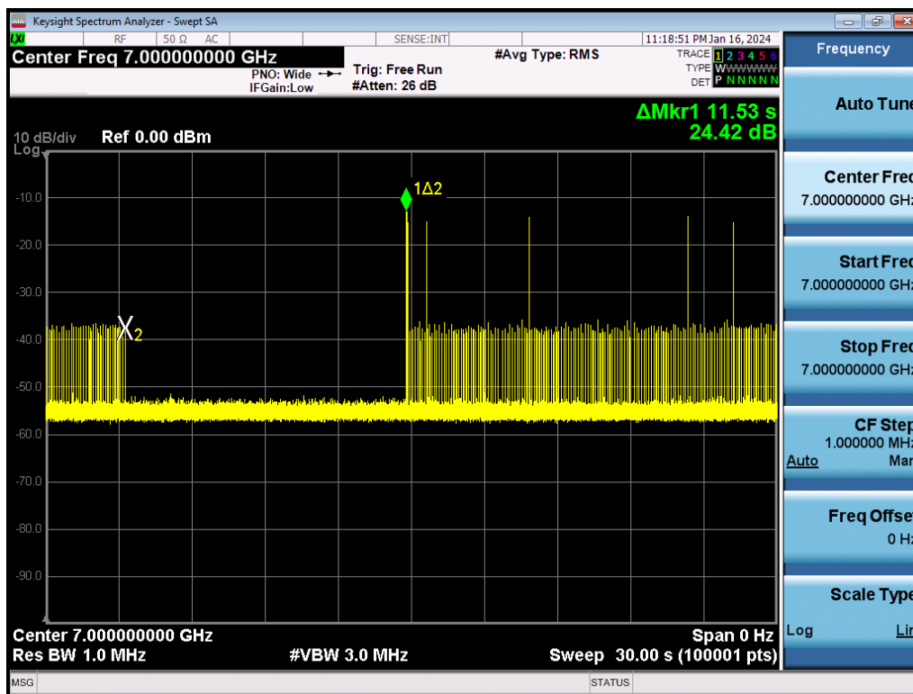
Plot 7-1208. Contention Based Protocol Timing Plot – UNII 8 – 160MHz Channel 207 – Mid
