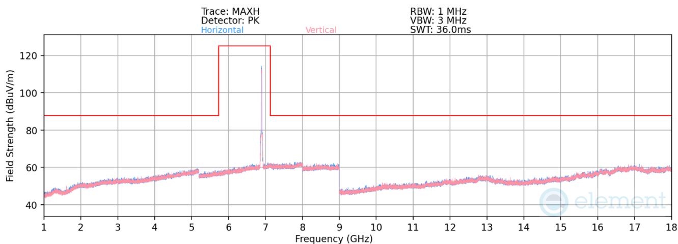
Plot 7-1235. Radiated Spurious Emissions above 1GHz Antenna WF8 (802.11ax – Ch. 189)
