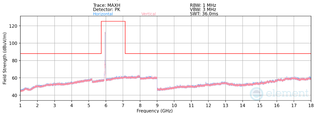
Plot 7-1238. Radiated Spurious Emissions above 1GHz Antenna WF7 (802.11ax – Ch. 1)
