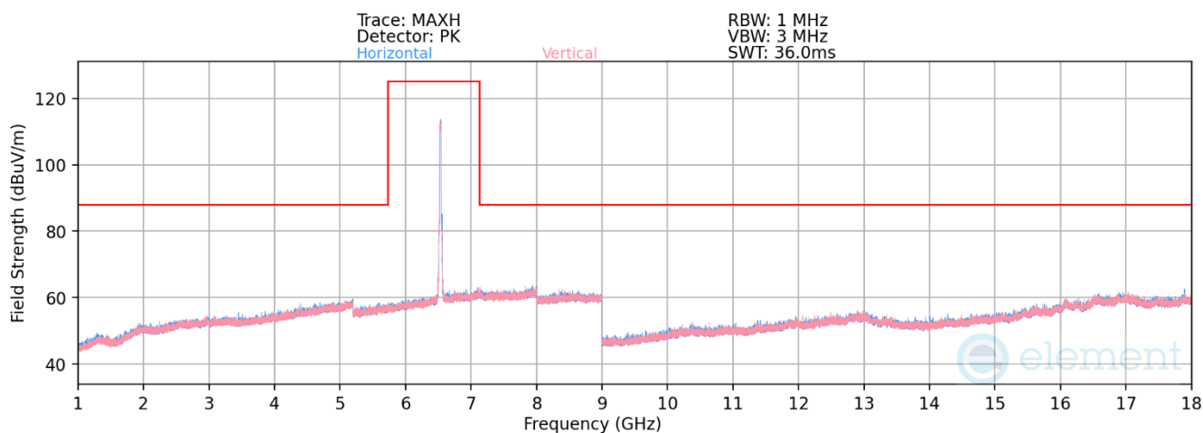
Plot 7-1244. Radiated Spurious Emissions above 1GHz Antenna WF7 (802.11ax – Ch. 117)
