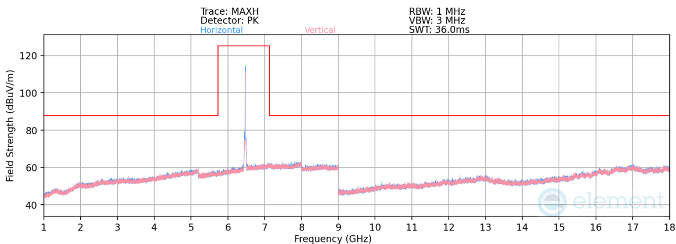
Plot 7-1230. Radiated Spurious Emissions above 1GHz Antenna WF8 (802.11ax – Ch. 105)
