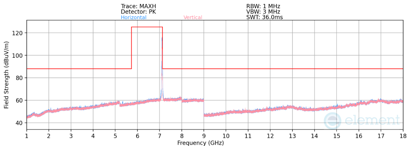
Plot 7-1225. Radiated Spurious Emissions above 1GHz Antenna WF5B (802.11ax – Ch. 233)
