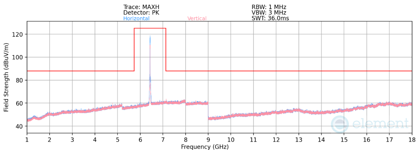
Plot 7-1254. Radiated Spurious Emissions SDM Primary (802.11ax – Ch.97)
