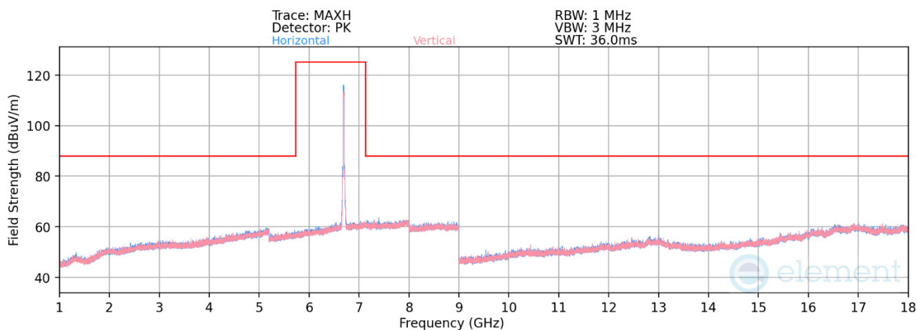
Plot 7-1245. Radiated Spurious Emissions above 1GHz Antenna WF7 (802.11ax – Ch. 149)
