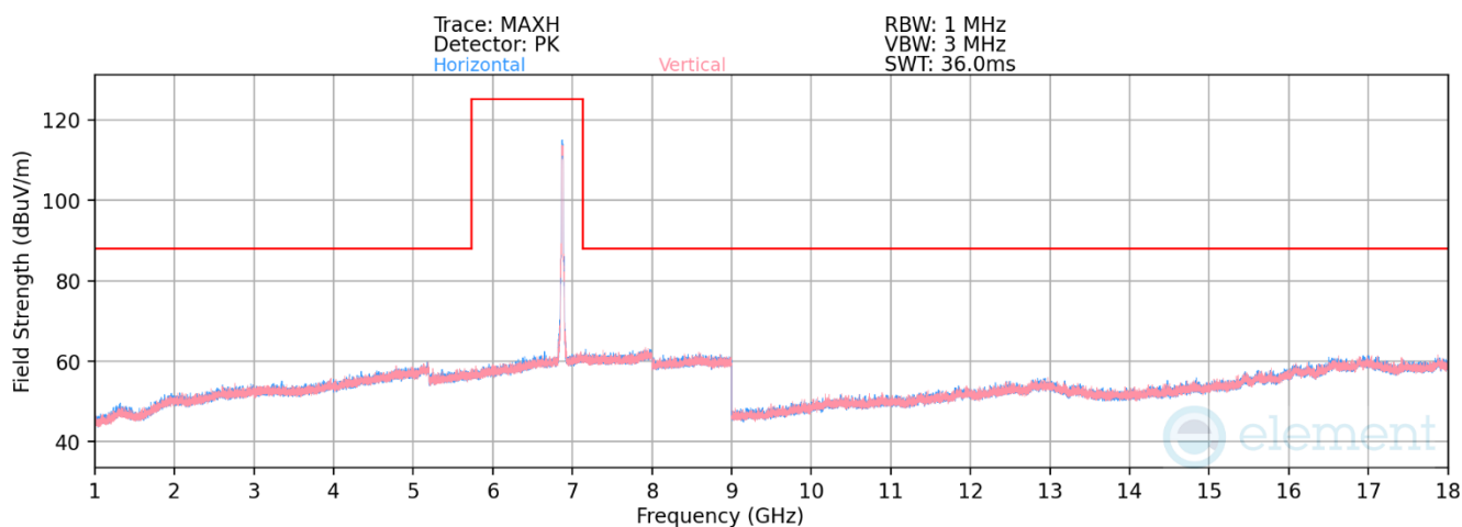
Plot 7-1246. Radiated Spurious Emissions above 1GHz Antenna WF7 (802.11ax – Ch. 185)
