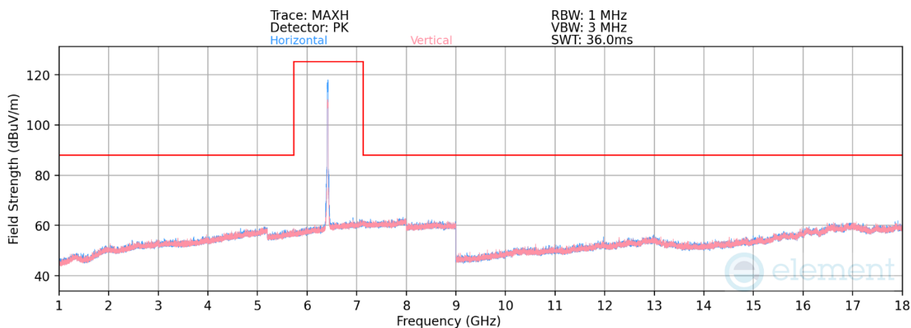
Plot 7-1253. Radiated Spurious Emissions SDM Primary (802.11ax – Ch. 93)
