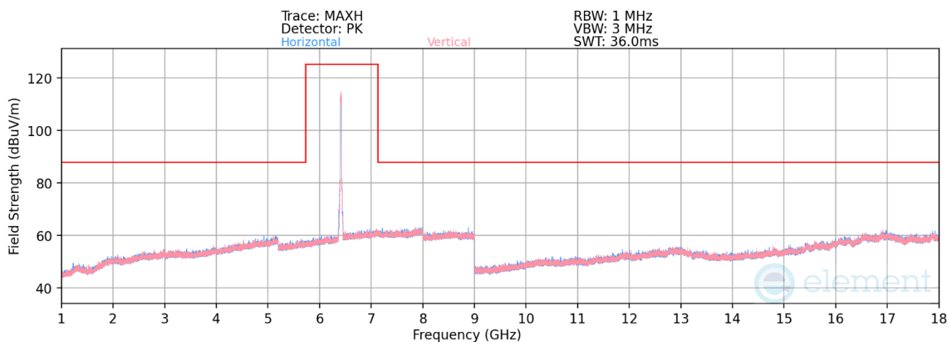
Plot 7-1240. Radiated Spurious Emissions above 1GHz Antenna WF7 (802.11ax – Ch. 93)
