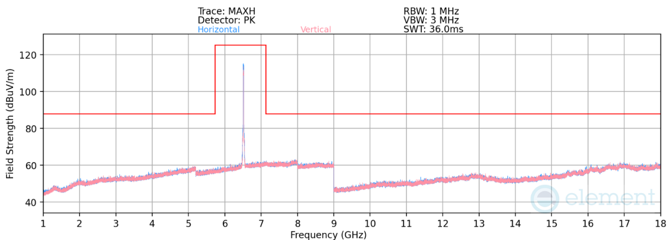
Plot 7-1231. Radiated Spurious Emissions above 1GHz Antenna WF8 (802.11ax – Ch. 113)
