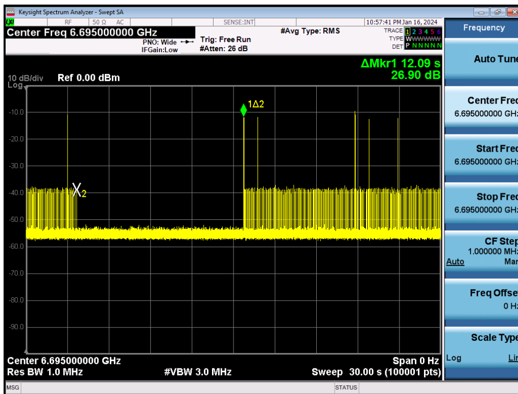
Plot 7-1202. Contention Based Protocol Timing Plot – UNII 7 – 20MHz Channel 149
