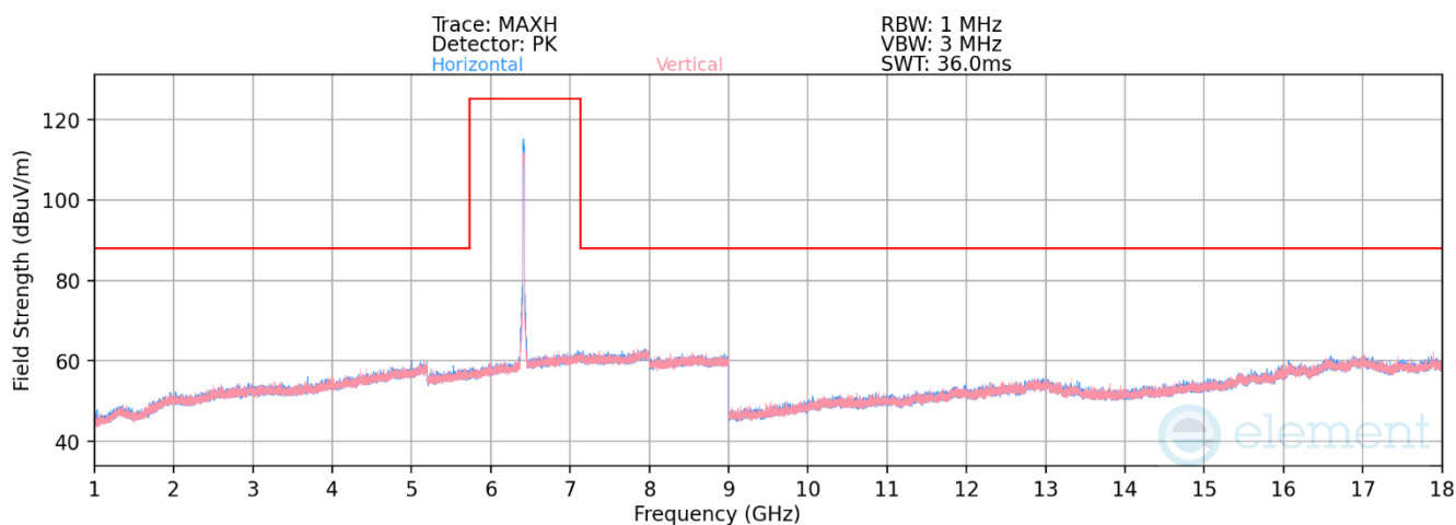
Plot 7-1228. Radiated Spurious Emissions above 1GHz Antenna WF8 (802.11ax – Ch. 93)
