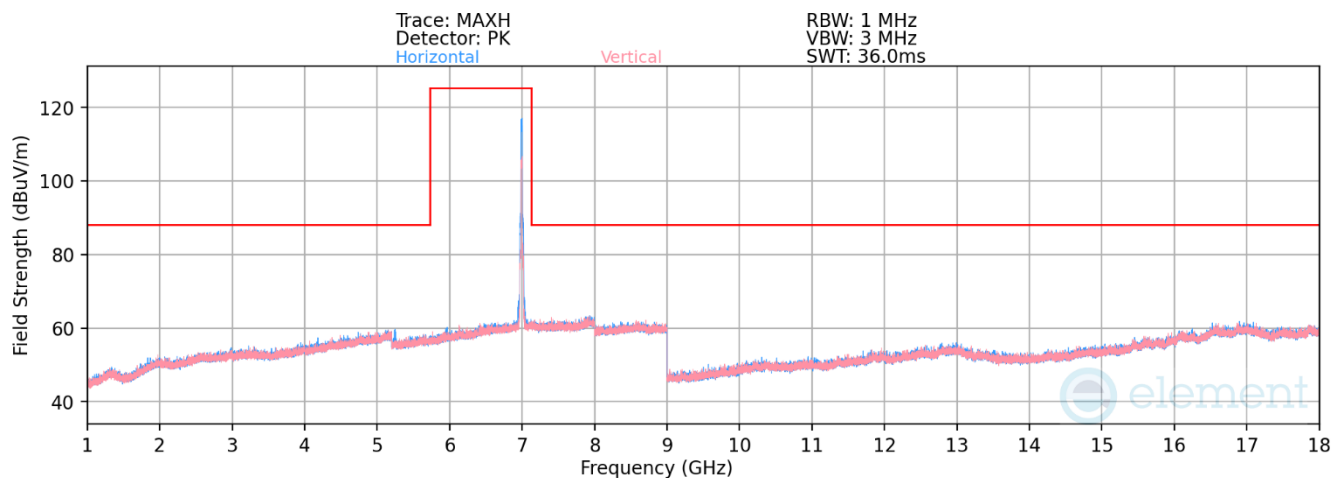
Plot 7-1224. Radiated Spurious Emissions above 1GHz Antenna WF5B (802.11ax – Ch. 209)
