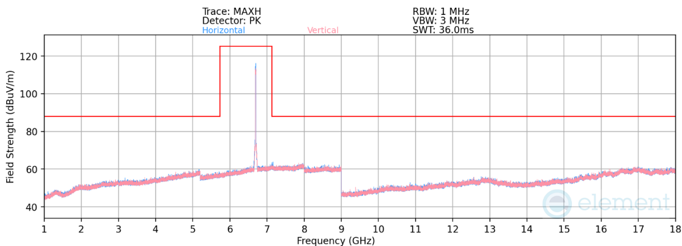
Plot 7-1233. Radiated Spurious Emissions above 1GHz Antenna WF8 (802.11ax – Ch. 149)
