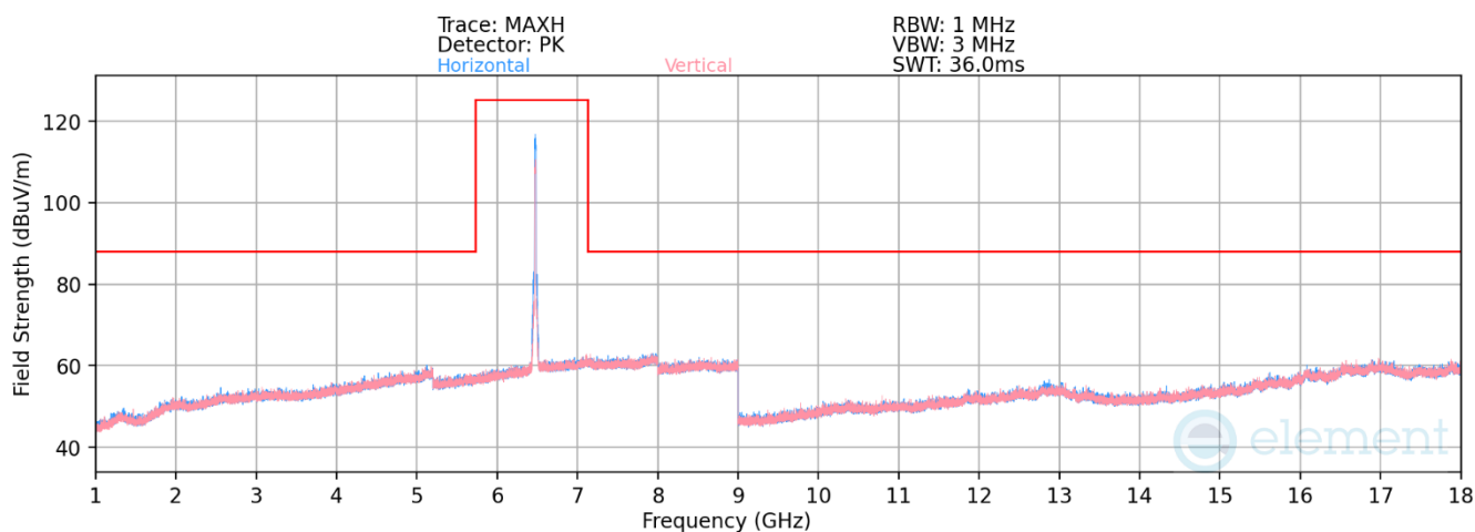
Plot 7-1255. Radiated Spurious Emissions SDM Primary (802.11ax – Ch. 105)
