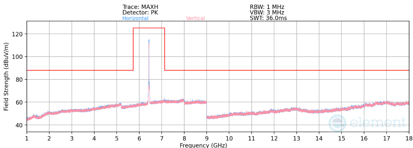
Plot 7-1229. Radiated Spurious Emissions above 1GHz Antenna WF8 (802.11ax – Ch. 97)
