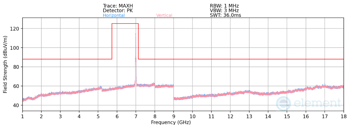
Plot 7-1248. Radiated Spurious Emissions above 1GHz Antenna WF7 (802.11ax – Ch. 209)
