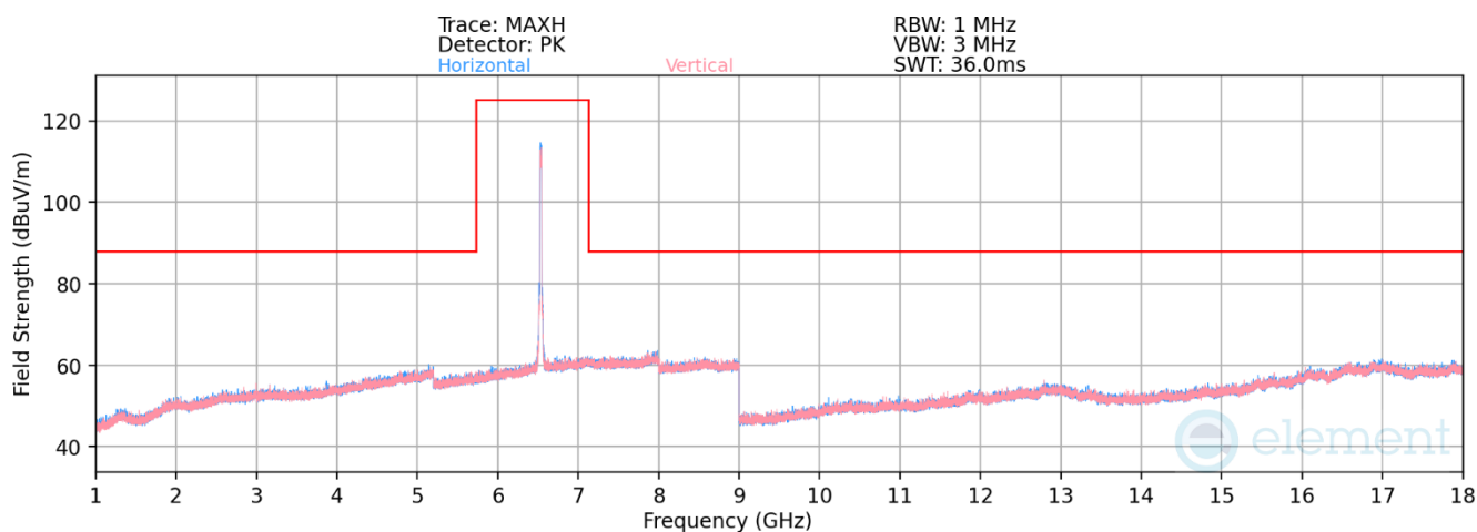
Plot 7-1232. Radiated Spurious Emissions above 1GHz Antenna WF8 (802.11ax – Ch. 117)
